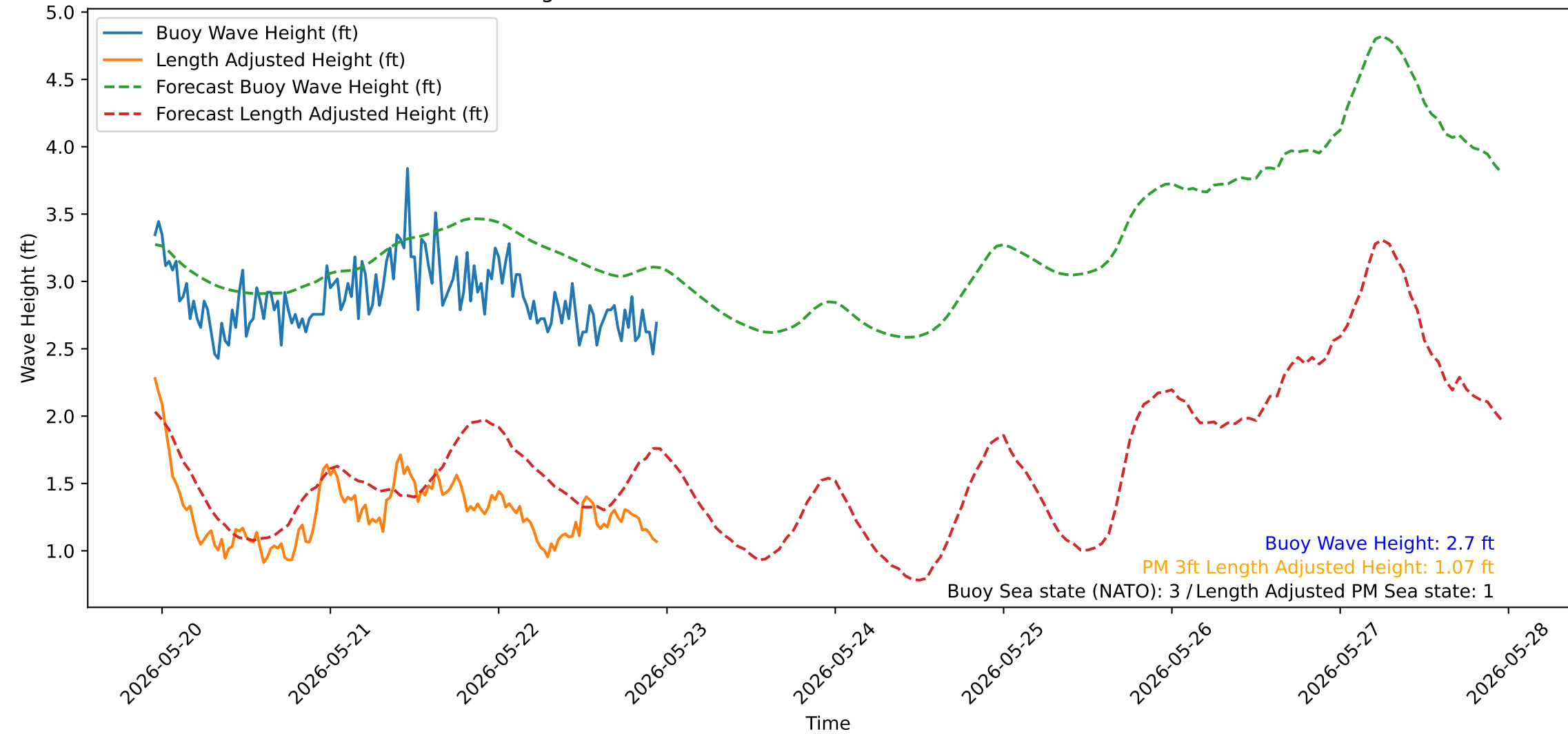
Wave Heights over Time for Oceanside Harbor at 2026-05-22 23:10:32
