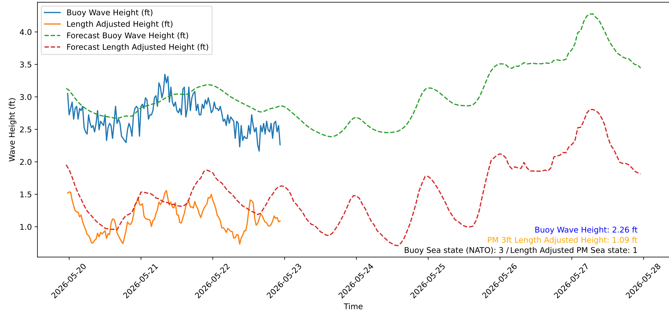
Wave Heights over Time for Red Beach at 2026-05-22 23:10:51
