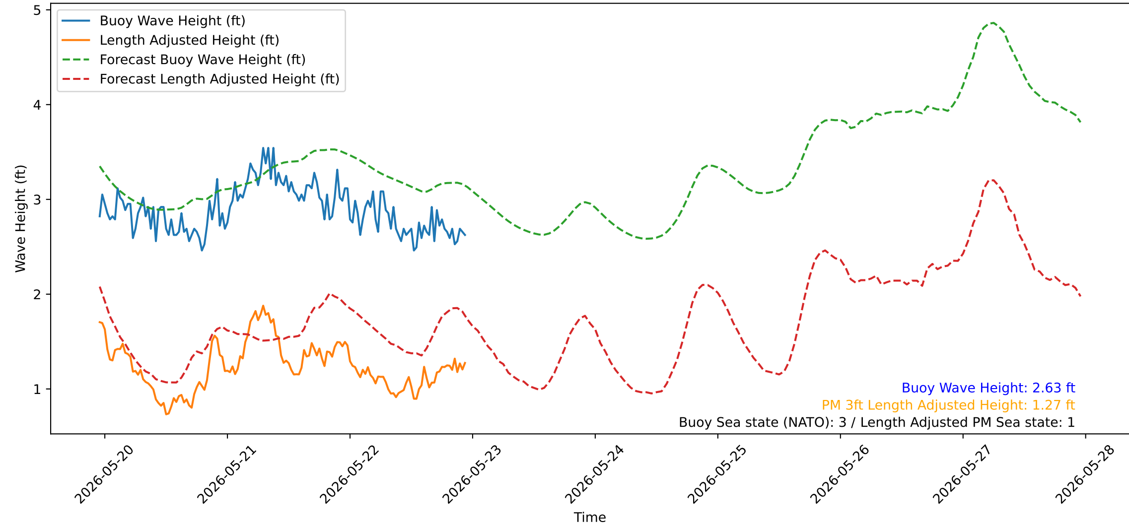
Wave Heights over Time for Green Beach at 2026-05-22 23:11:14
