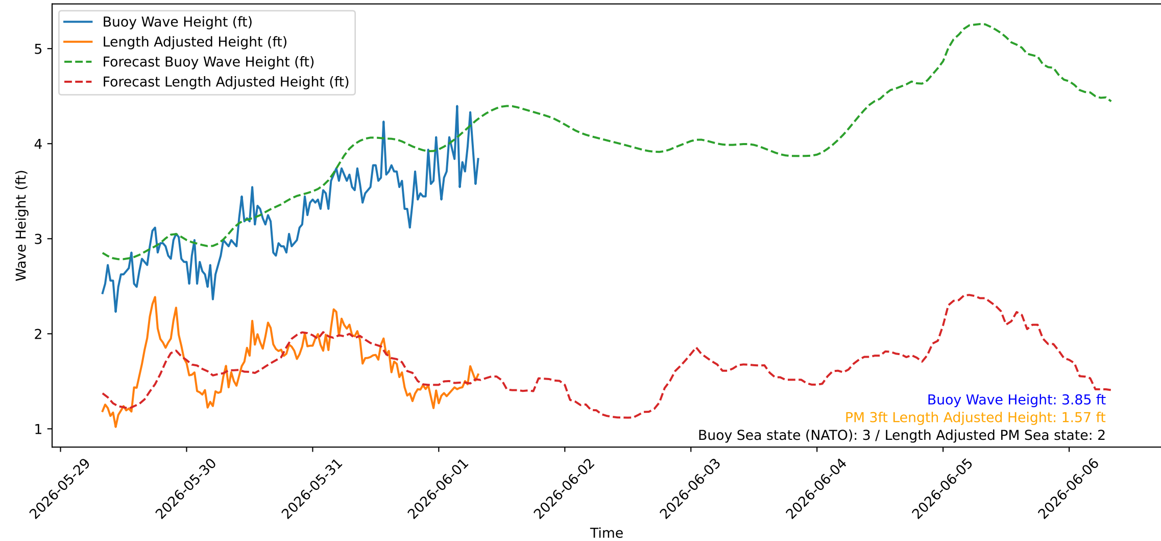
Wave Heights over Time for Oceanside Harbor at 2026-06-01 08:10:25
