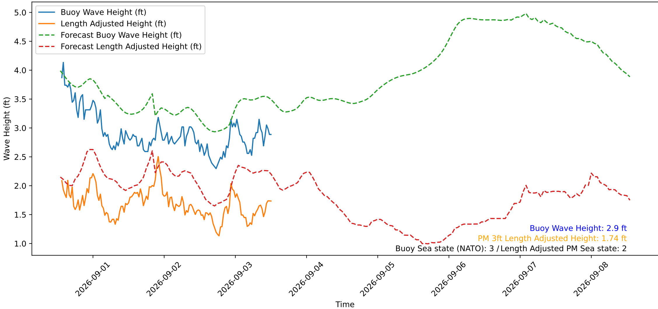
Wave Heights over Time for Red Beach at 2026-09-03 13:00:50
