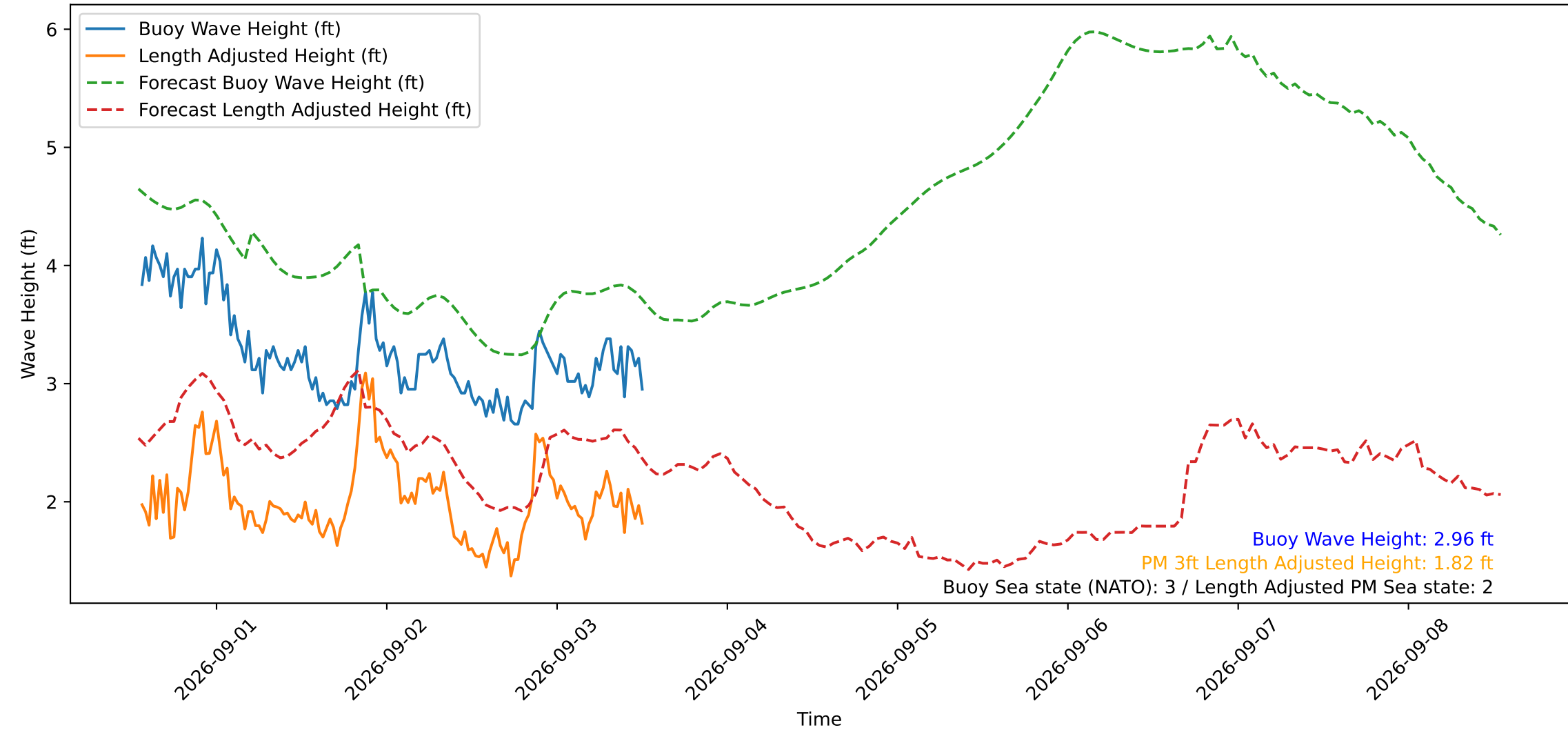
Wave Heights over Time for Green Beach at 2026-09-03 13:01:13
