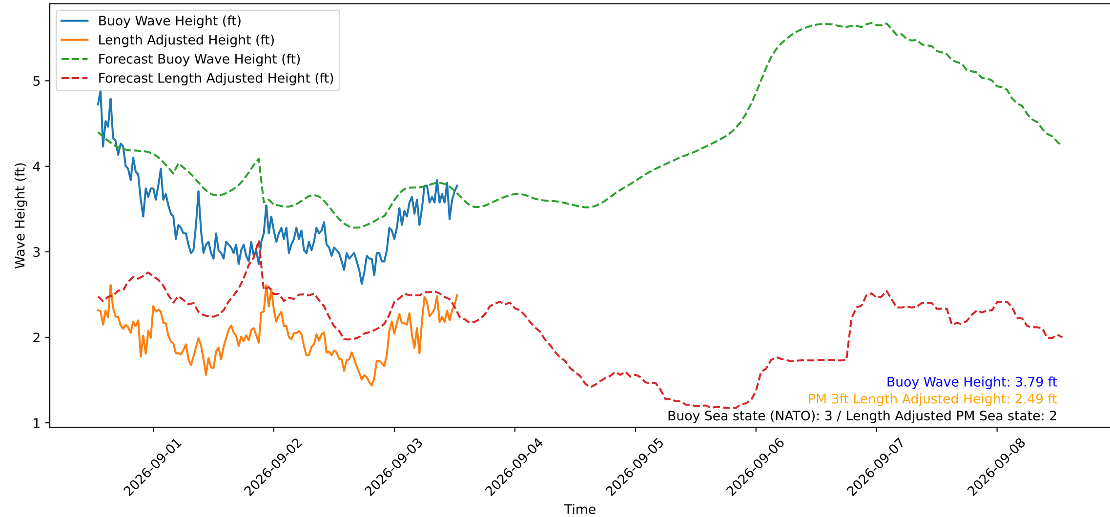
Wave Heights over Time for Oceanside Harbor at 2026-09-03 13:00:30
