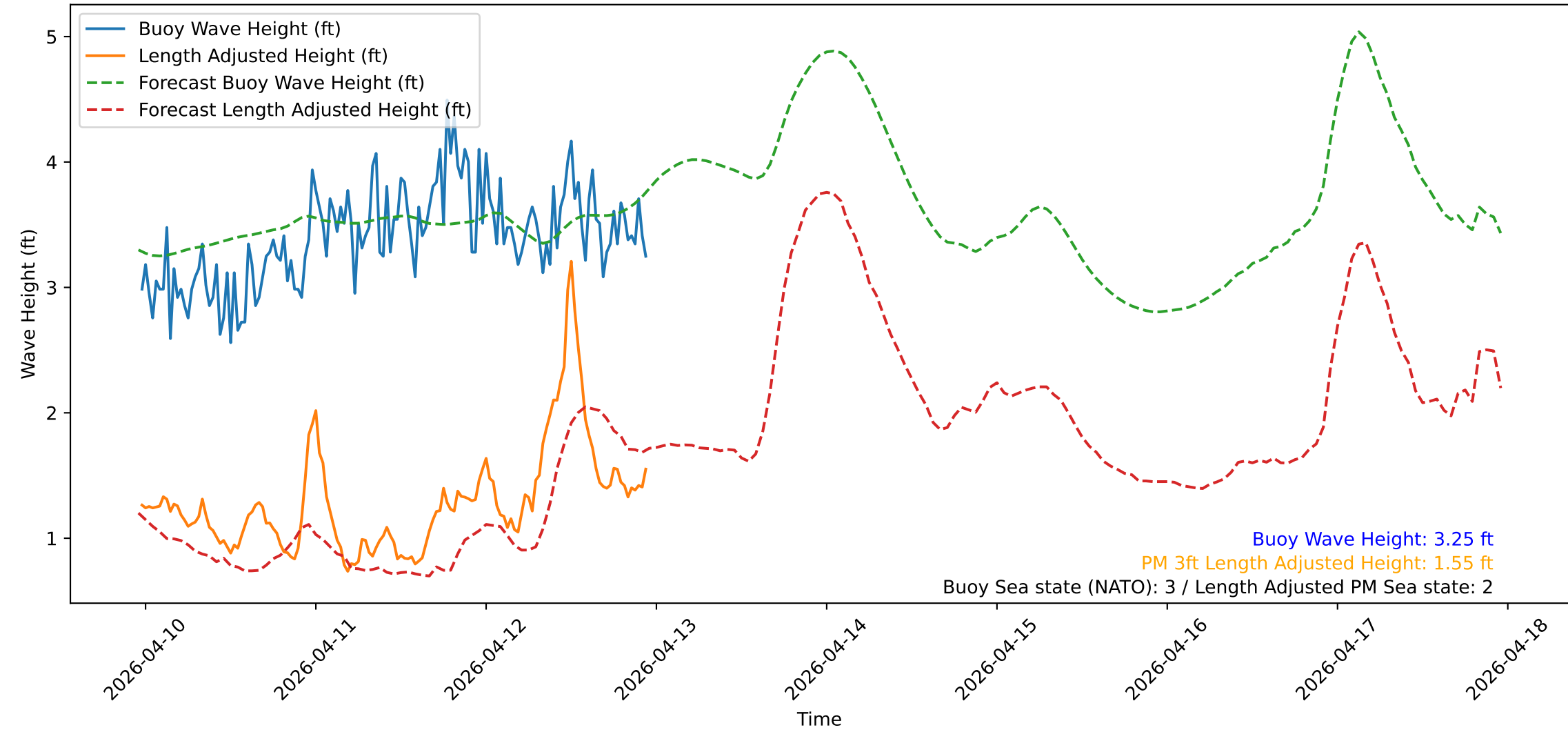
Wave Heights over Time for Green Beach at 2026-04-12 23:21:12
