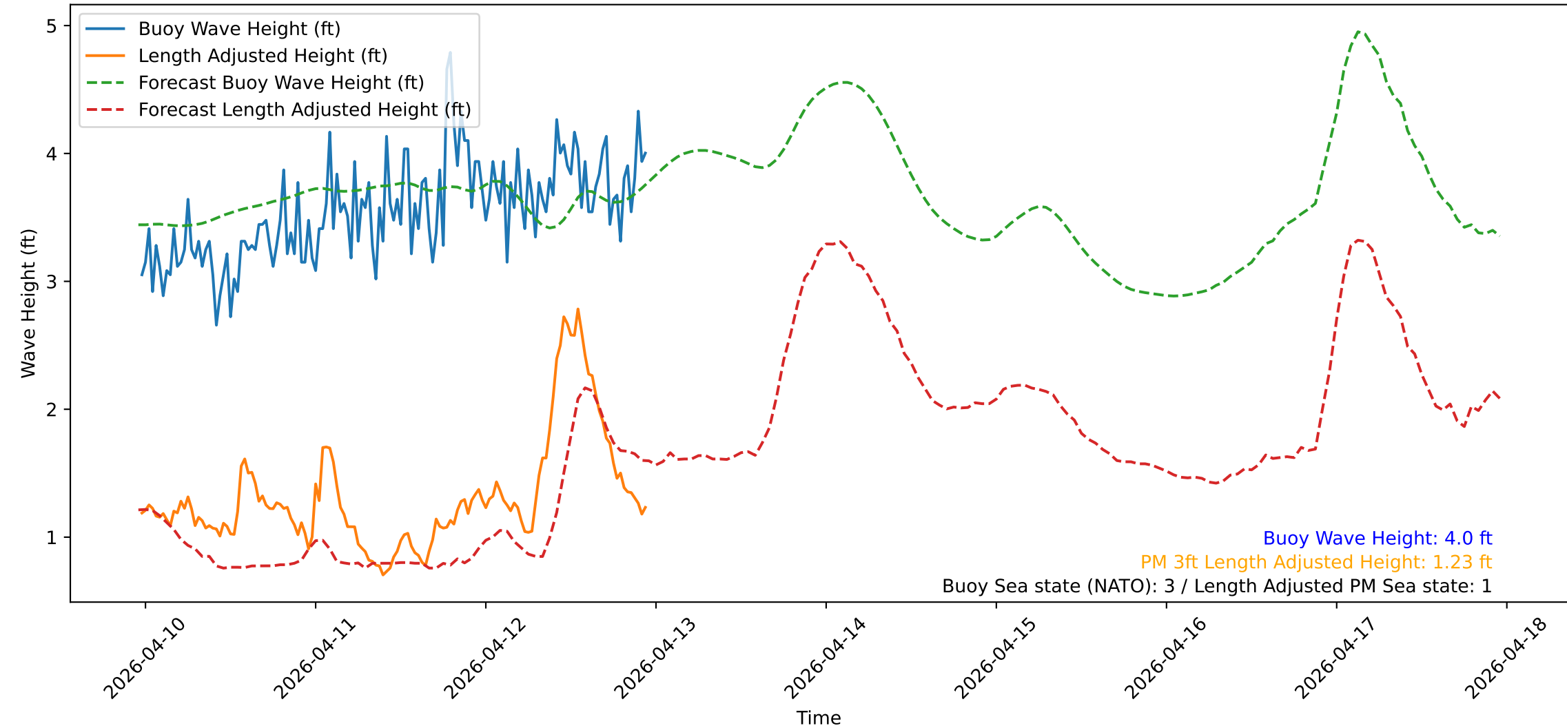
Wave Heights over Time for Oceanside Harbor at 2026-04-12 23:20:30
