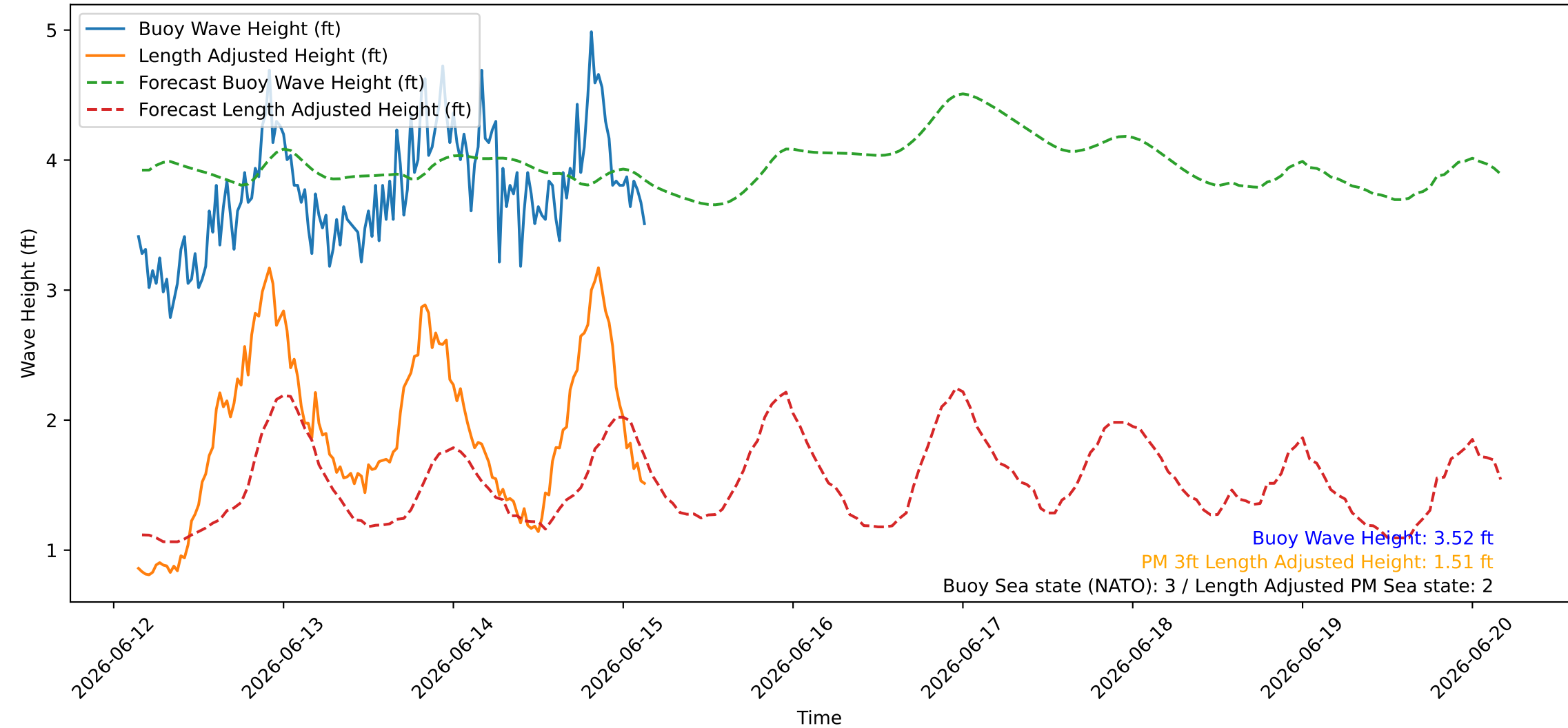
Wave Heights over Time for Oceanside Harbor at 2026-06-15 03:40:26
