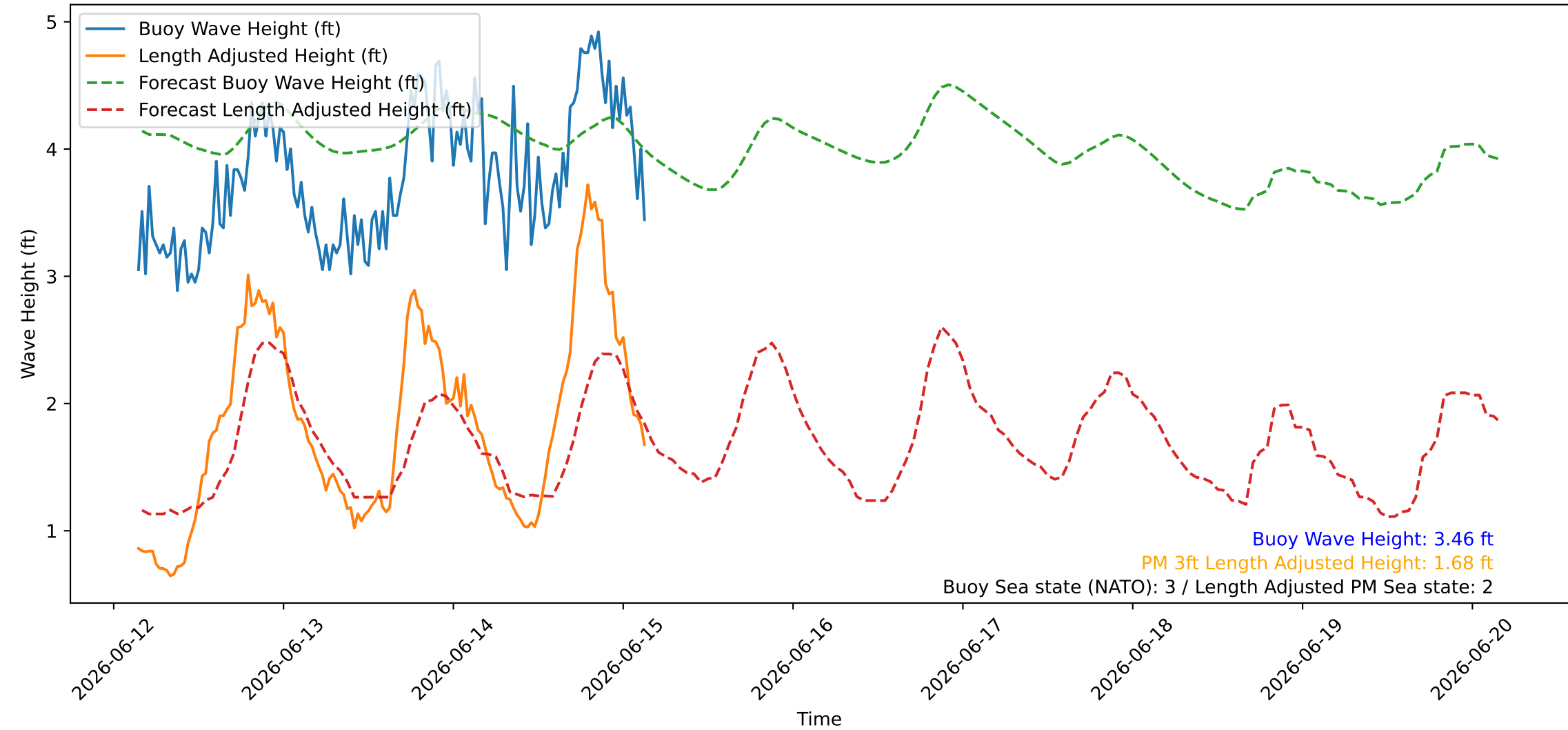
Wave Heights over Time for Green Beach at 2026-06-15 03:41:08
