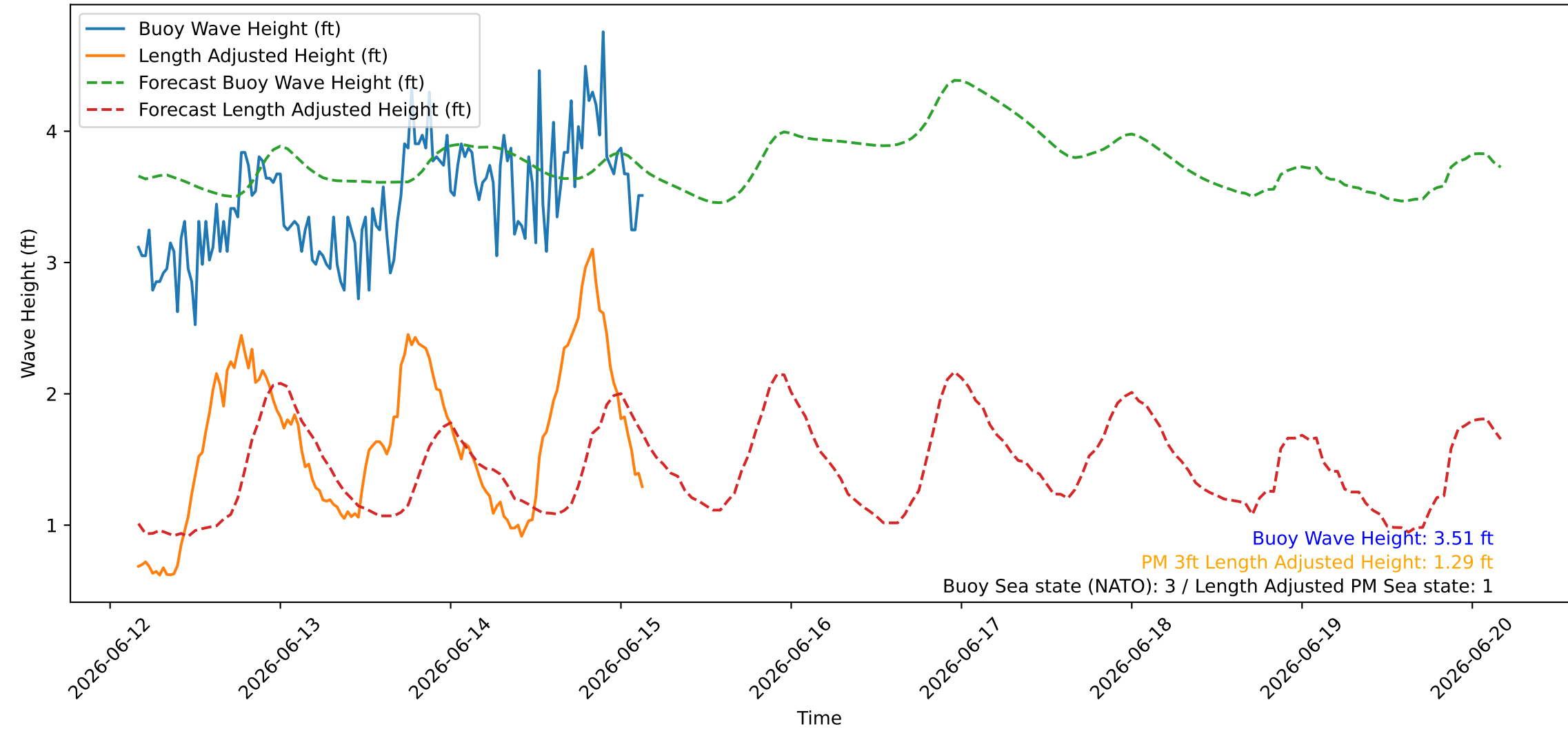
Wave Heights over Time for Red Beach at 2026-06-15 03:40:45
