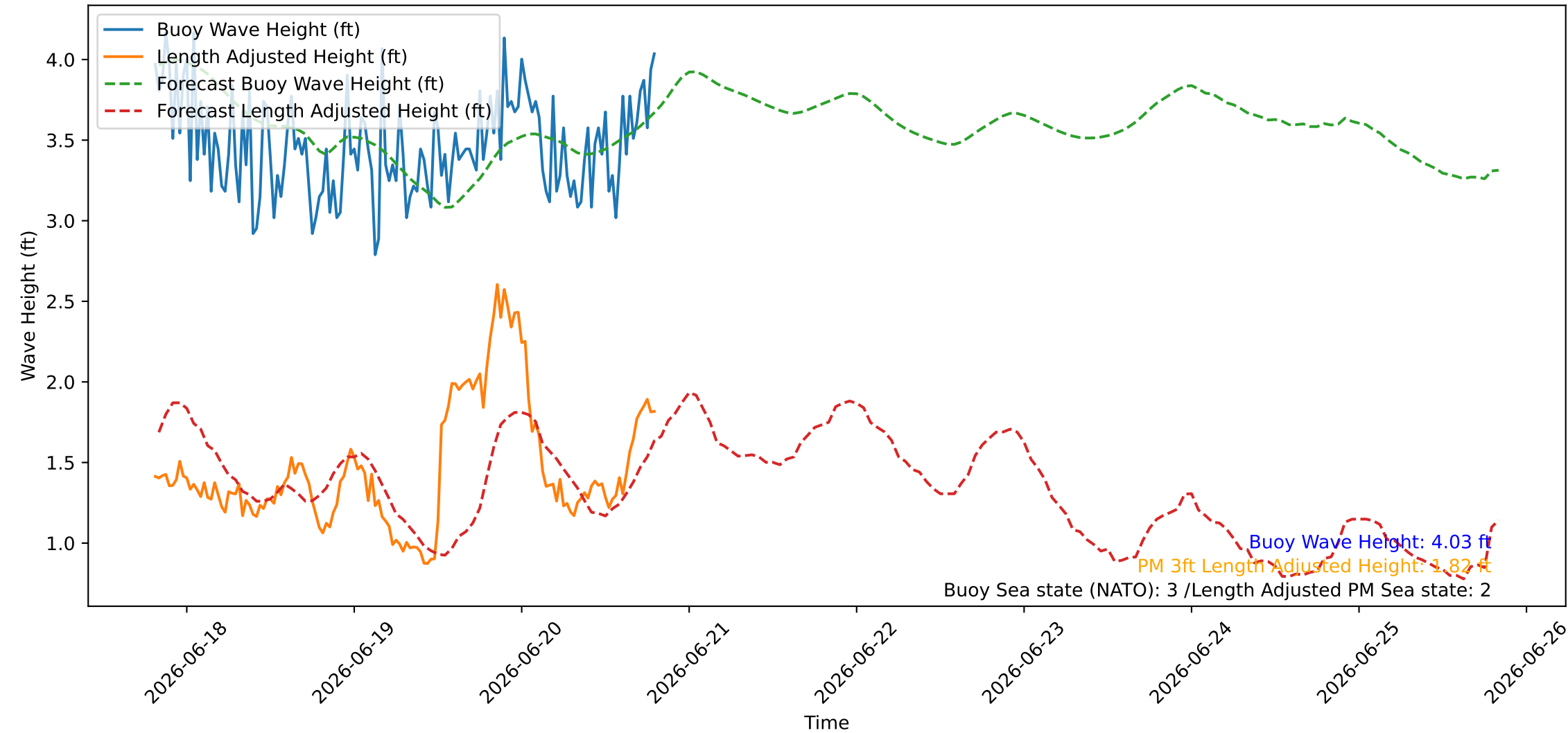
Wave Heights over Time for Oceanside Harbor at 2026-06-20 19:40:25
