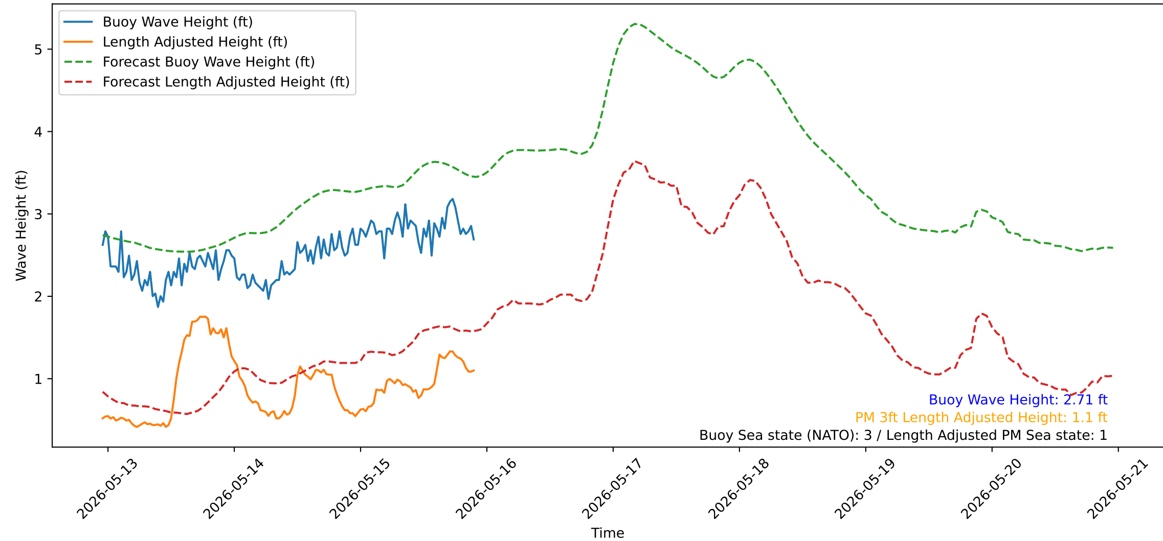
Wave Heights over Time for Red Beach at 2026-05-15 22:30:50
