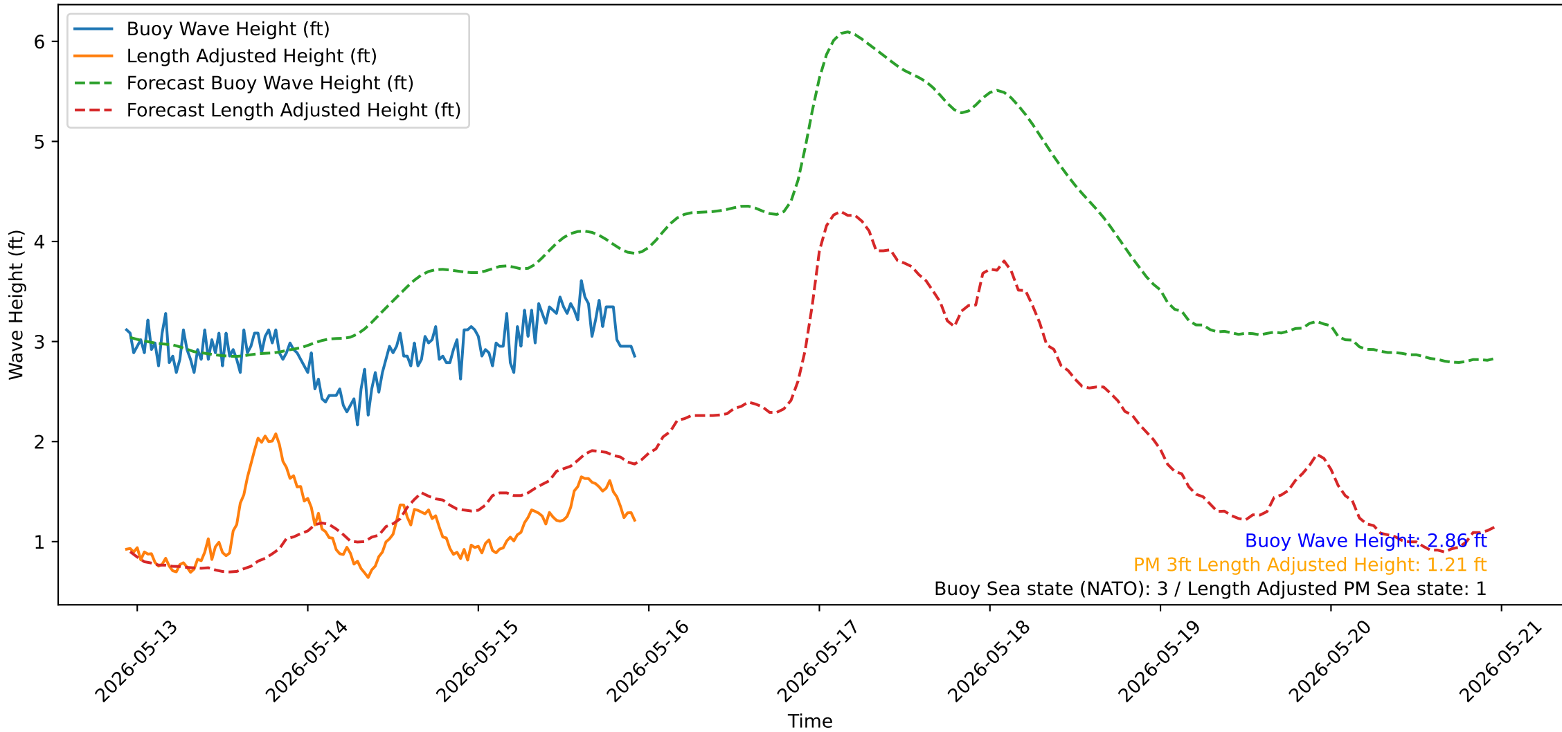
Wave Heights over Time for Oceanside Harbor at 2026-05-15 22:30:31
