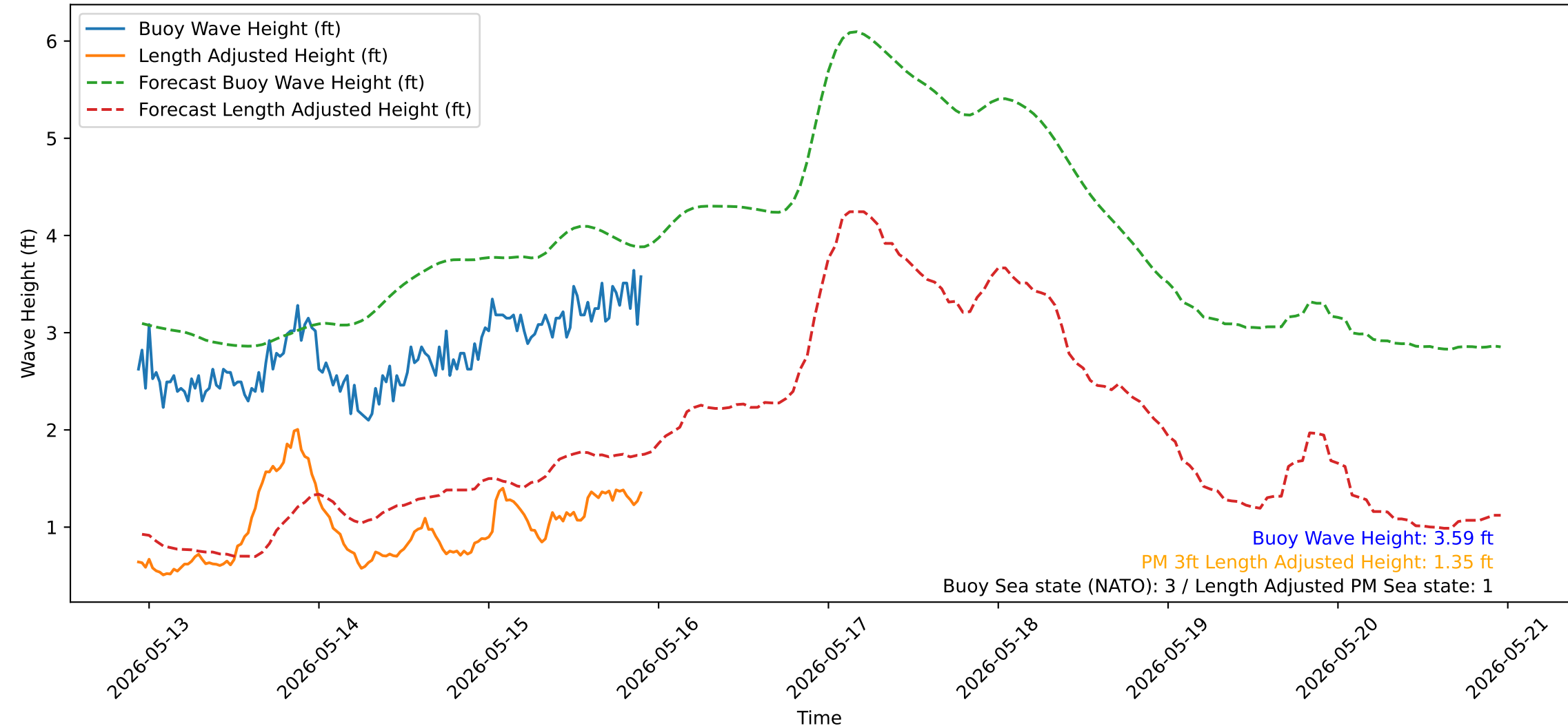
Wave Heights over Time for Green Beach at 2026-05-15 22:31:12
