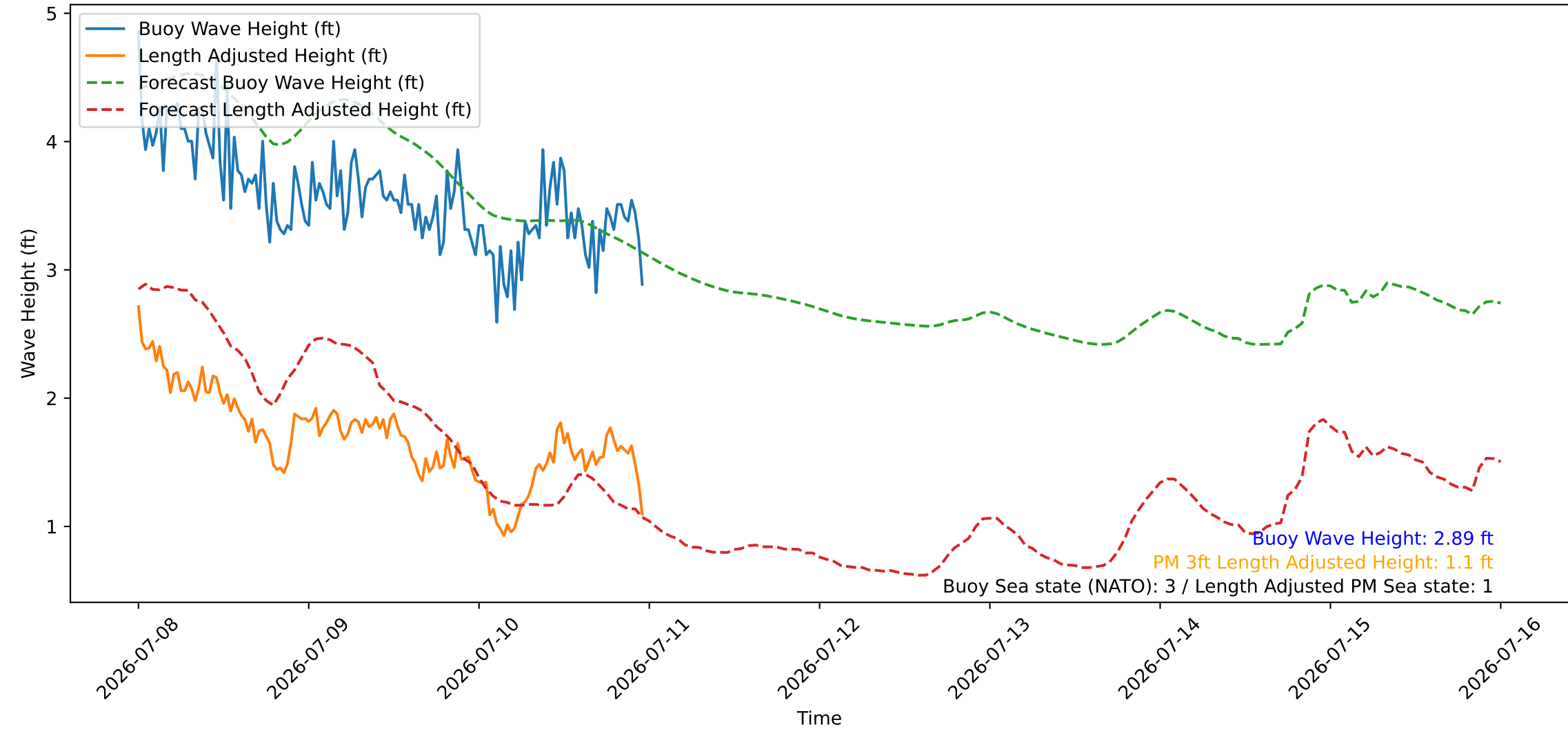
Wave Heights over Time for Red Beach at 2026-07-10 23:50:47
