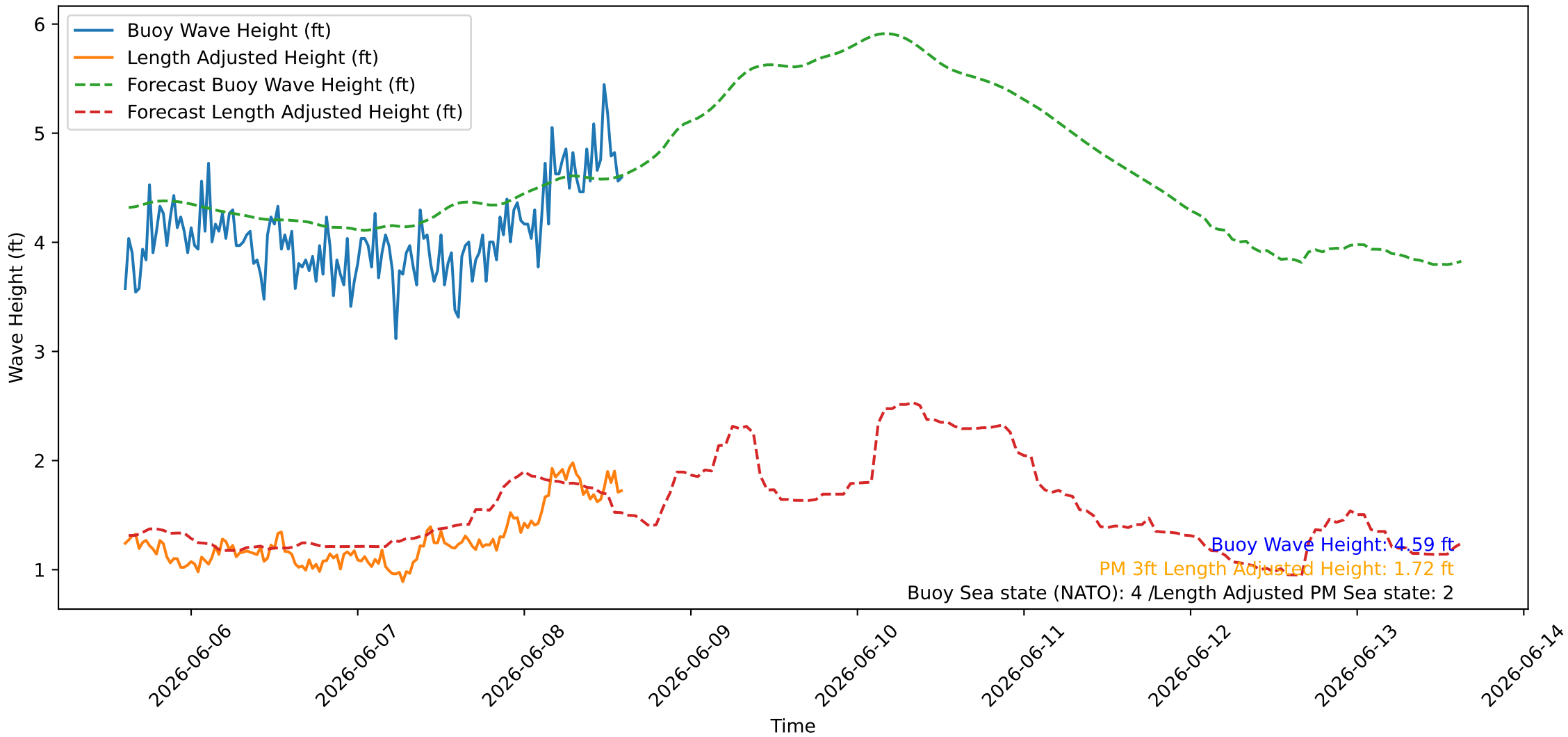
Wave Heights over Time for Green Beach at 2026-06-08 14:41:09
