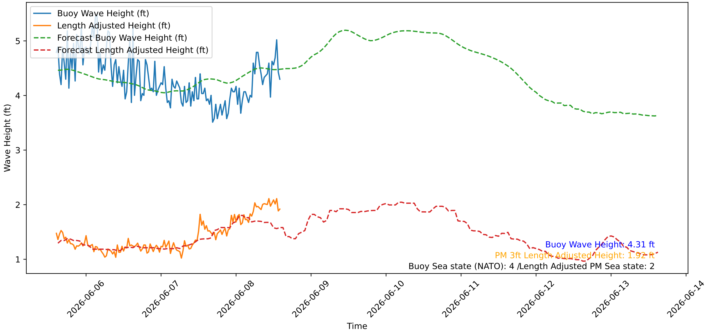
Wave Heights over Time for Oceanside Harbor at 2026-06-08 14:40:26
