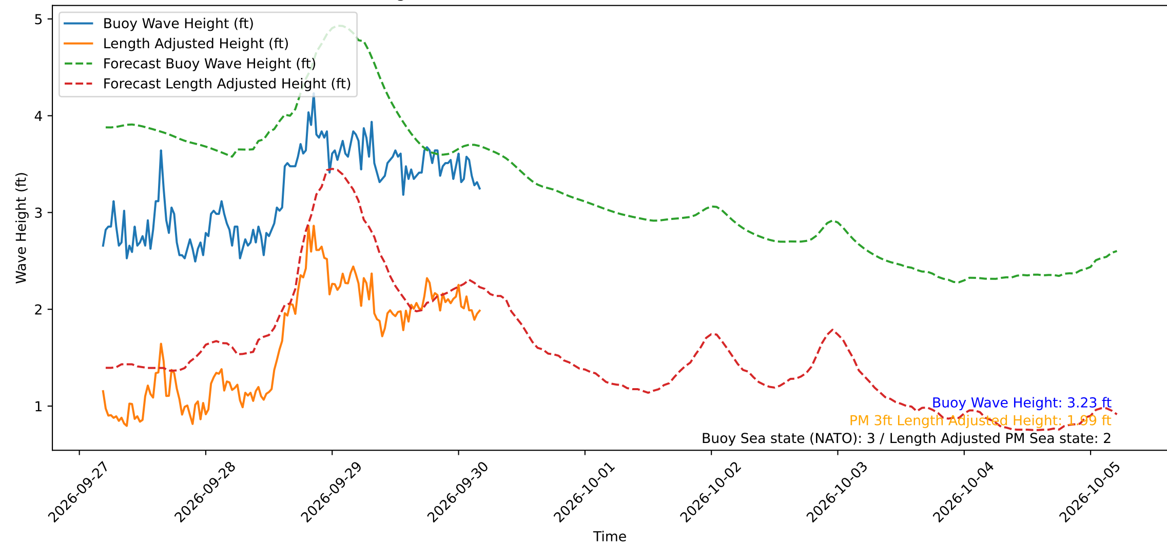
Wave Heights over Time for Oceanside Harbor at 2026-09-30 04:40:29
