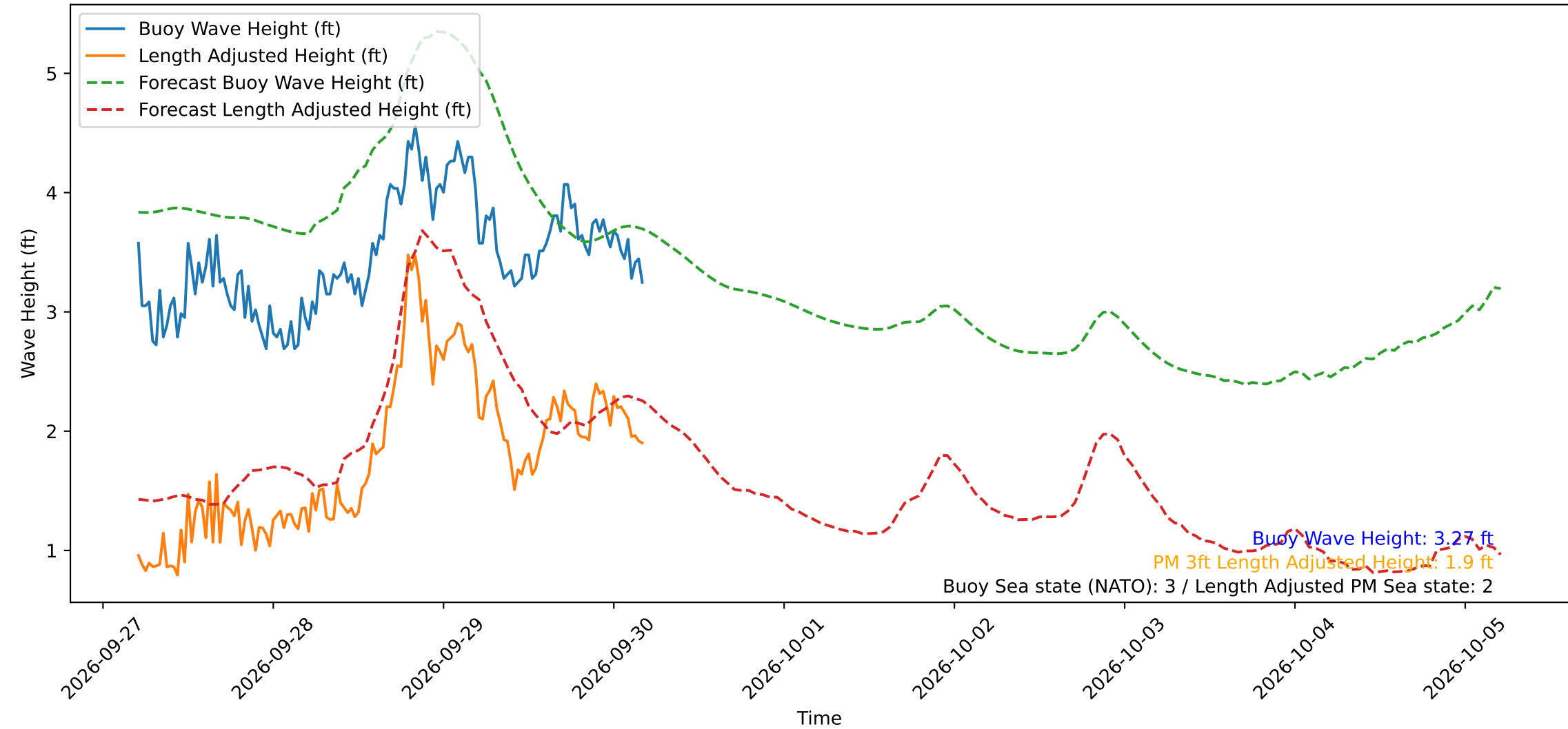
Wave Heights over Time for Green Beach at 2026-09-30 04:41:11
