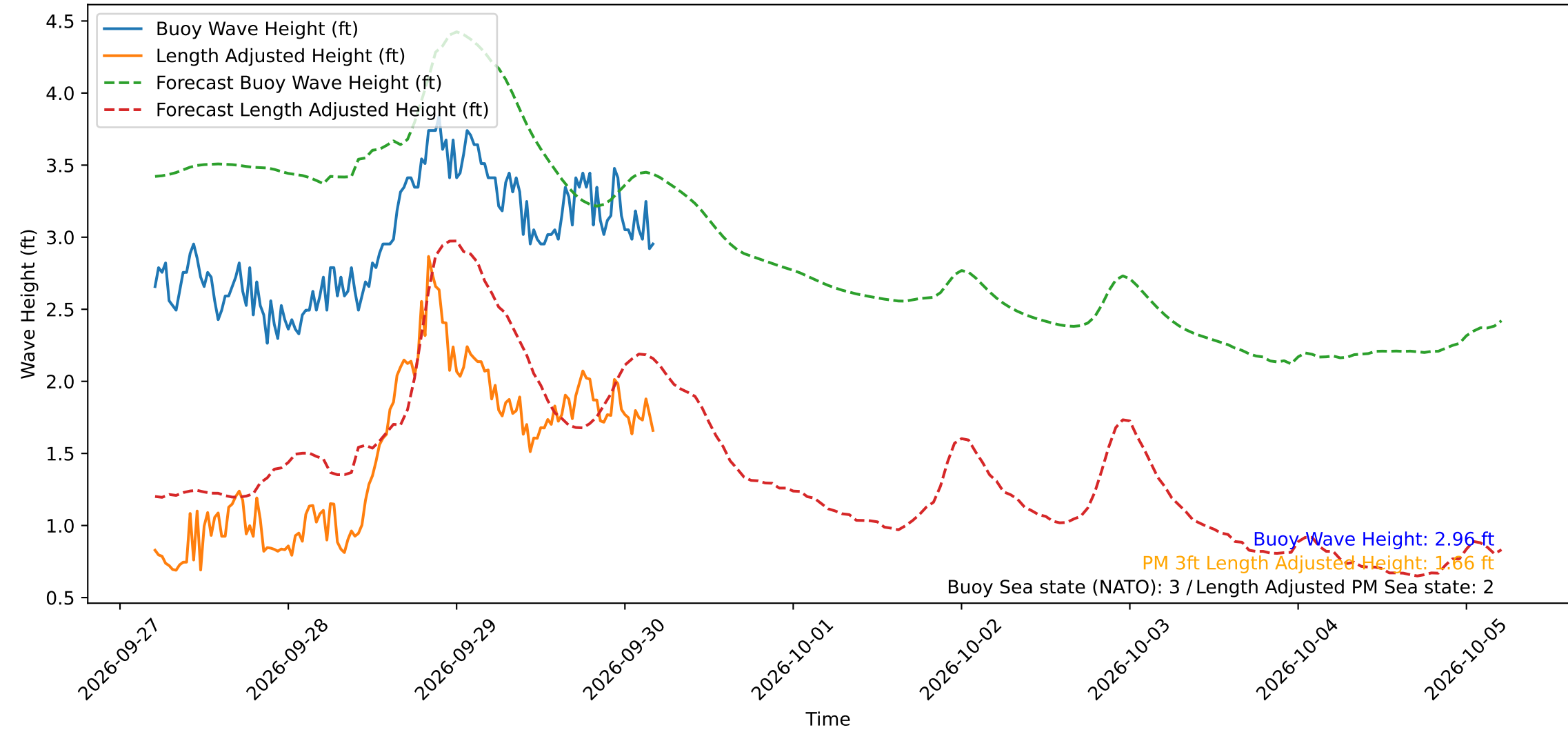
Wave Heights over Time for Red Beach at 2026-09-30 04:40:49
