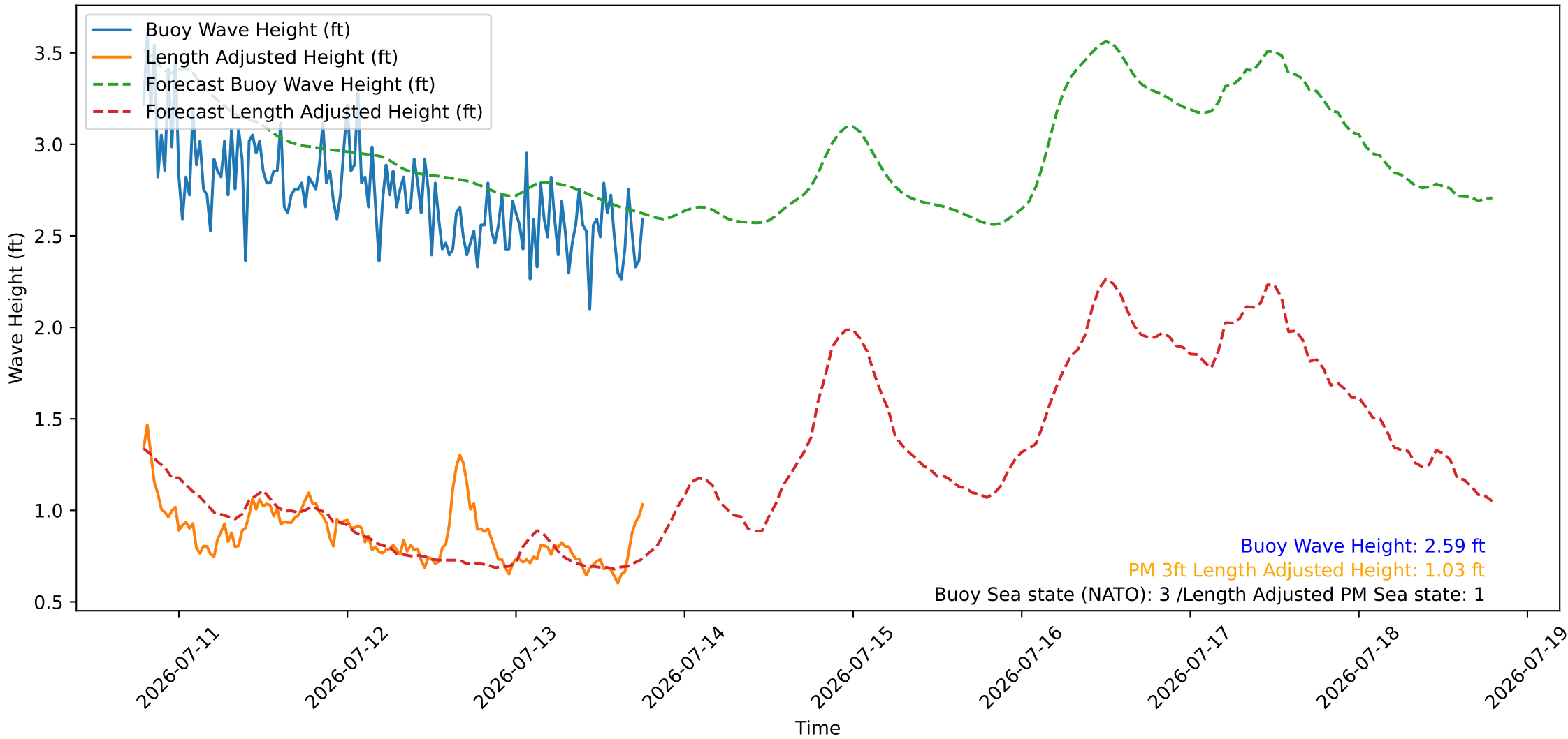
Wave Heights over Time for Oceanside Harbor at 2026-07-13 18:50:26
