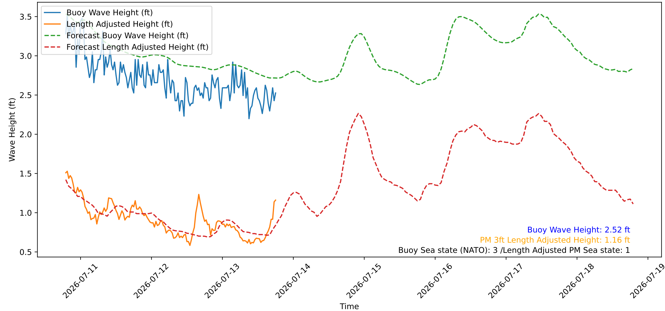
Wave Heights over Time for Green Beach at 2026-07-13 18:51:09
