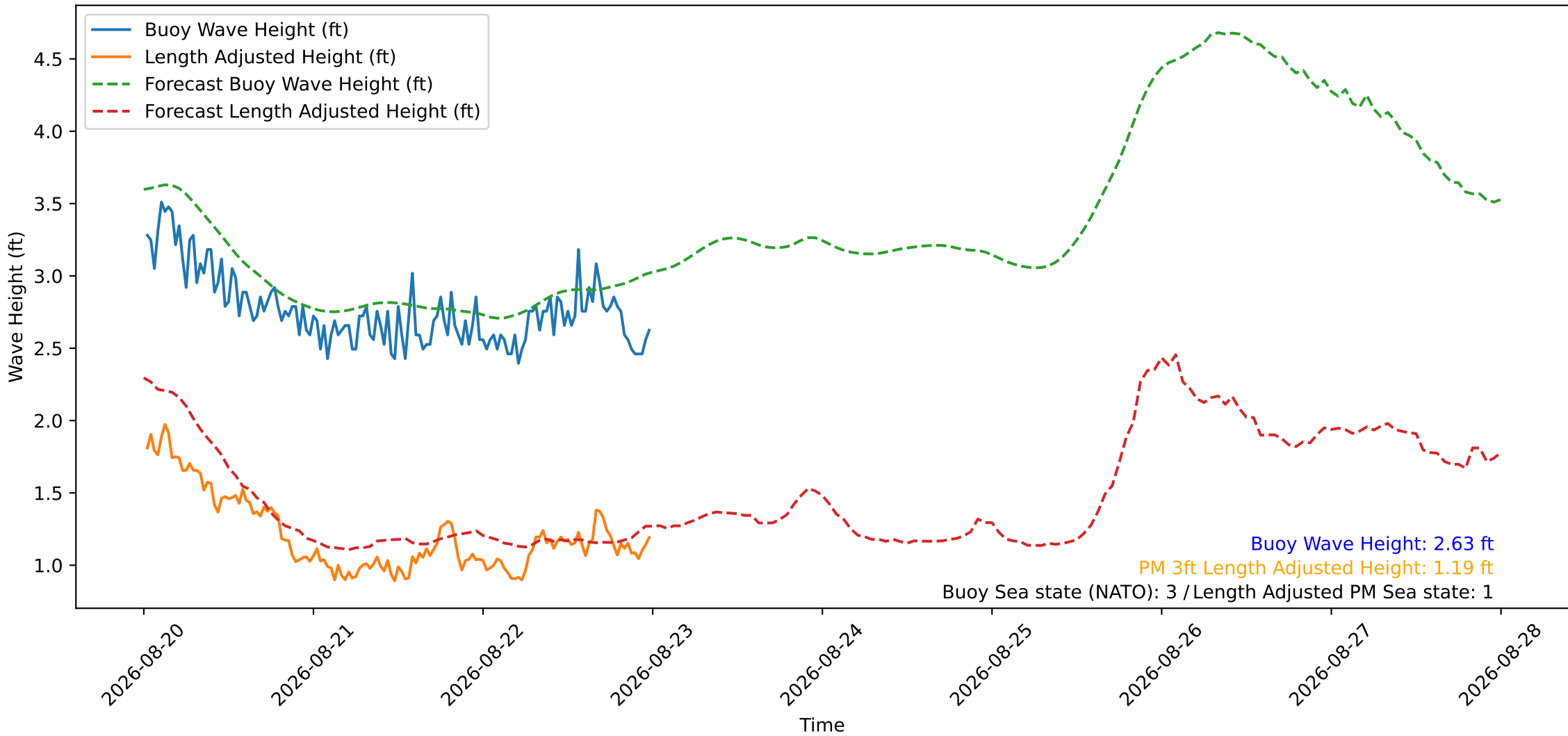
Wave Heights over Time for Green Beach at 2026-08-23 00:21:14
