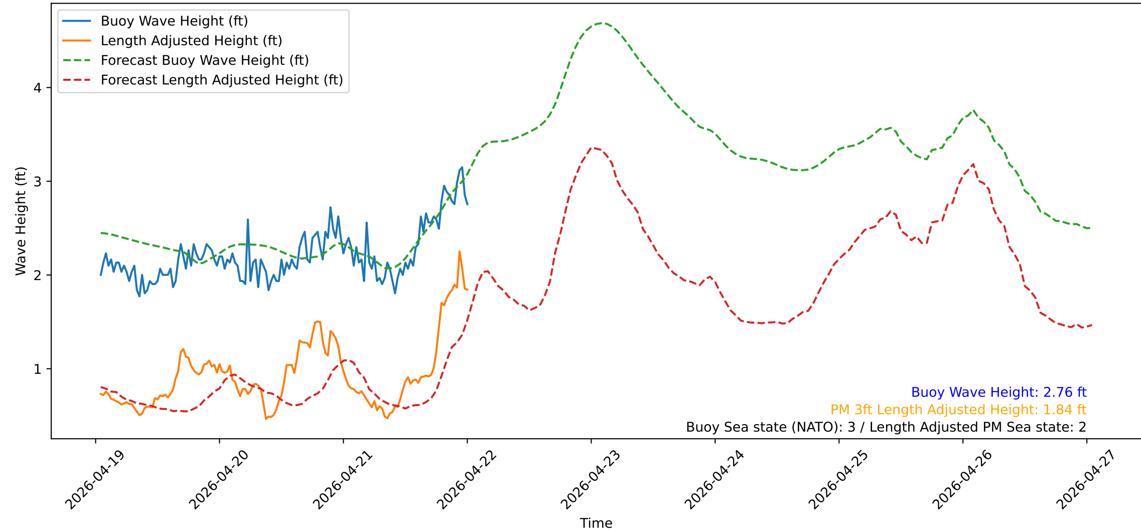
Wave Heights over Time for Red Beach at 2026-04-22 00:40:50
