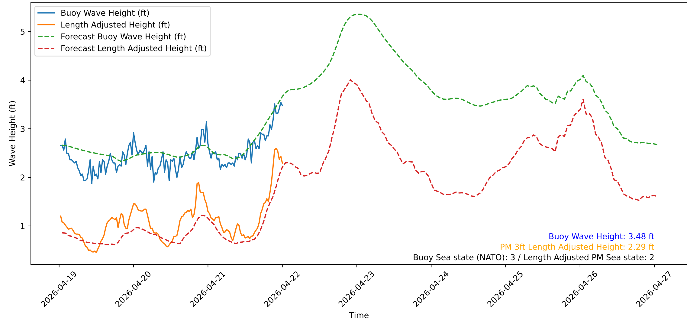
Wave Heights over Time for Green Beach at 2026-04-22 00:41:12
