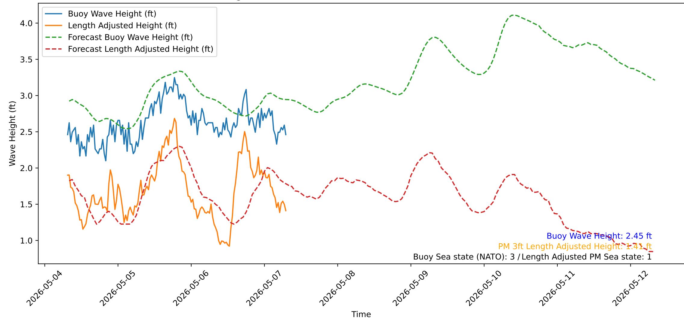
Wave Heights over Time for Oceanside Harbor at 2026-05-07 07:30:31
