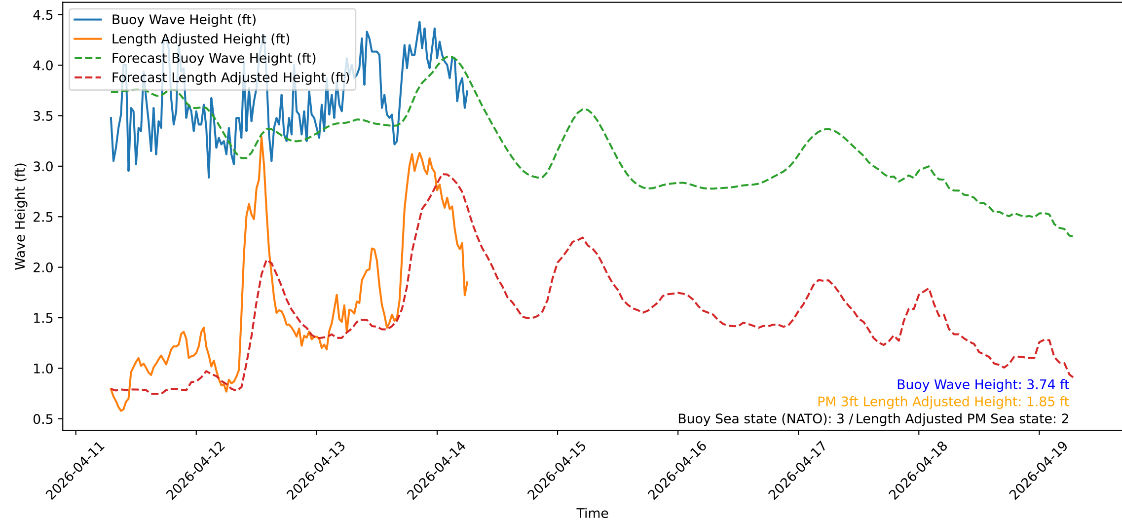
Wave Heights over Time for Red Beach at 2026-04-14 06:50:52
