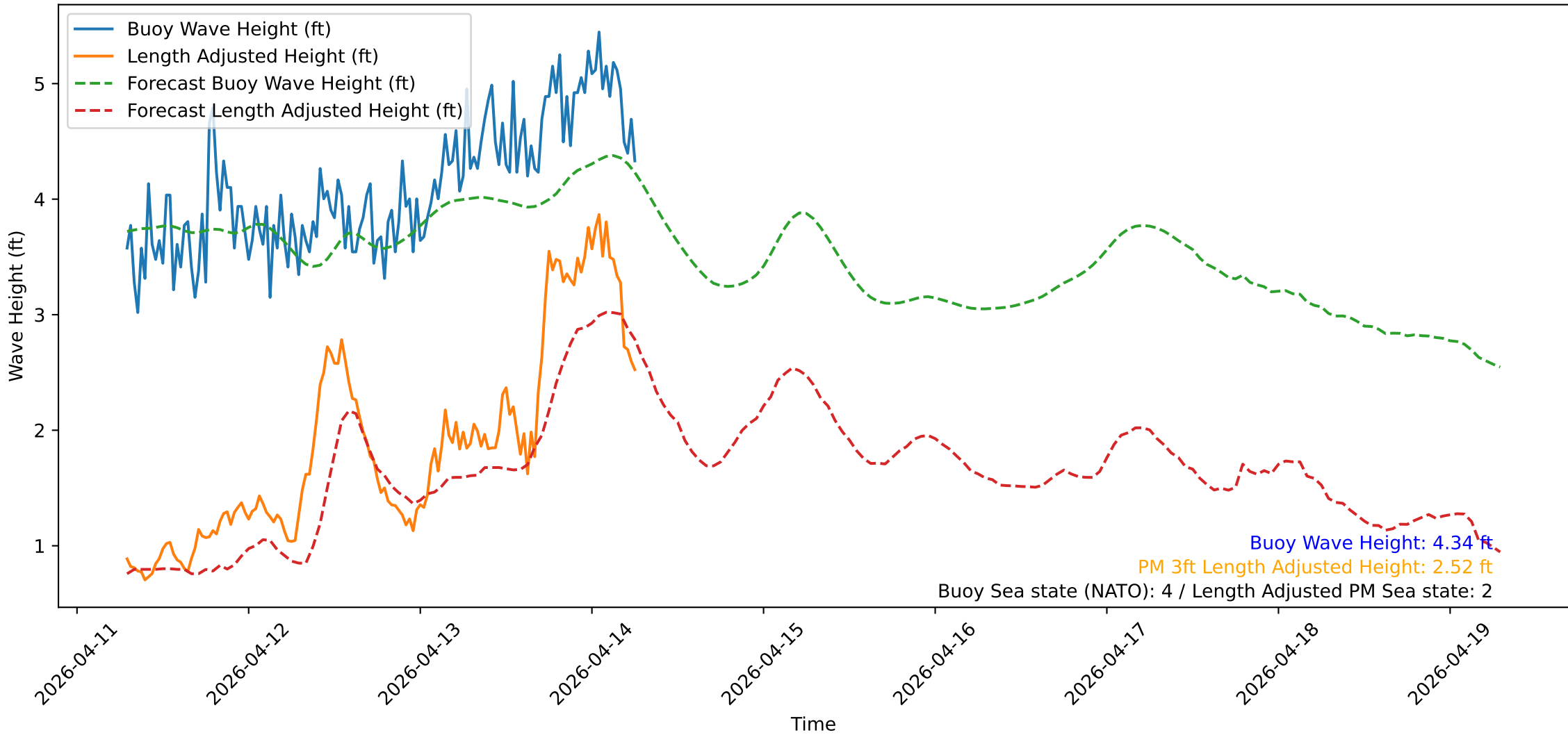
Wave Heights over Time for Oceanside Harbor at 2026-04-14 06:50:31
