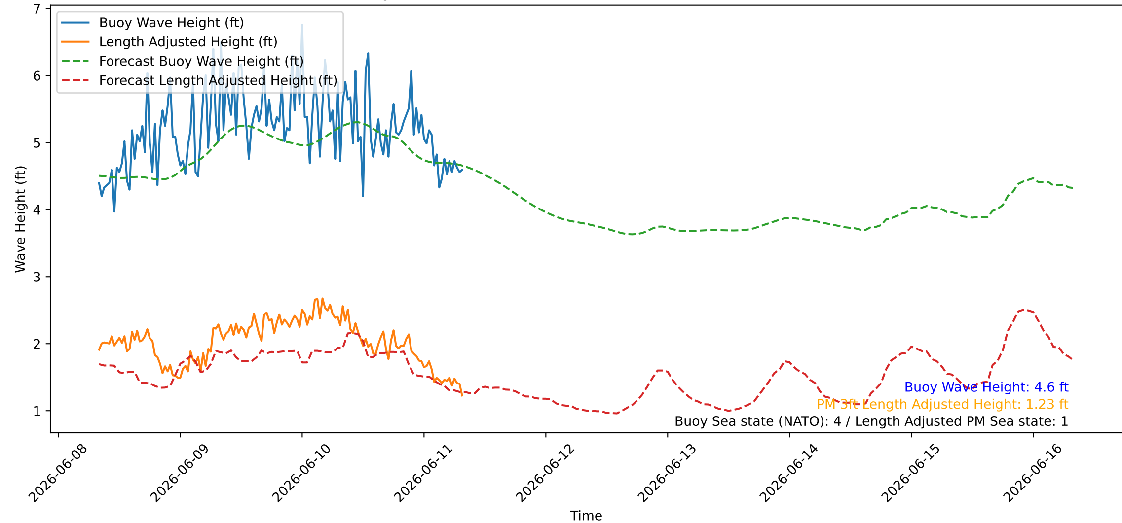
Wave Heights over Time for Oceanside Harbor at 2026-06-11 08:10:26
