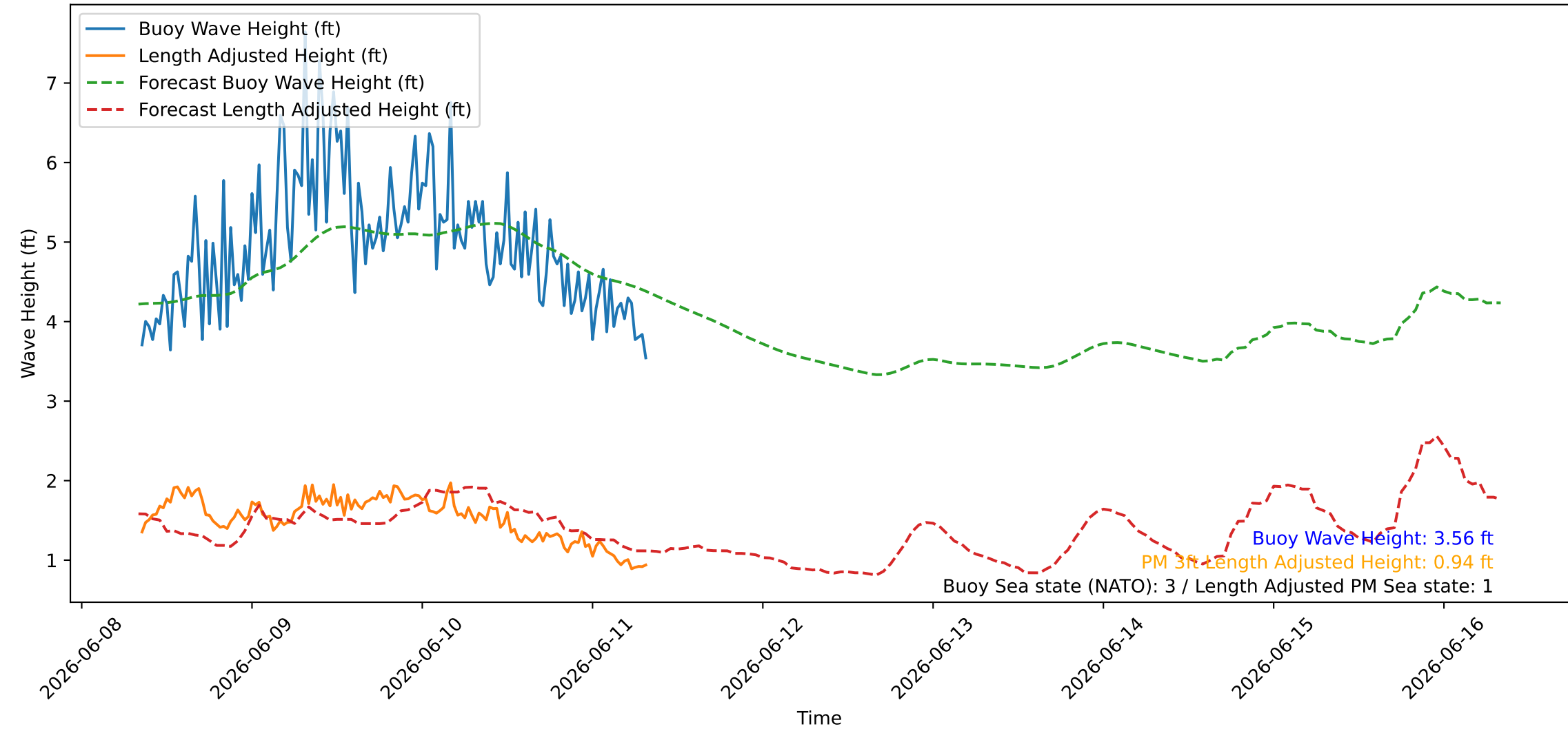
Wave Heights over Time for Red Beach at 2026-06-11 08:10:46
