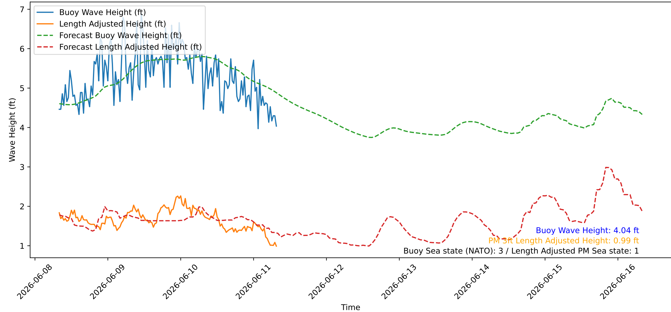
Wave Heights over Time for Green Beach at 2026-06-11 08:11:08
