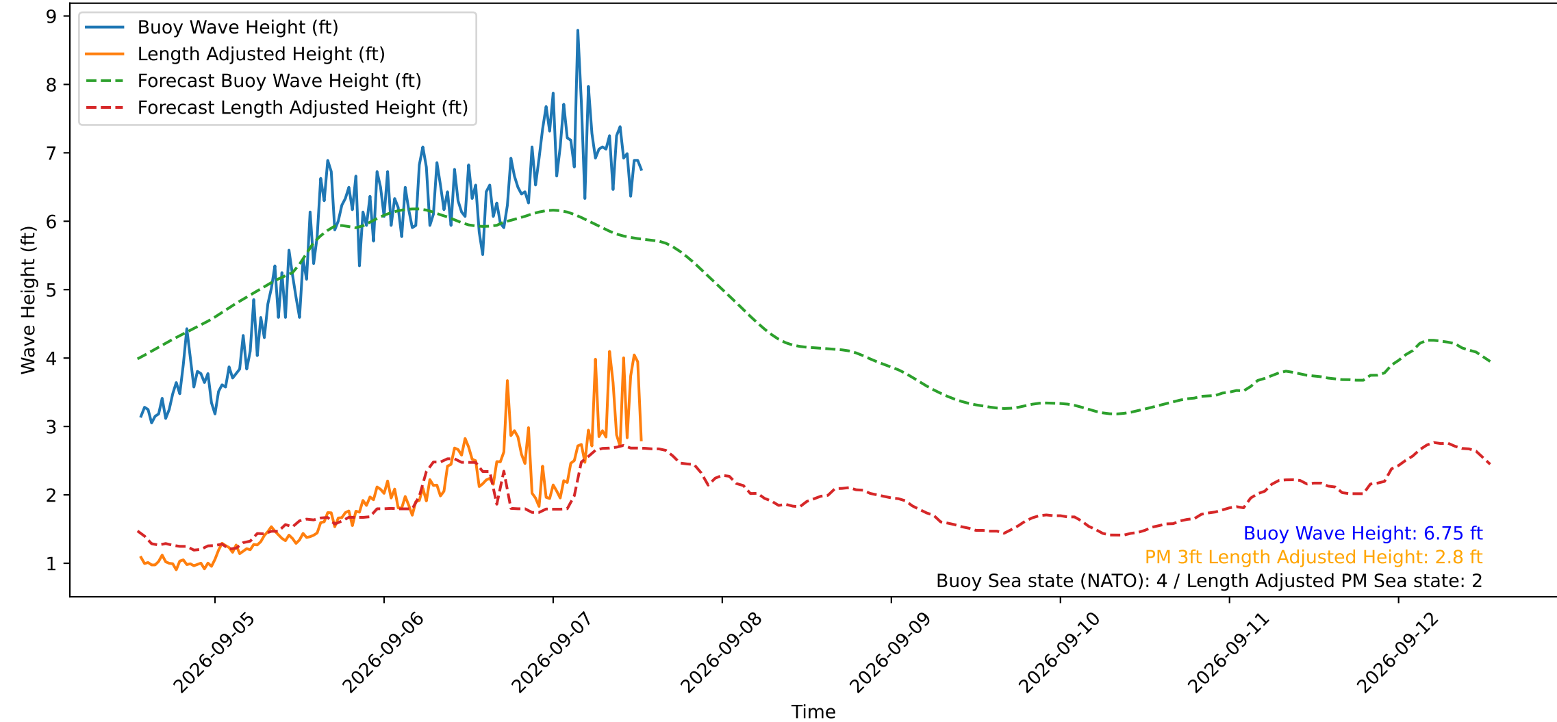
Wave Heights over Time for Green Beach at 2026-09-07 13:11:12
