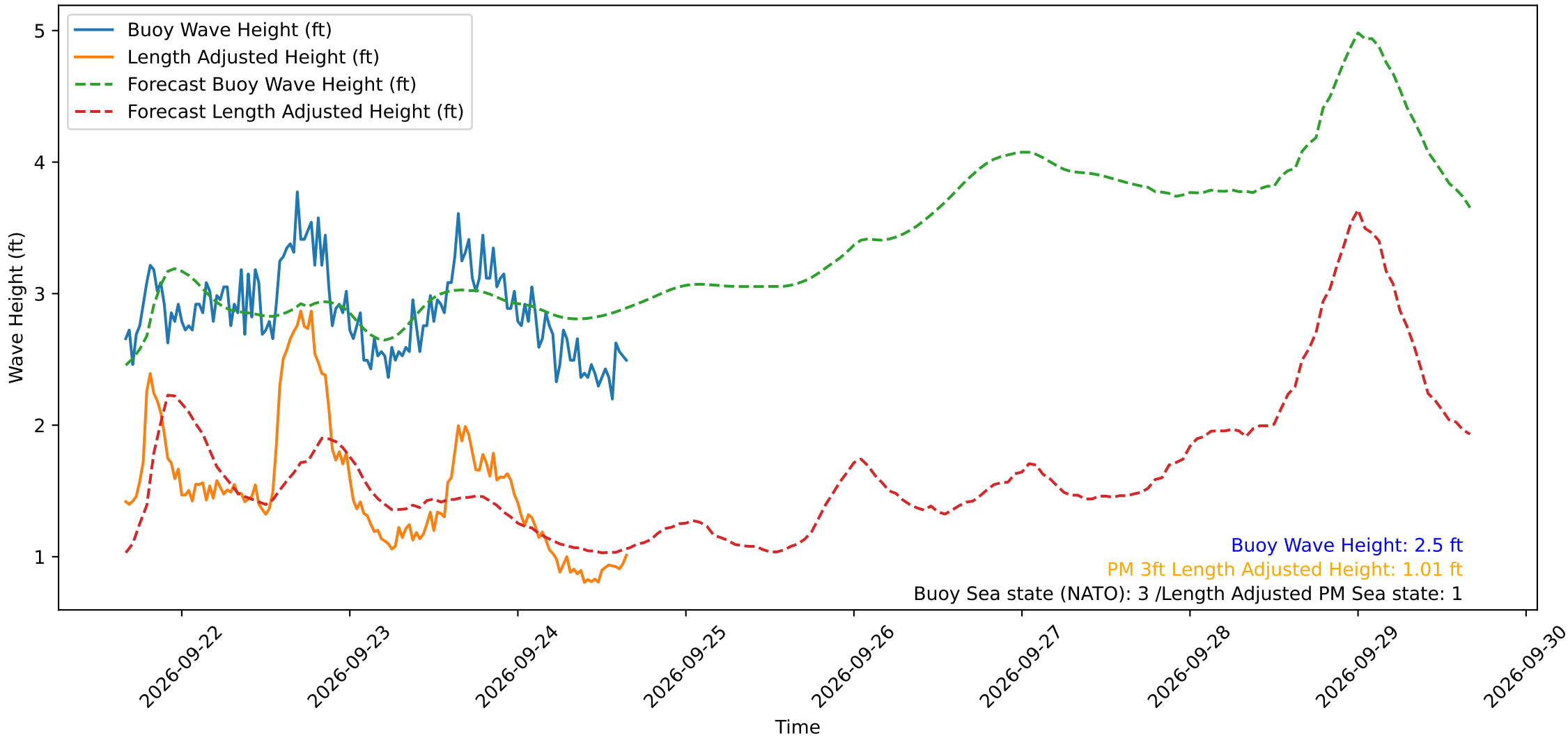
Wave Heights over Time for Oceanside Harbor at 2026-09-24 16:00:30
