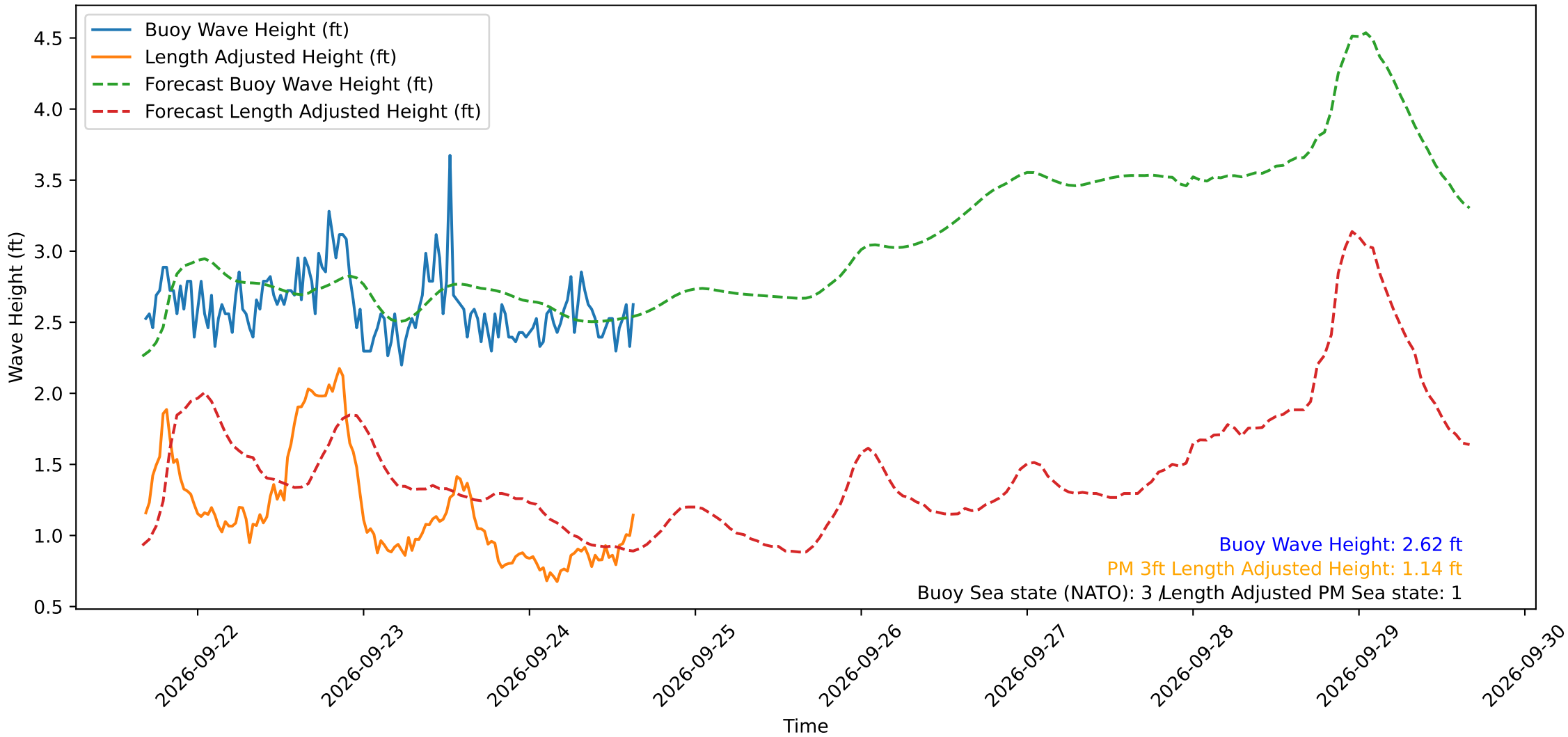
Wave Heights over Time for Red Beach at 2026-09-24 16:00:50
