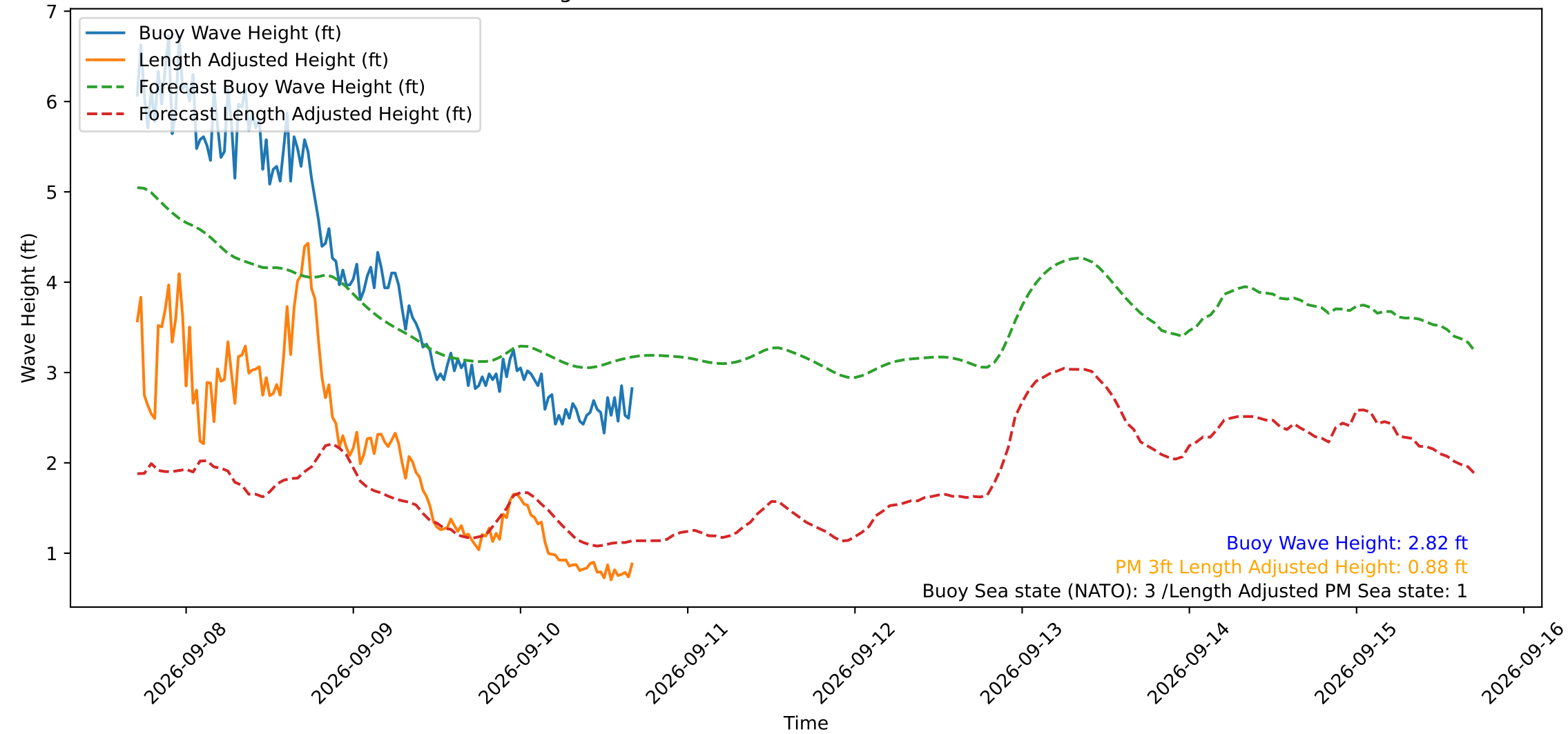
Wave Heights over Time for Red Beach at 2026-09-10 16:50:50
