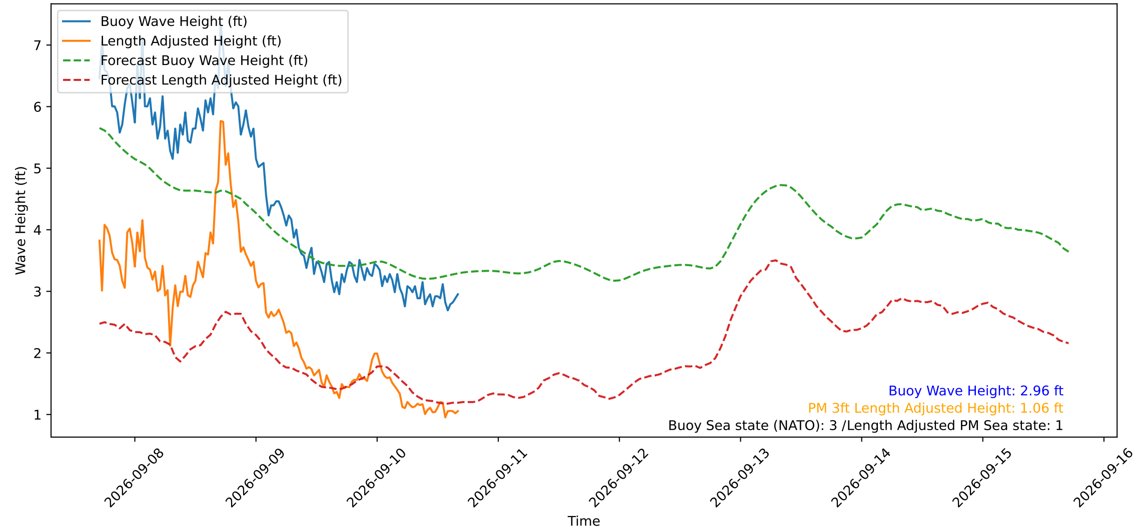
Wave Heights over Time for Oceanside Harbor at 2026-09-10 16:50:29
