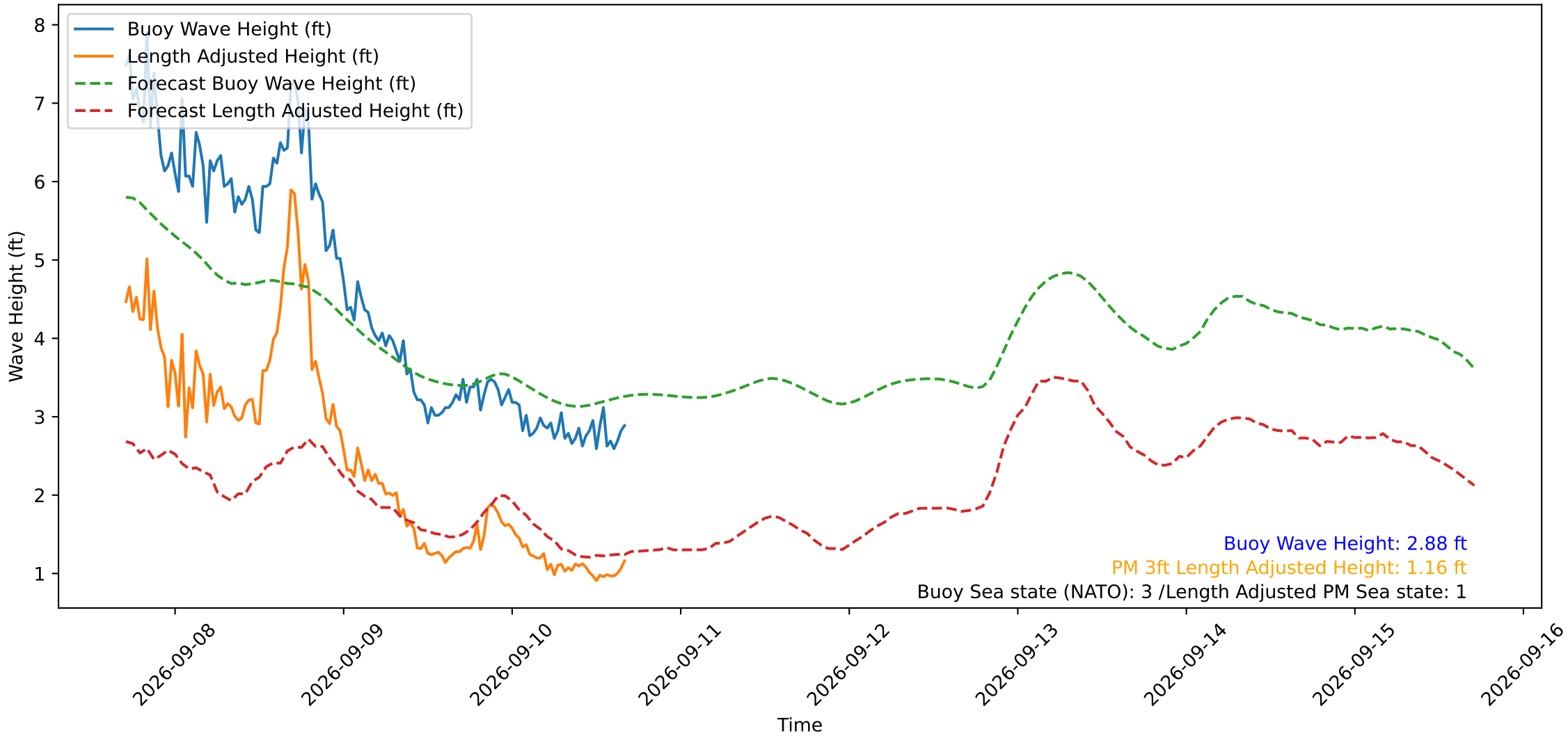
Wave Heights over Time for Green Beach at 2026-09-10 16:51:14
