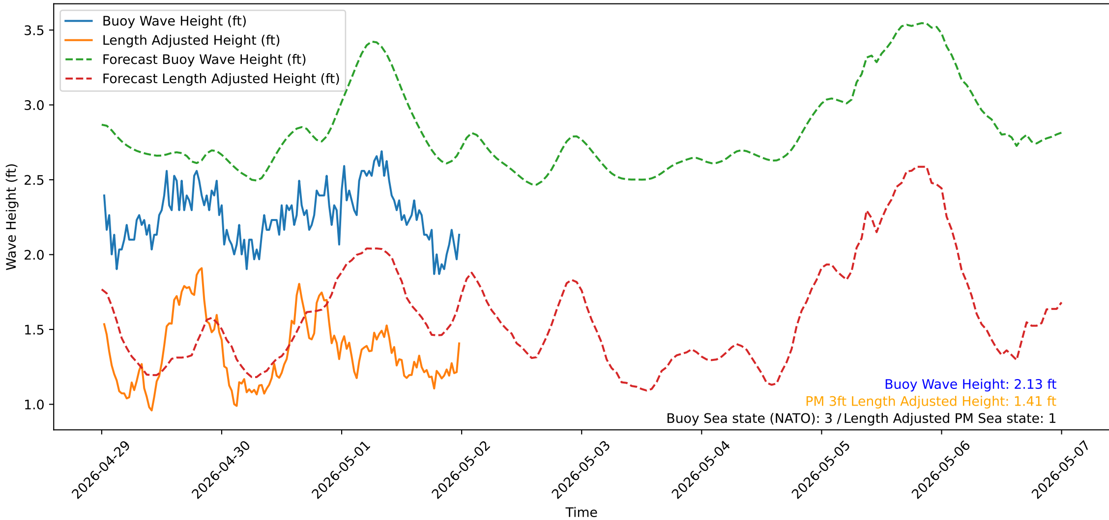
Wave Heights over Time for Oceanside Harbor at 2026-05-02 00:20:31
