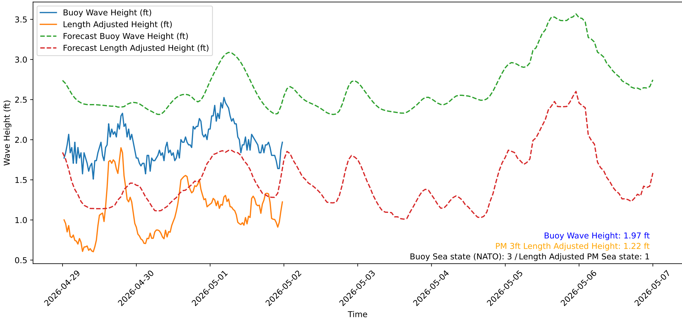
Wave Heights over Time for Red Beach at 2026-05-02 00:20:51
