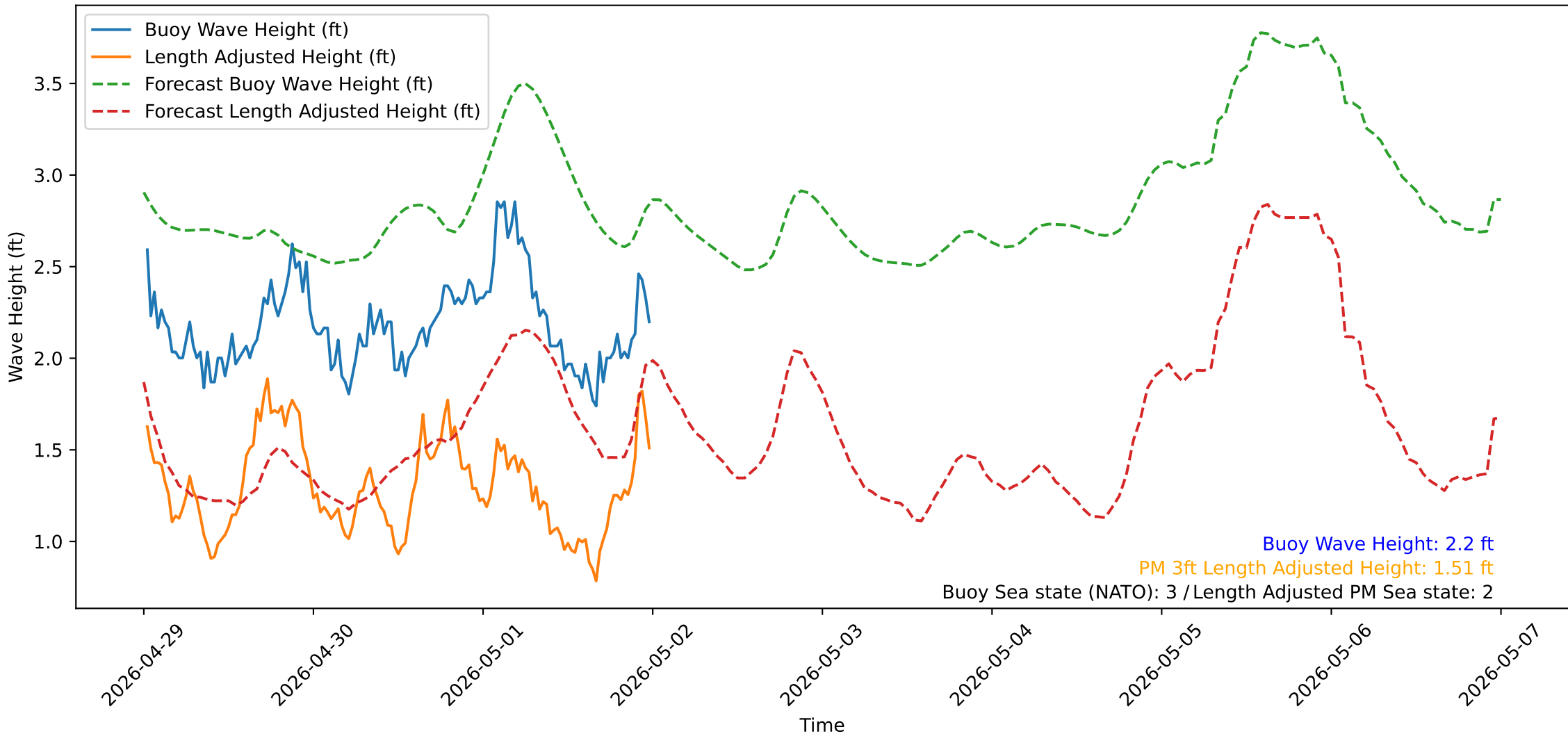
Wave Heights over Time for Green Beach at 2026-05-02 00:21:13
