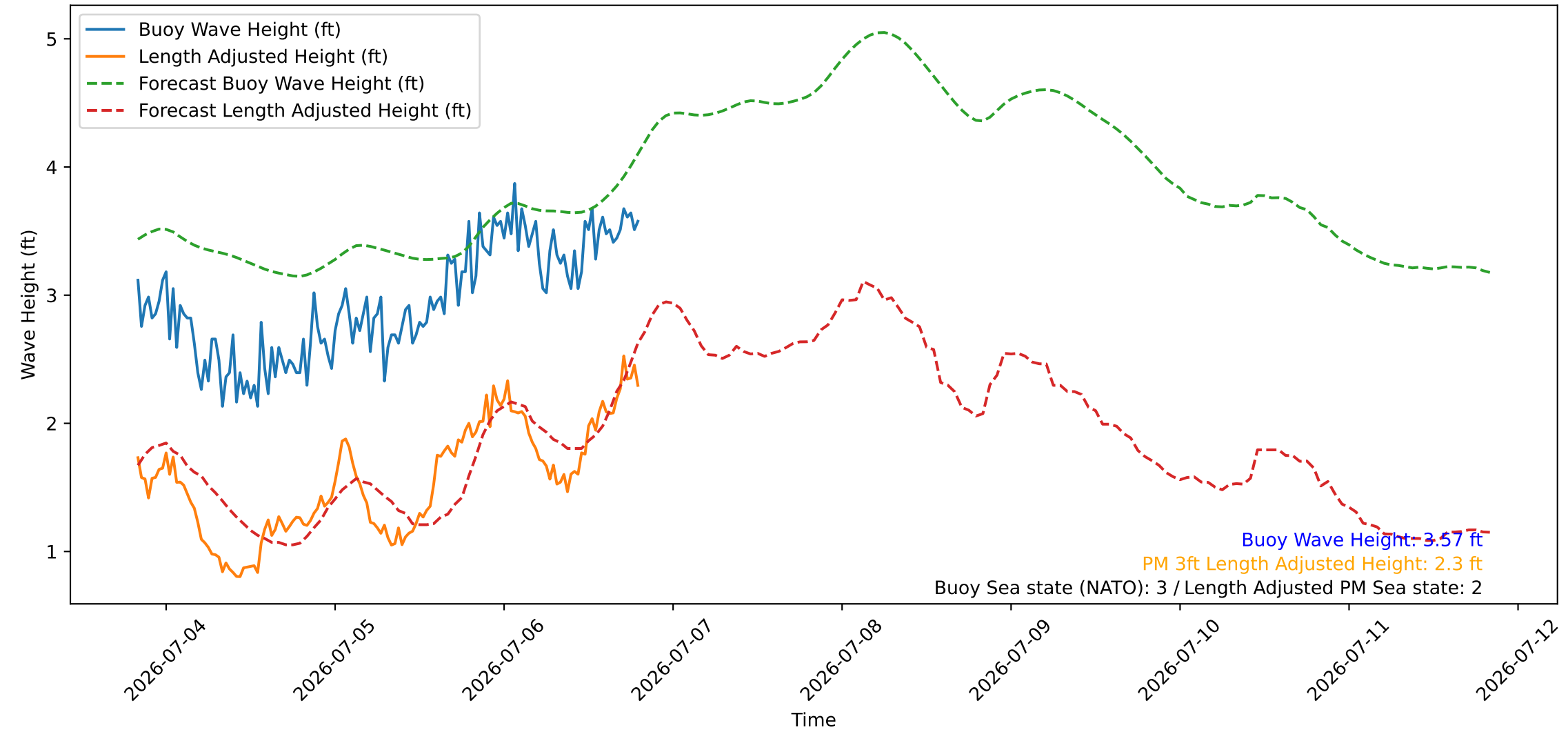
Wave Heights over Time for Oceanside Harbor at 2026-07-06 19:50:27
