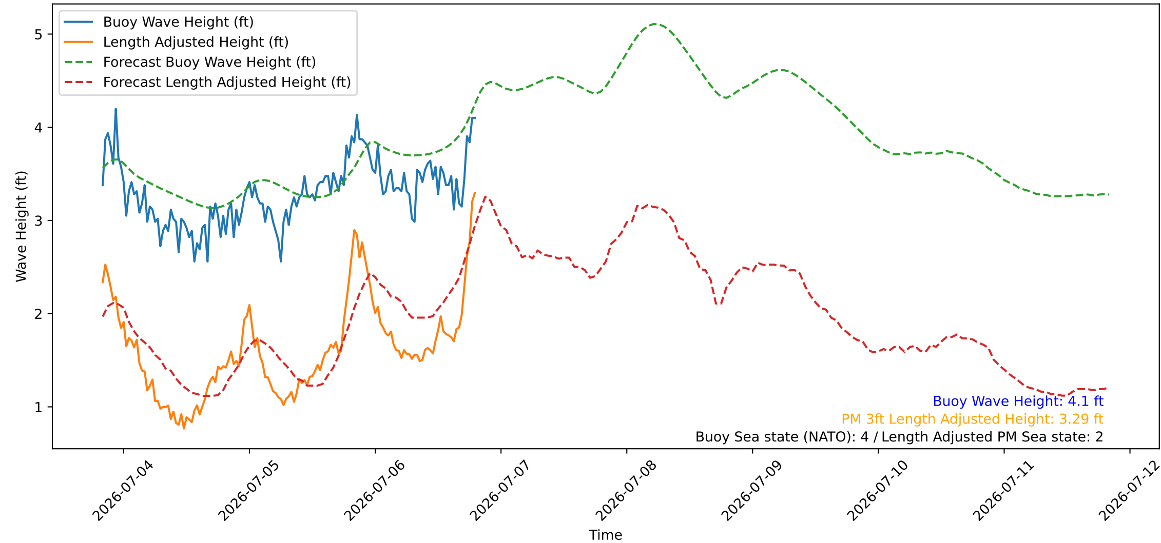
Wave Heights over Time for Green Beach at 2026-07-06 19:51:10
