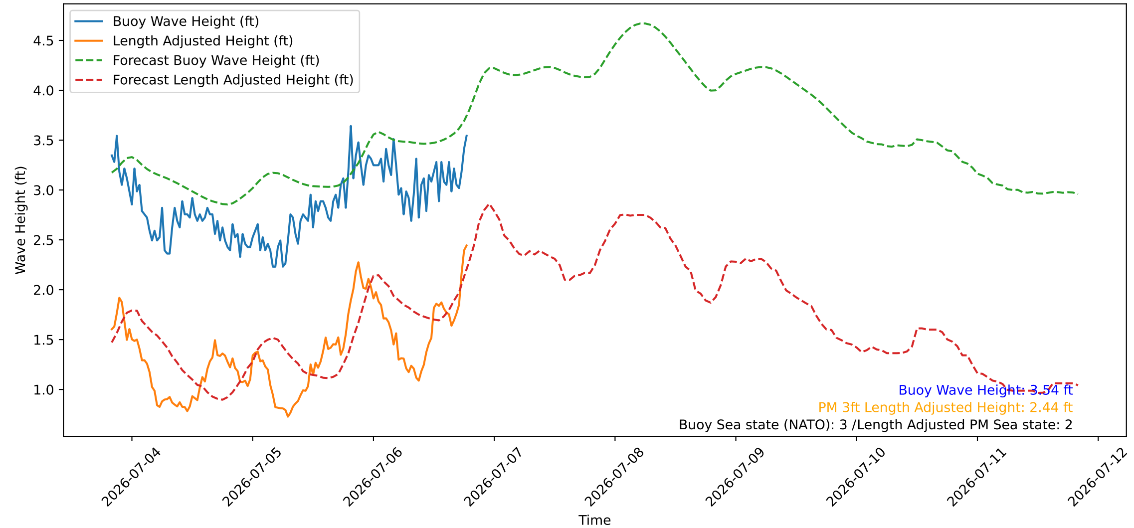
Wave Heights over Time for Red Beach at 2026-07-06 19:50:47
