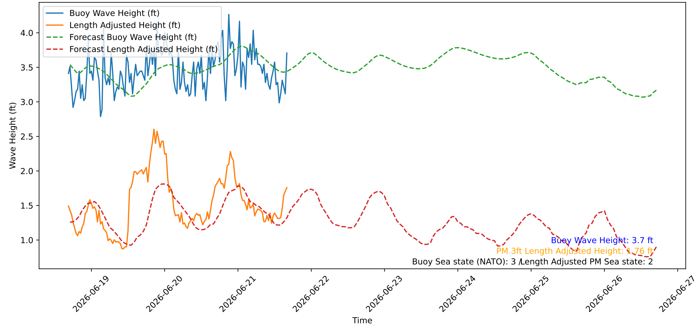
Wave Heights over Time for Oceanside Harbor at 2026-06-21 16:30:26
