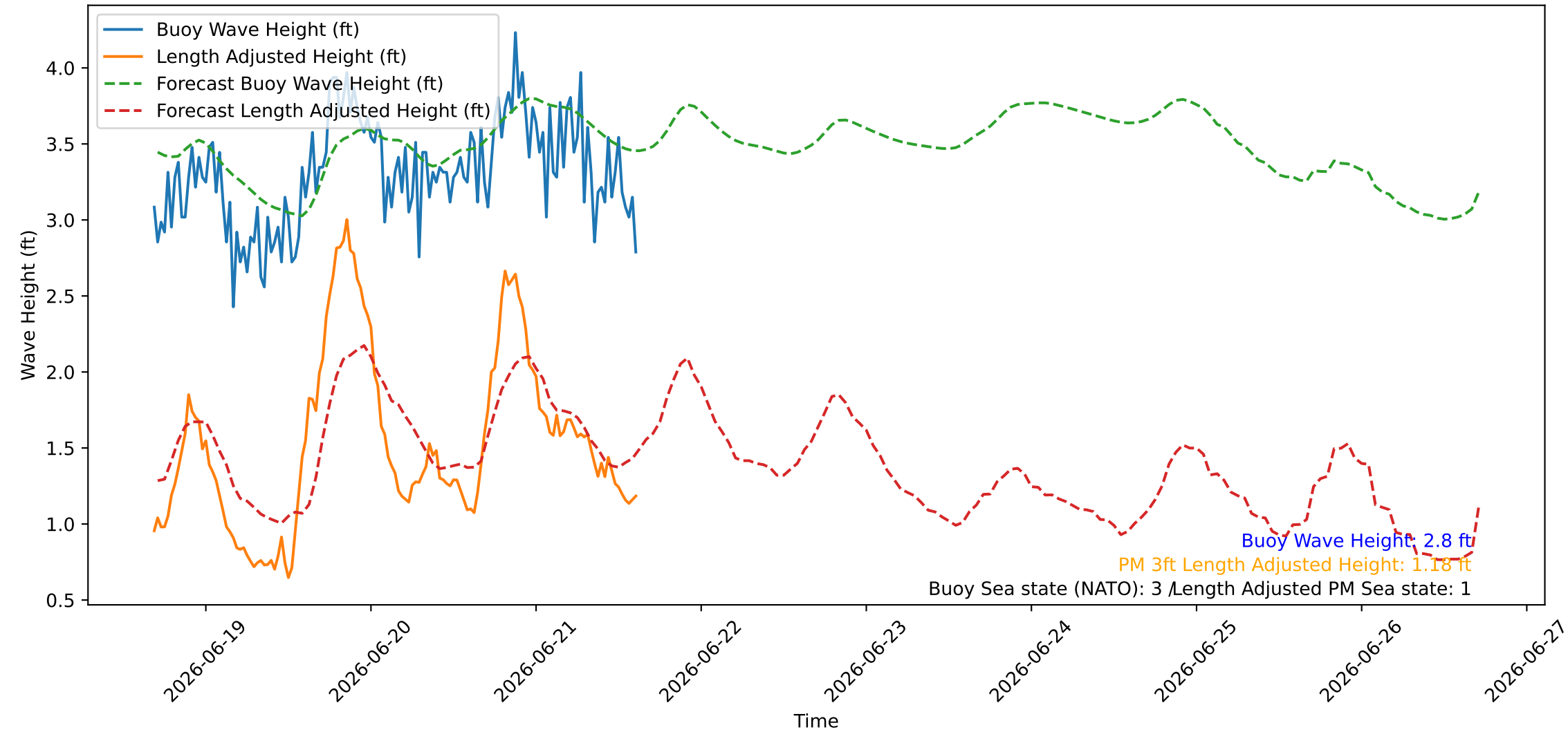
Wave Heights over Time for Green Beach at 2026-06-21 16:31:07
