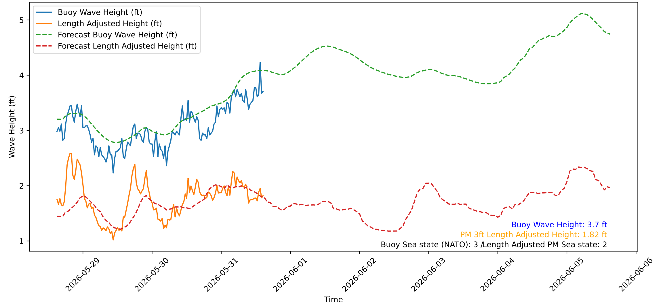
Wave Heights over Time for Oceanside Harbor at 2026-05-31 15:10:26
