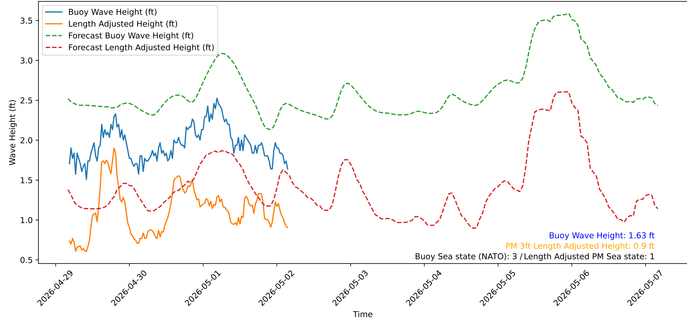
Wave Heights over Time for Red Beach at 2026-05-02 04:20:52
