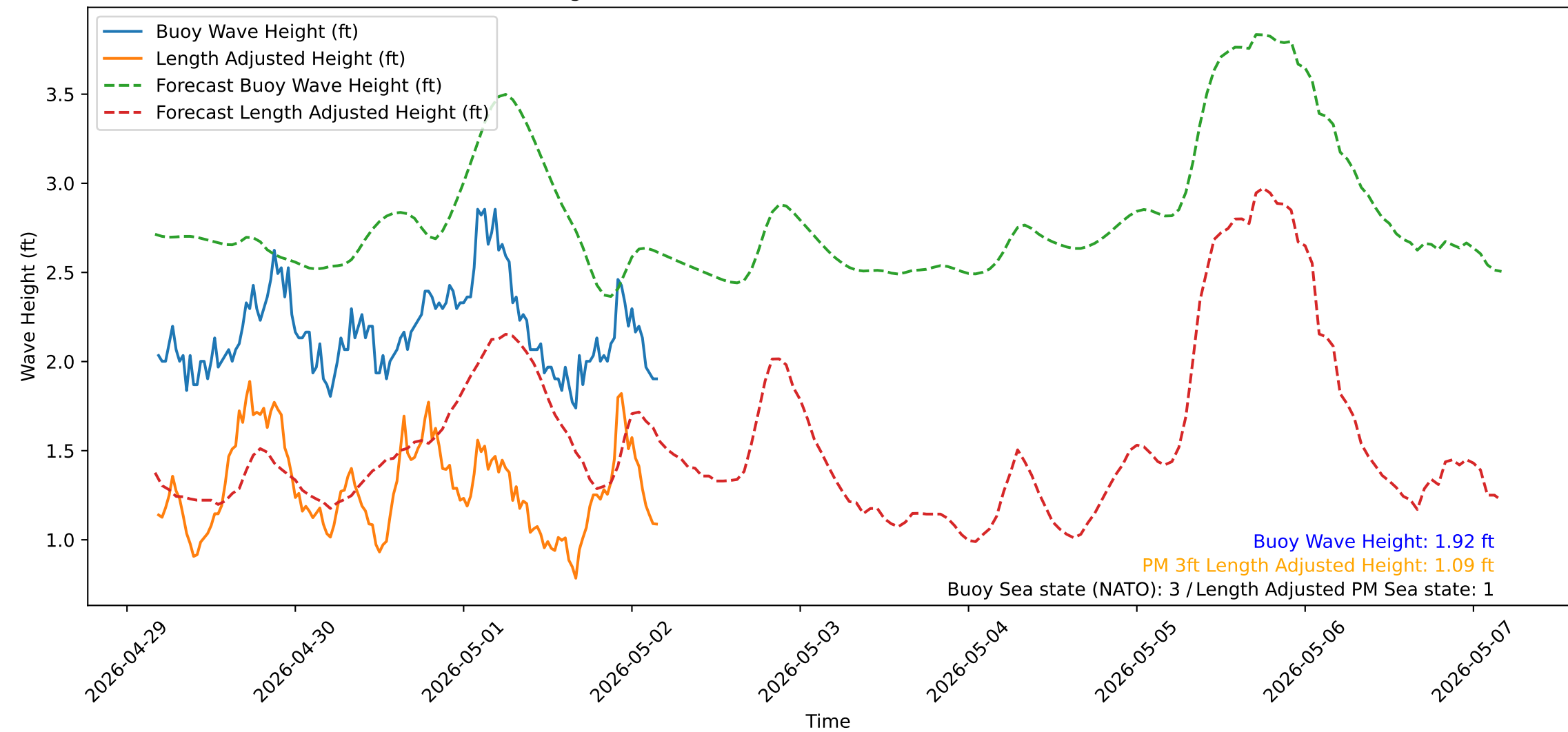
Wave Heights over Time for Green Beach at 2026-05-02 04:21:15
