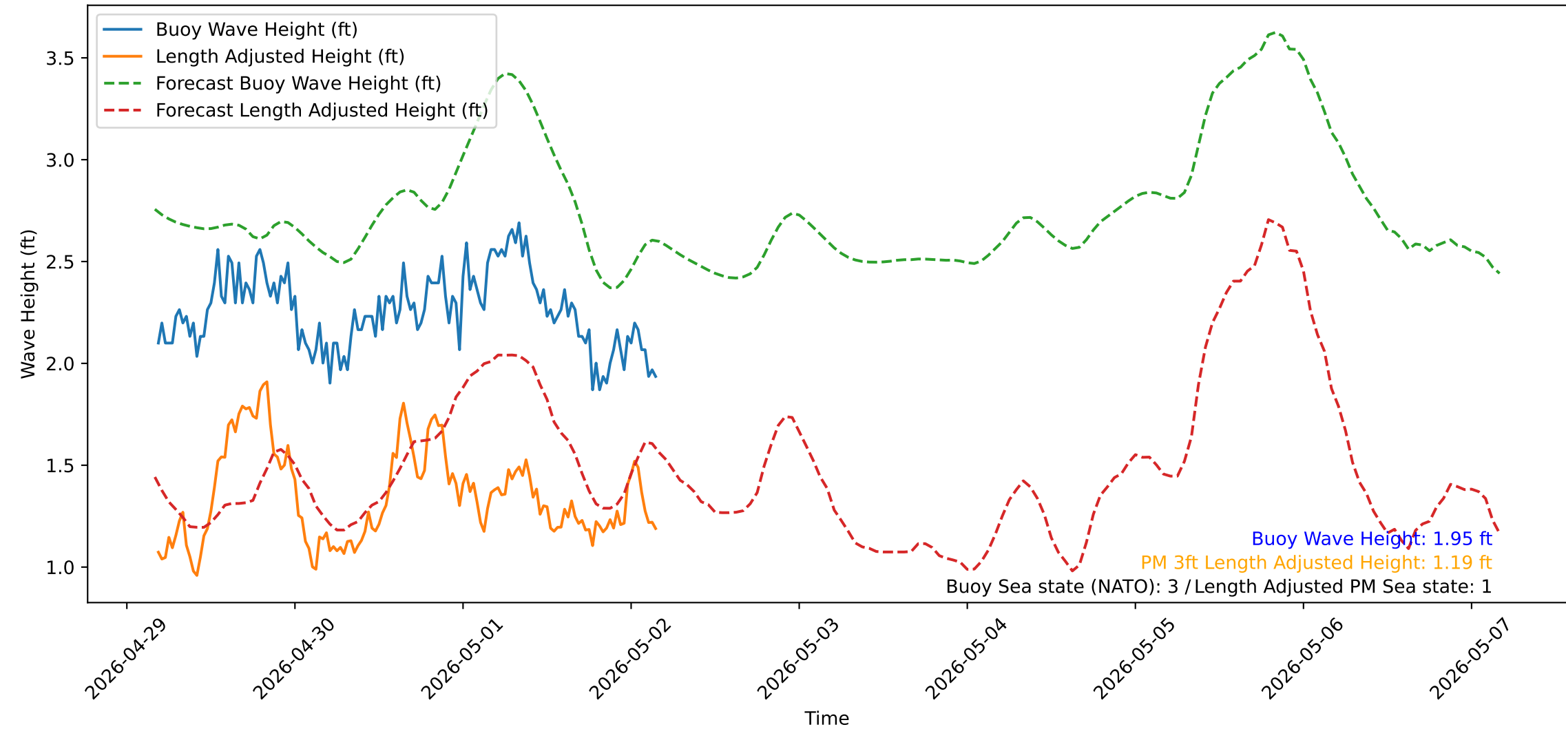
Wave Heights over Time for Oceanside Harbor at 2026-05-02 04:20:31
