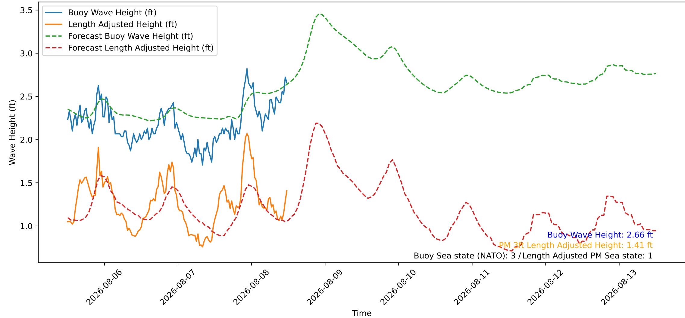
Wave Heights over Time for Green Beach at 2026-08-08 12:11:08
