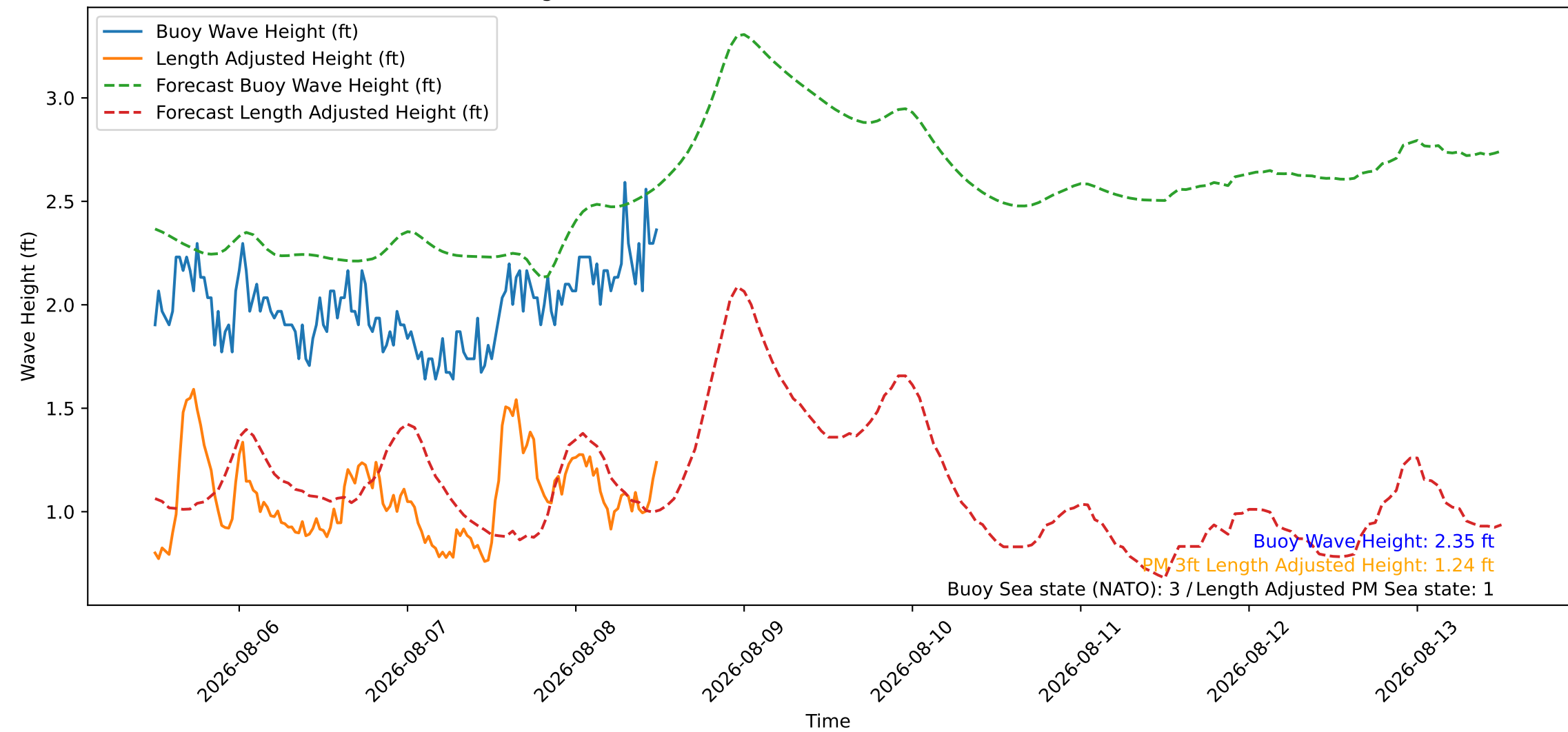
Wave Heights over Time for Oceanside Harbor at 2026-08-08 12:10:26
