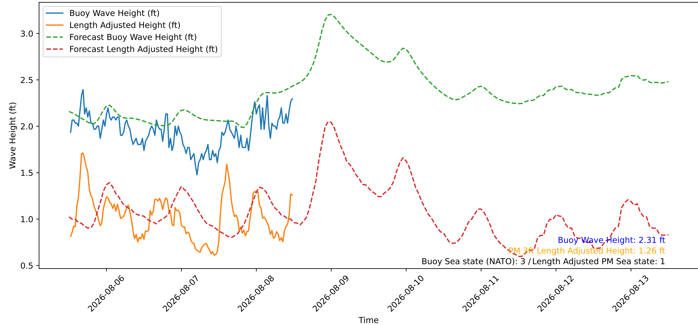
Wave Heights over Time for Red Beach at 2026-08-08 12:10:45
