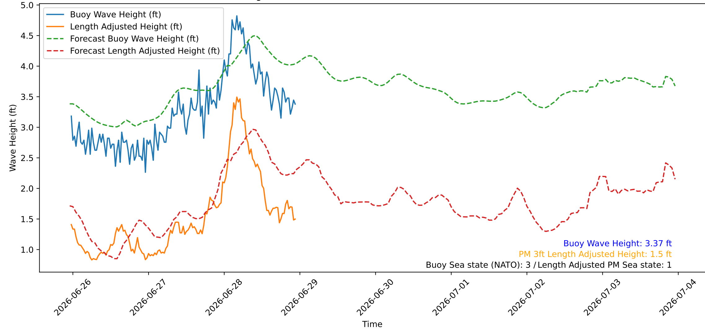
Wave Heights over Time for Green Beach at 2026-06-28 23:21:08
