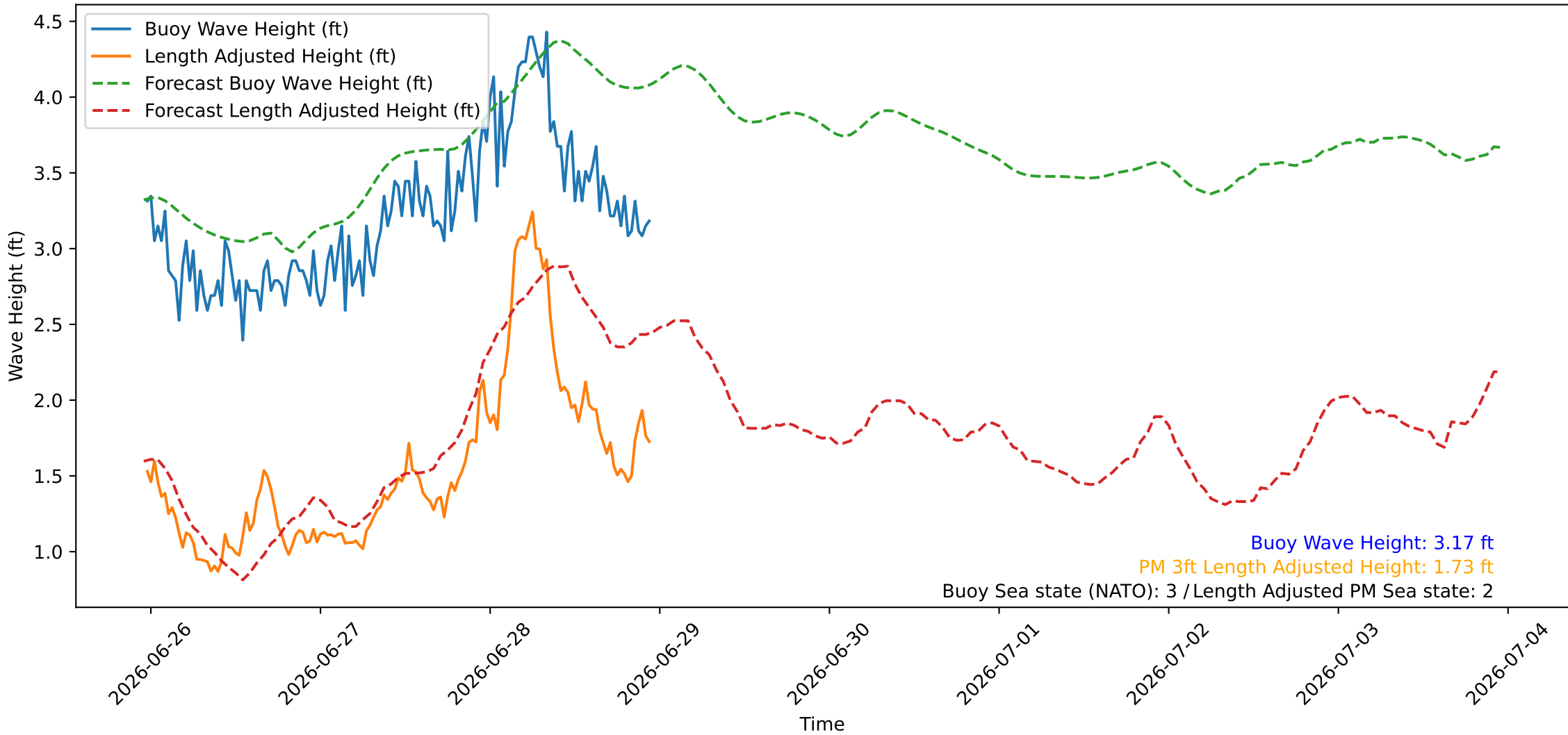
Wave Heights over Time for Oceanside Harbor at 2026-06-28 23:20:26
