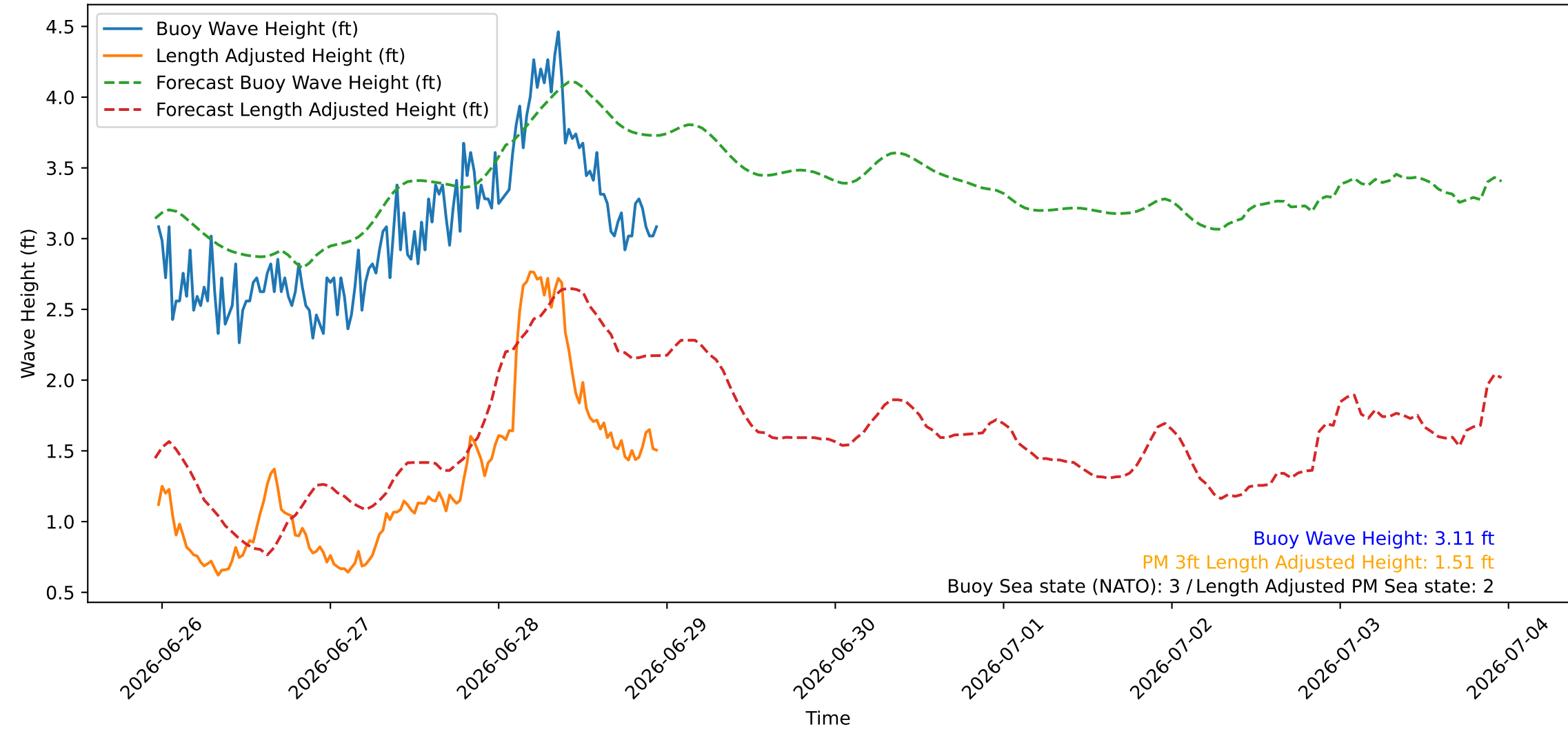
Wave Heights over Time for Red Beach at 2026-06-28 23:20:46
