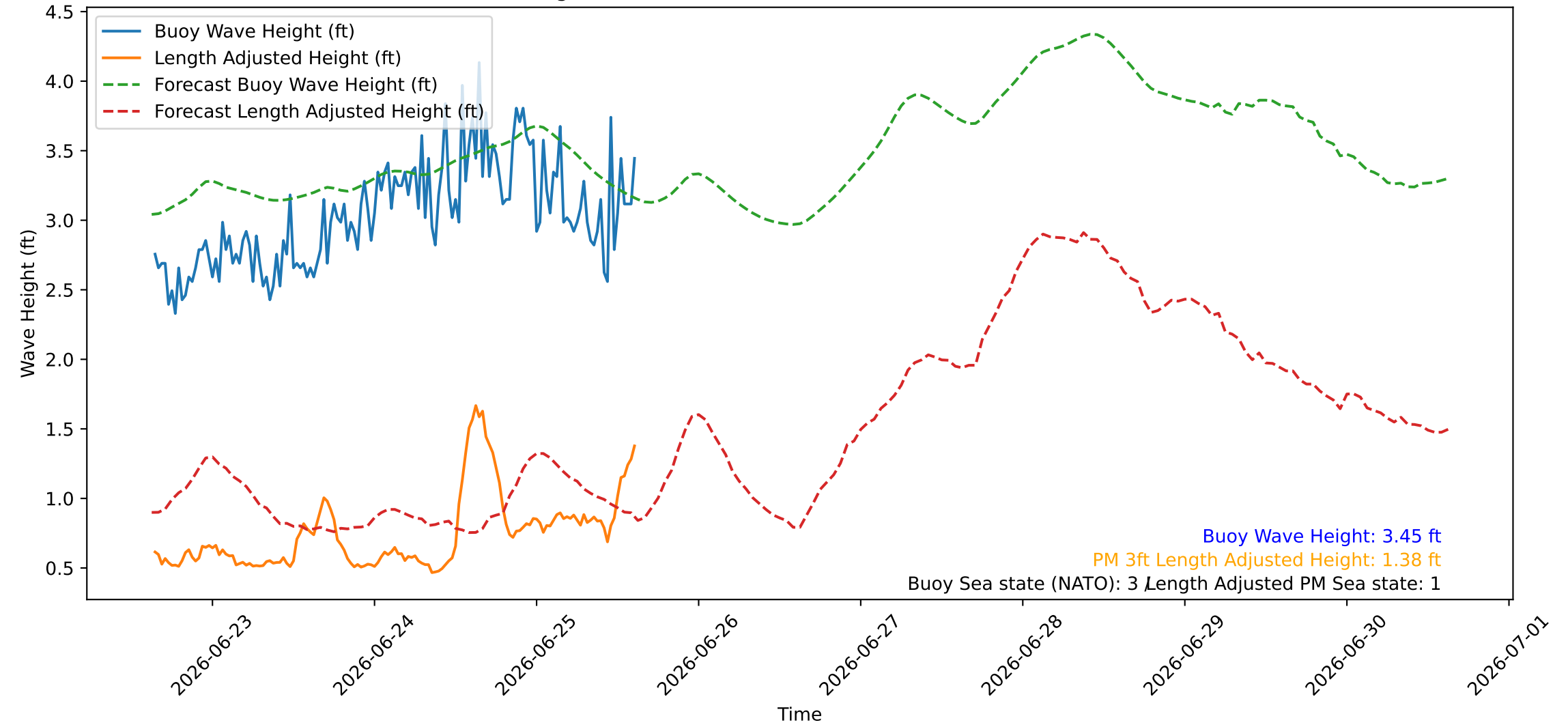
Wave Heights over Time for Red Beach at 2026-06-25 15:10:46
