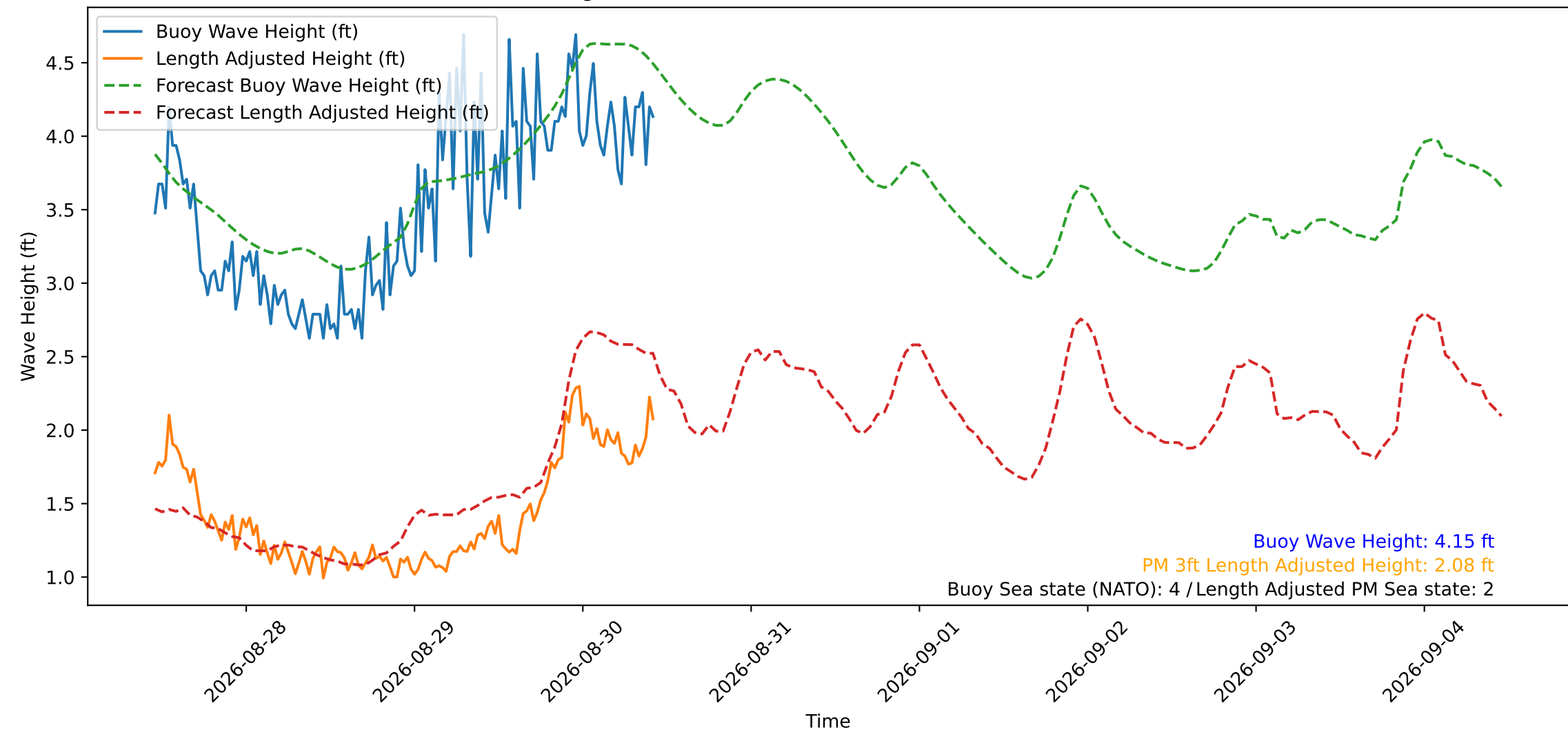
Wave Heights over Time for Red Beach at 2026-08-30 10:50:51
