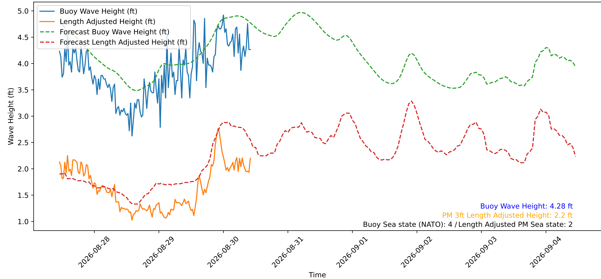
Wave Heights over Time for Green Beach at 2026-08-30 10:51:15
