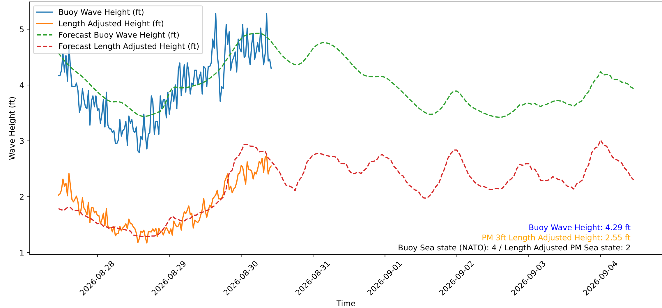
Wave Heights over Time for Oceanside Harbor at 2026-08-30 10:50:30
