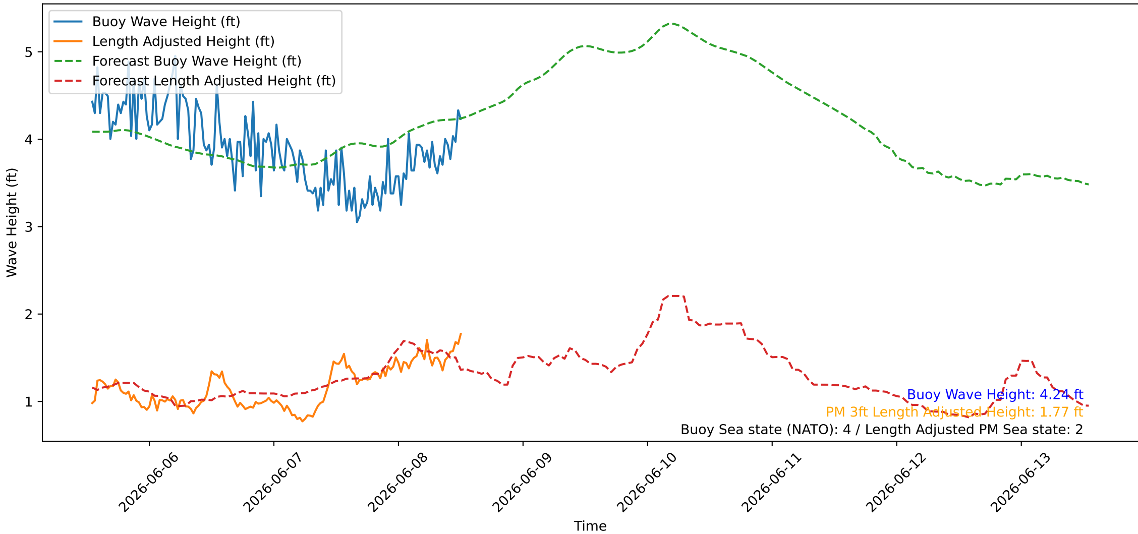
Wave Heights over Time for Red Beach at 2026-06-08 12:40:45
