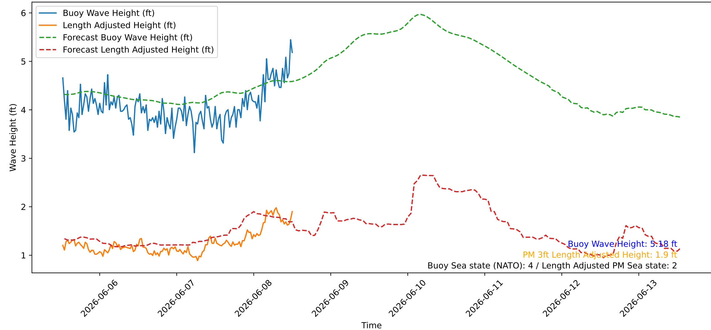
Wave Heights over Time for Green Beach at 2026-06-08 12:41:07
