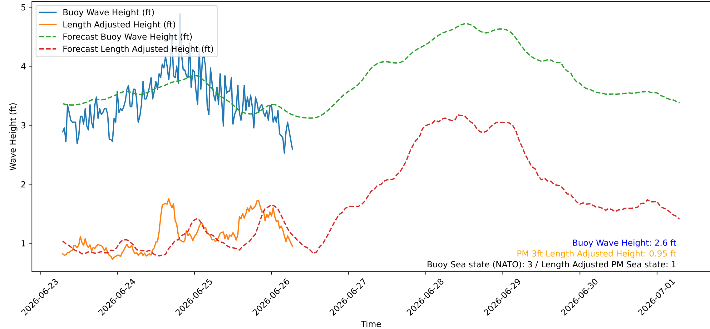
Wave Heights over Time for Oceanside Harbor at 2026-06-26 07:00:26
