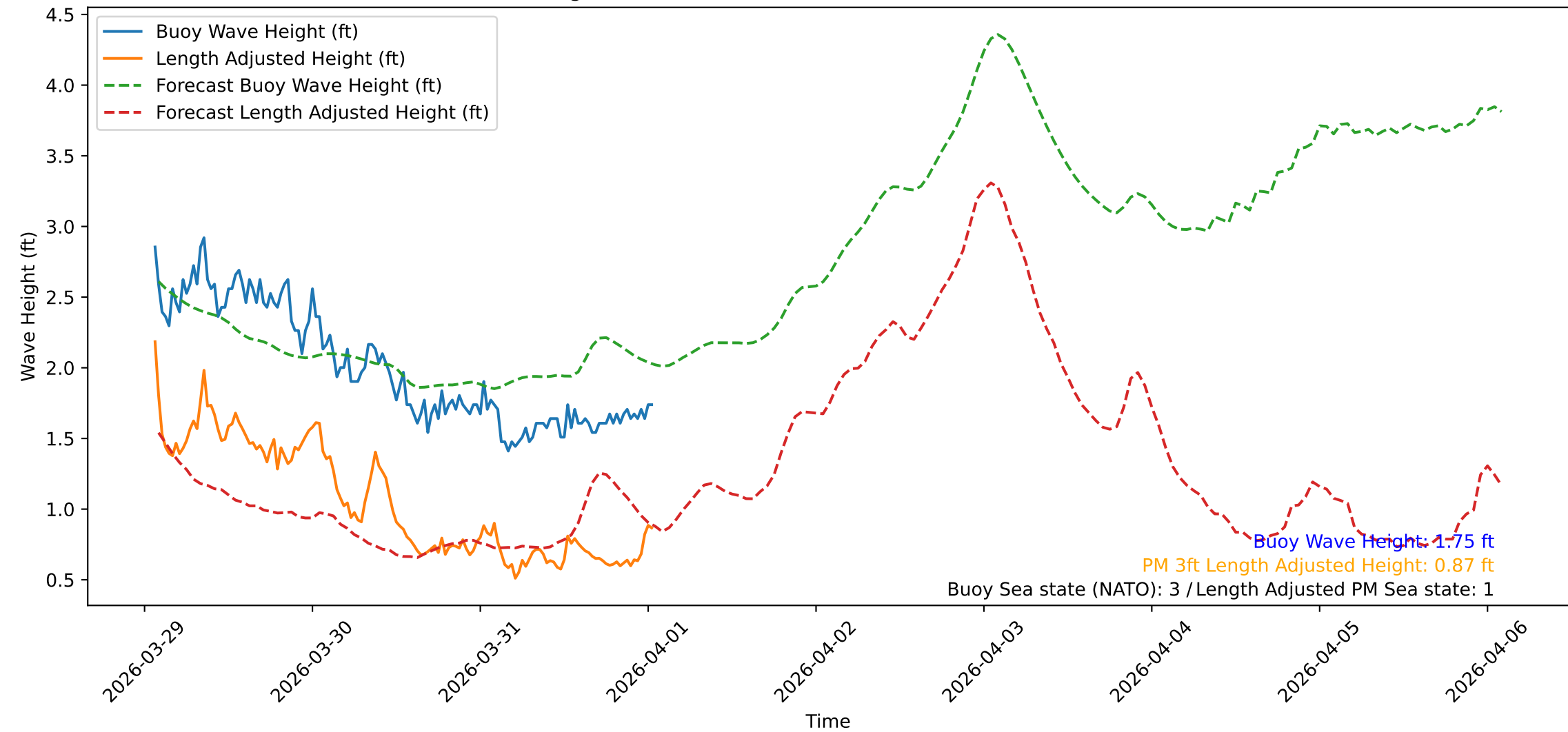
Wave Heights over Time for Green Beach at 2026-04-01 01:31:09
