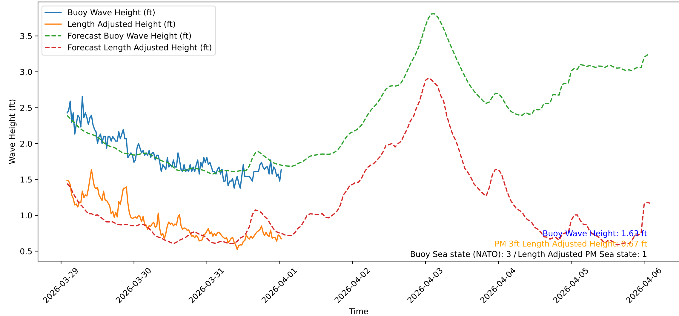
Wave Heights over Time for Red Beach at 2026-04-01 01:30:47
