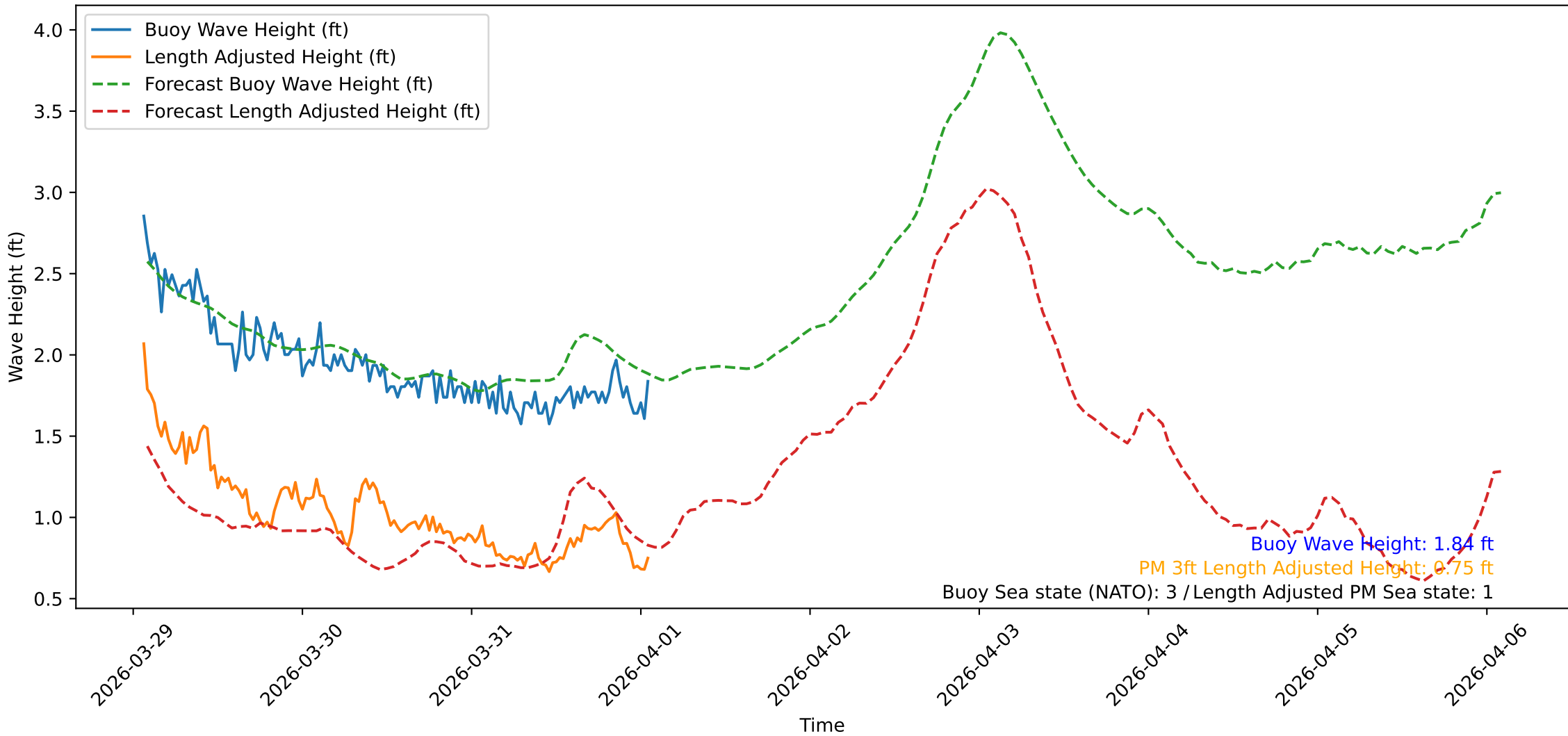
Wave Heights over Time for Oceanside Harbor at 2026-04-01 01:30:31
