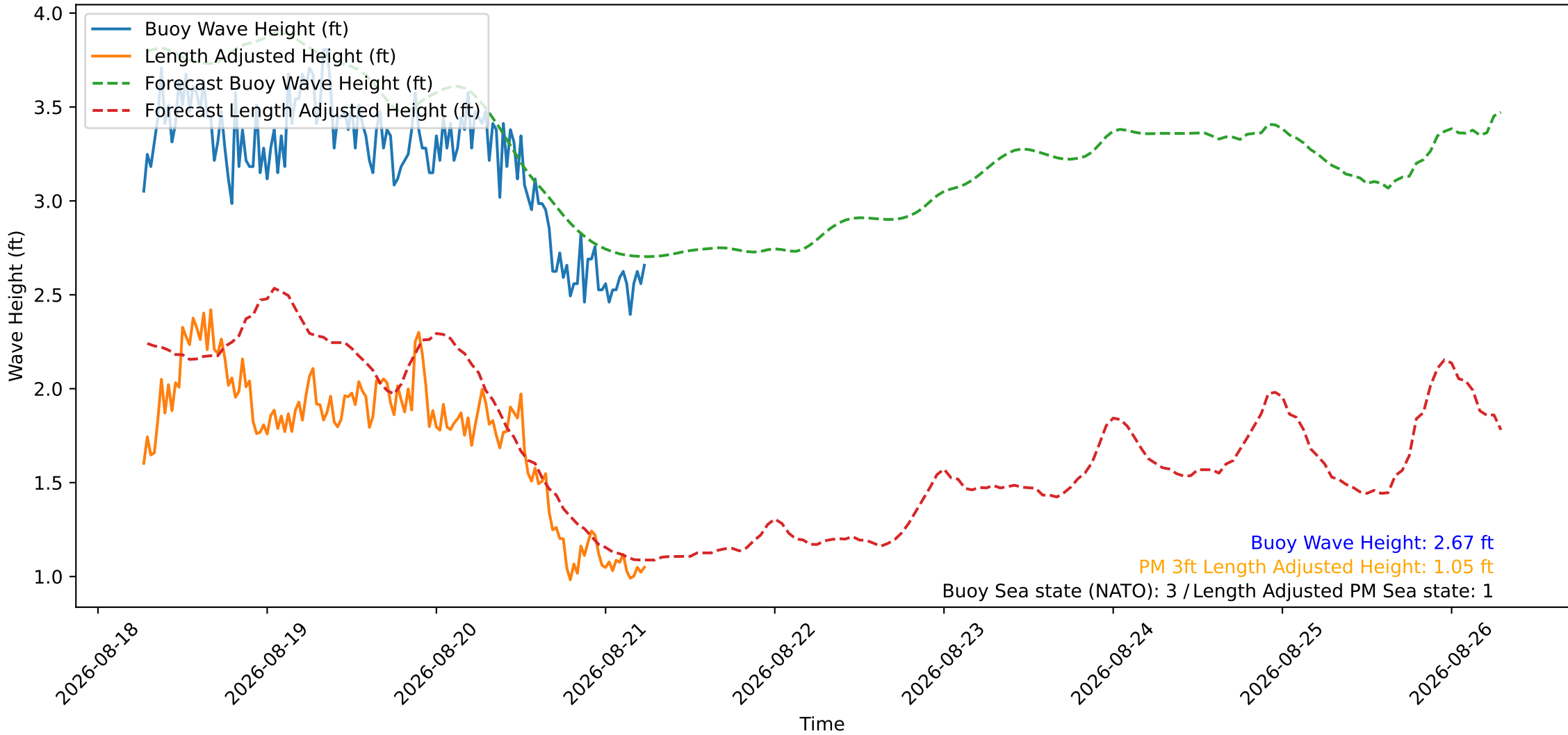
Wave Heights over Time for Oceanside Harbor at 2026-08-21 06:30:26
