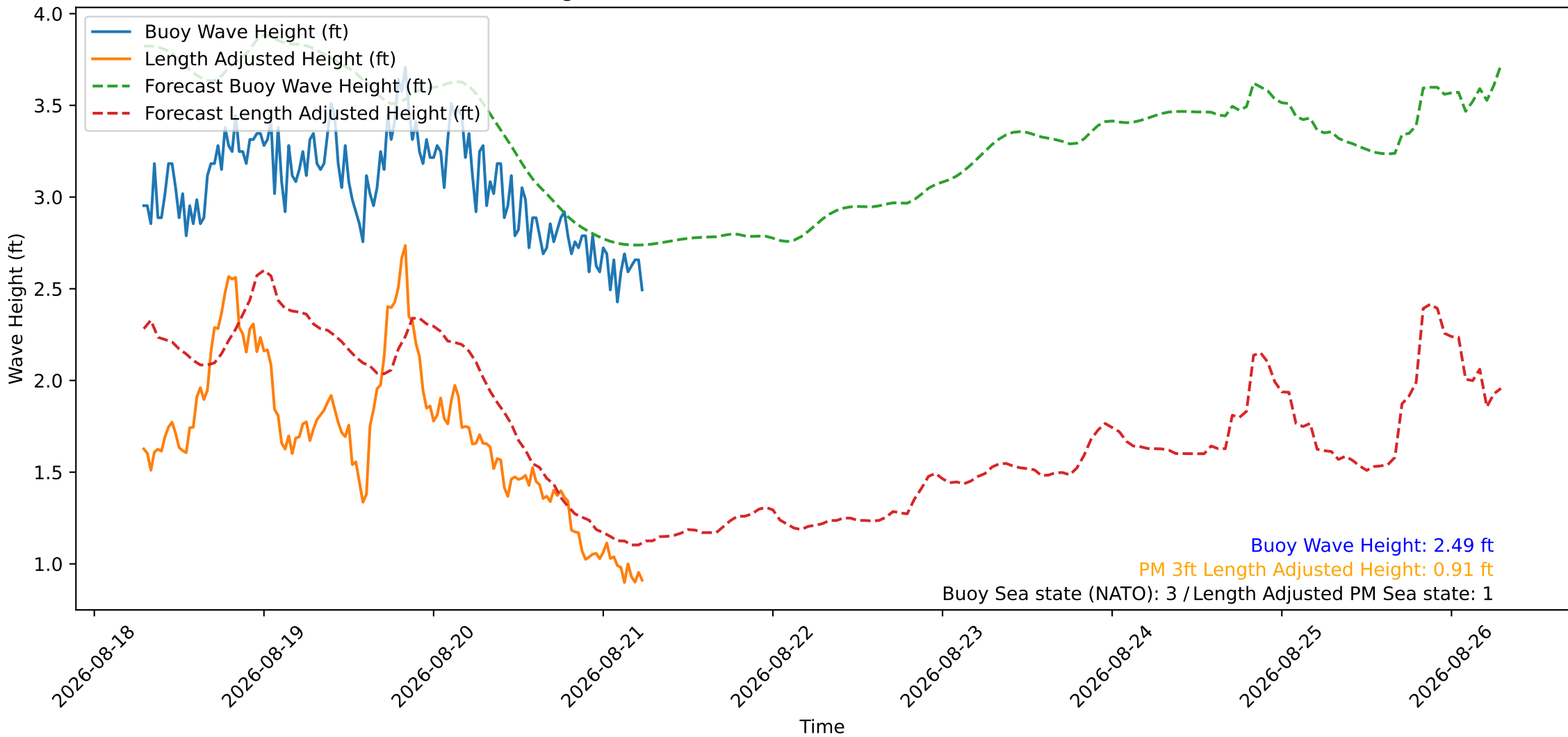
Wave Heights over Time for Green Beach at 2026-08-21 06:31:08
