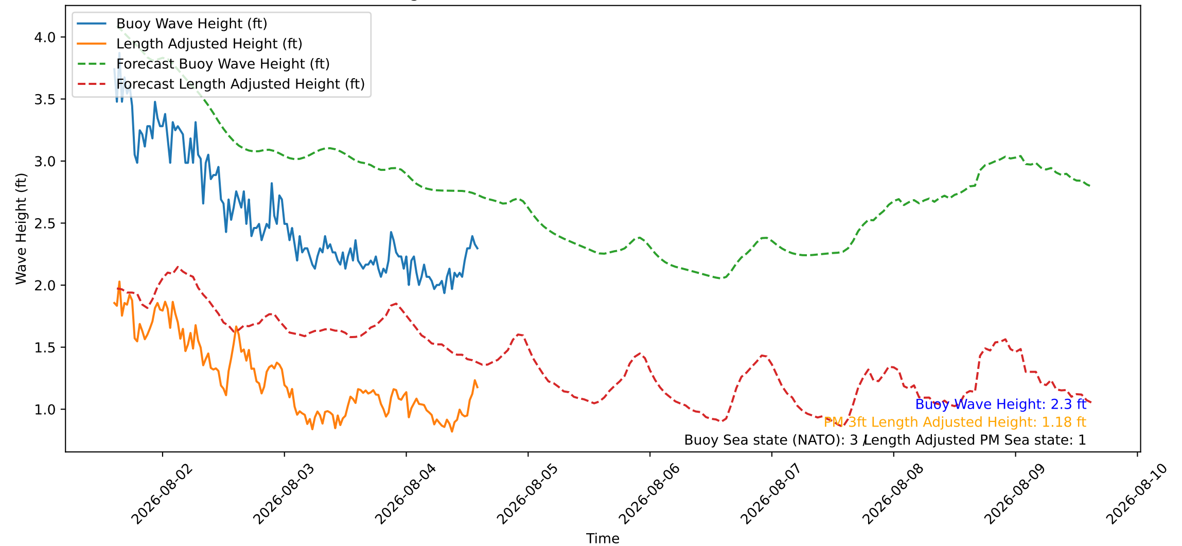
Wave Heights over Time for Green Beach at 2026-08-04 14:41:09
