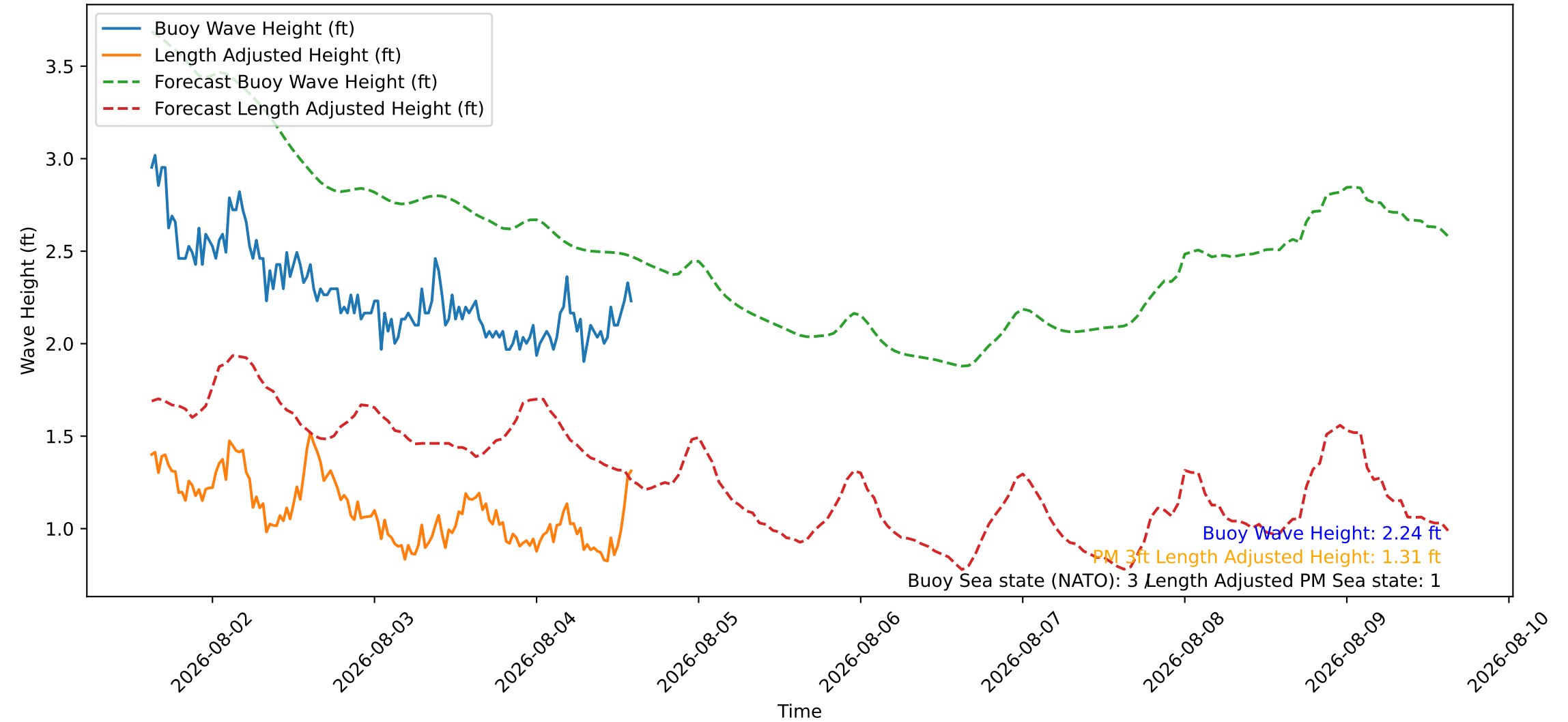
Wave Heights over Time for Red Beach at 2026-08-04 14:40:47
