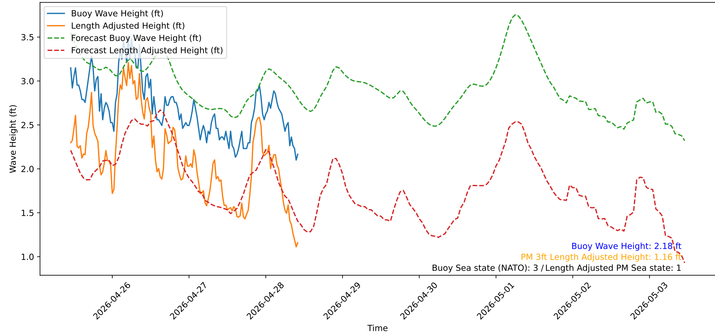
Wave Heights over Time for Green Beach at 2026-04-28 11:01:14
