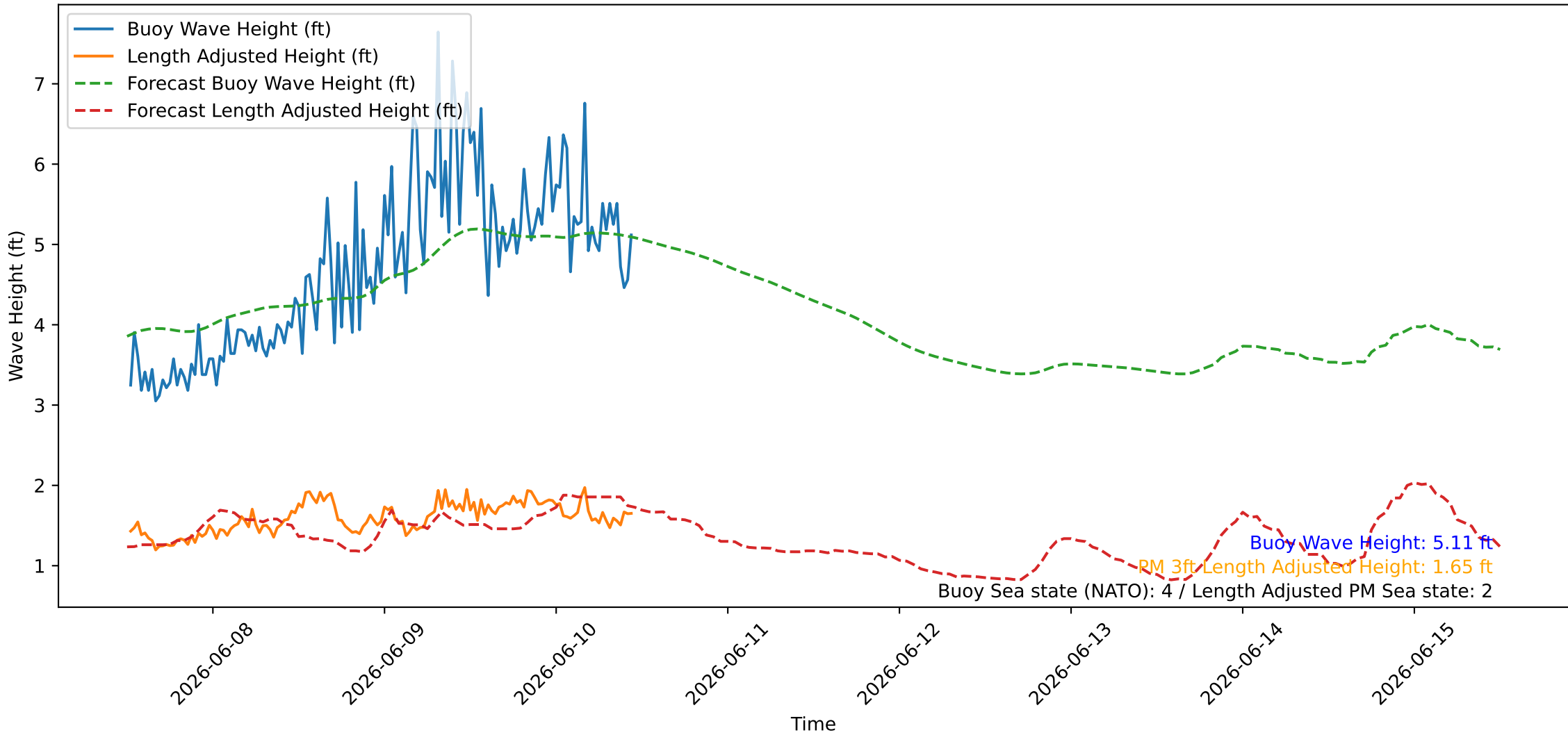
Wave Heights over Time for Red Beach at 2026-06-10 12:00:46
