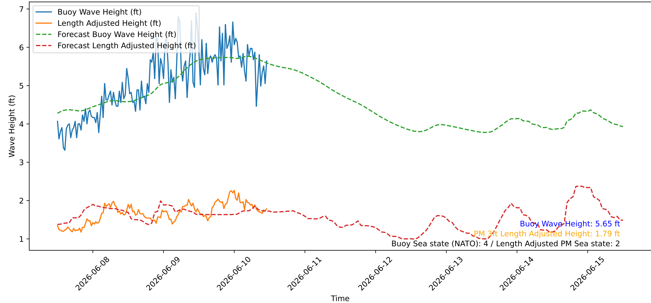
Wave Heights over Time for Green Beach at 2026-06-10 12:01:09
