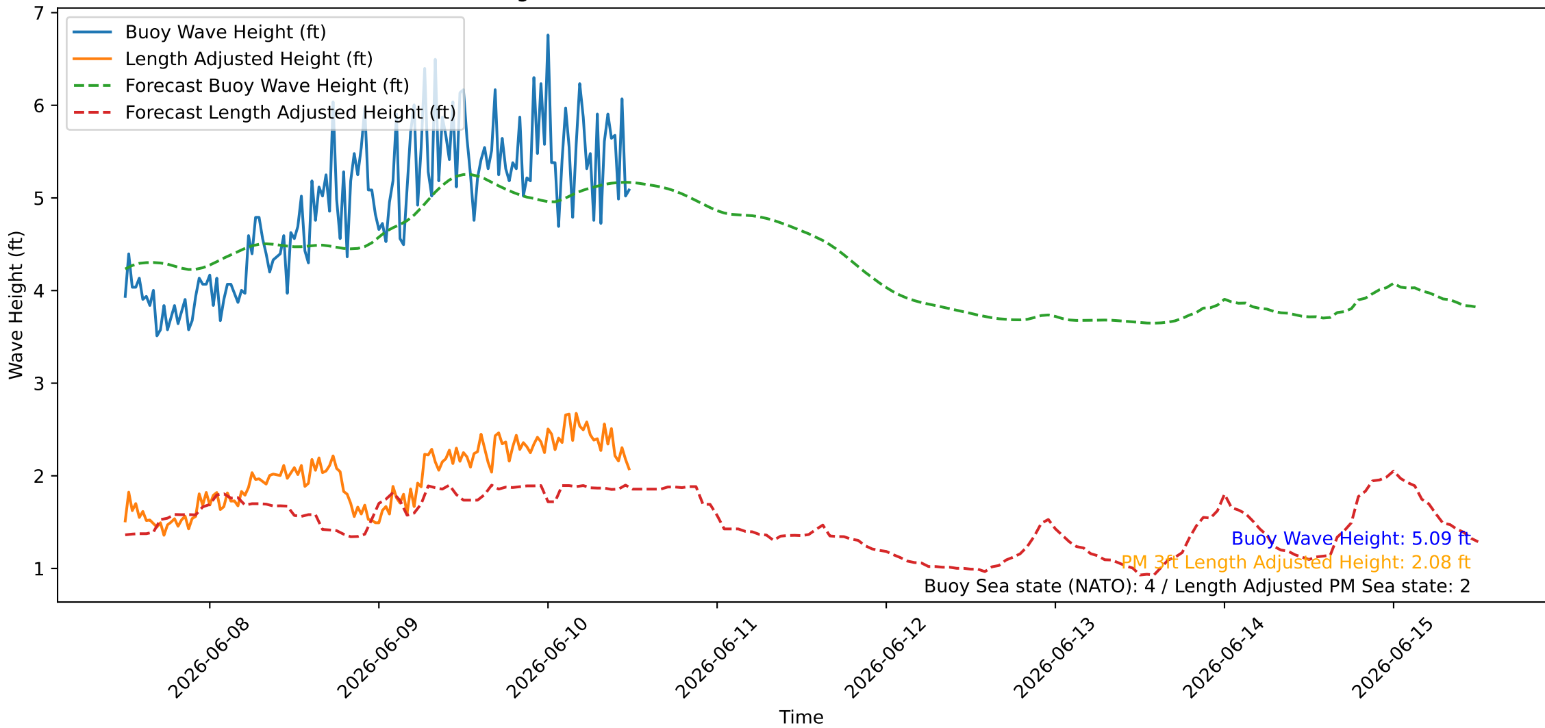
Wave Heights over Time for Oceanside Harbor at 2026-06-10 12:00:26
