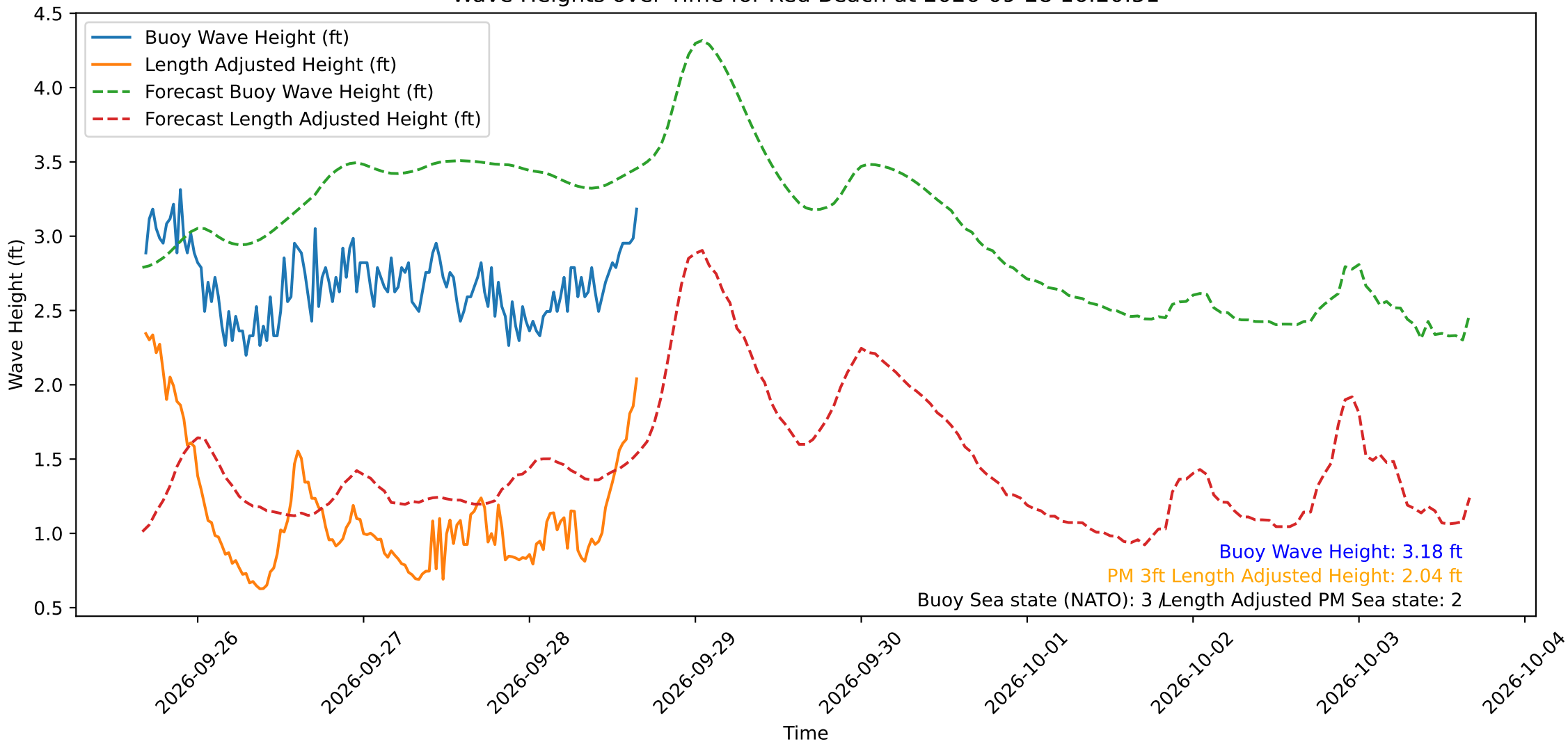
Wave Heights over Time for Red Beach at 2026-09-28 16:20:51
