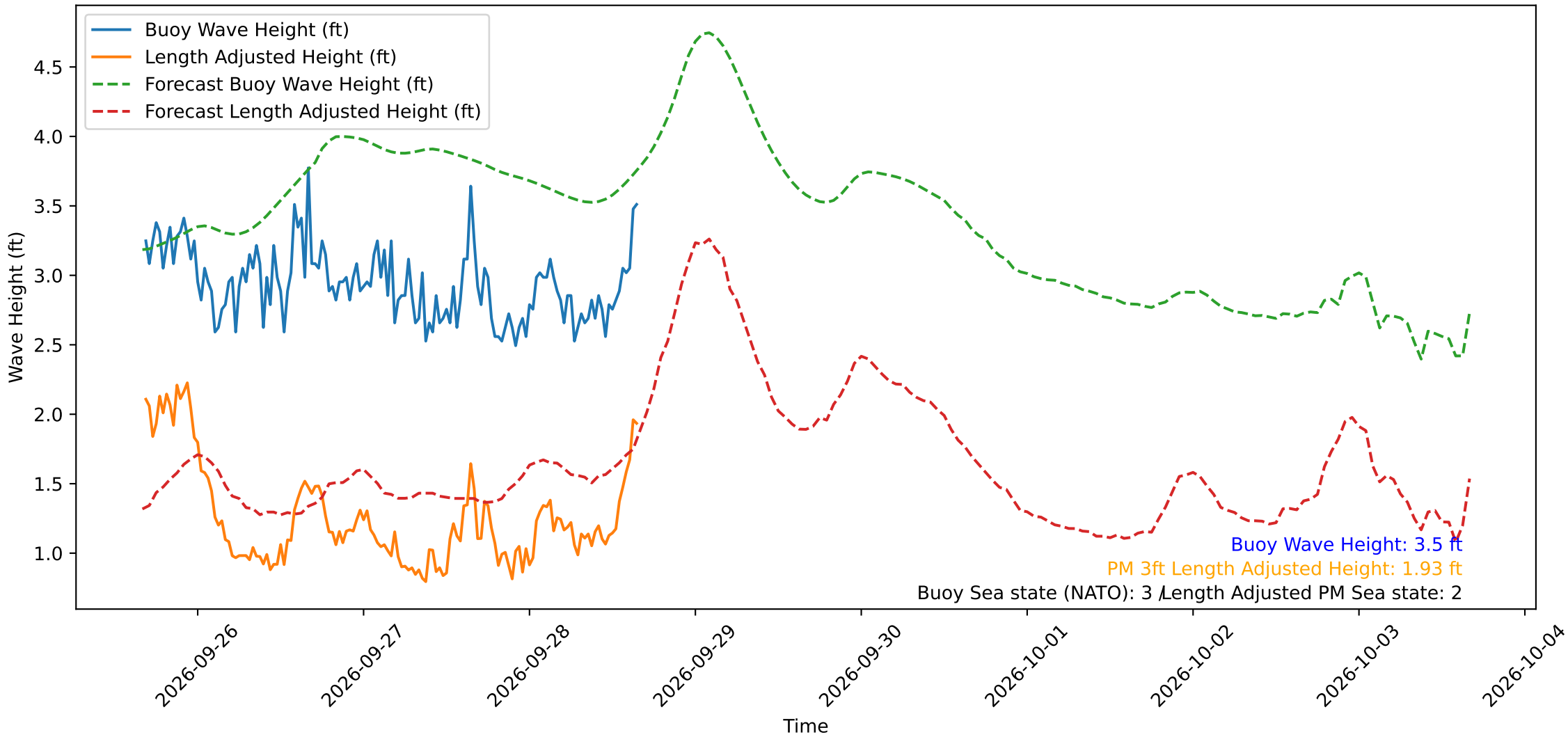
Wave Heights over Time for Oceanside Harbor at 2026-09-28 16:20:30
