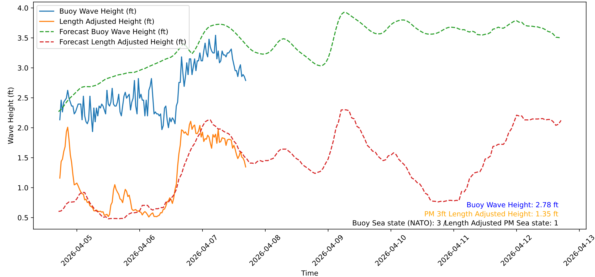
Wave Heights over Time for Red Beach at 2026-04-07 17:10:48
