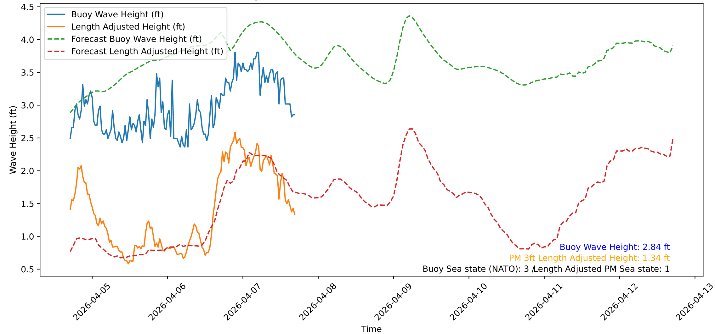
Wave Heights over Time for Green Beach at 2026-04-07 17:11:11
