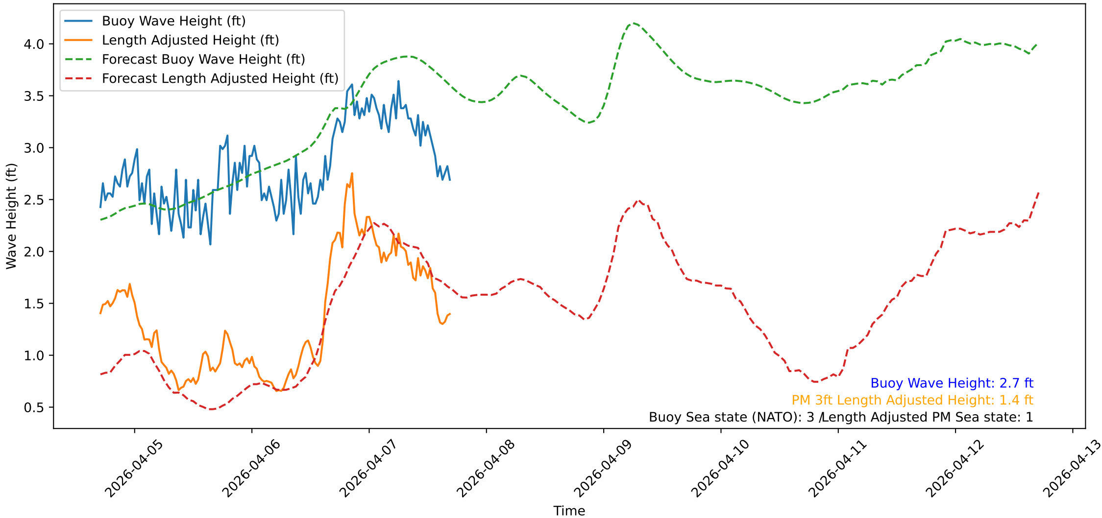
Wave Heights over Time for Oceanside Harbor at 2026-04-07 17:10:31
