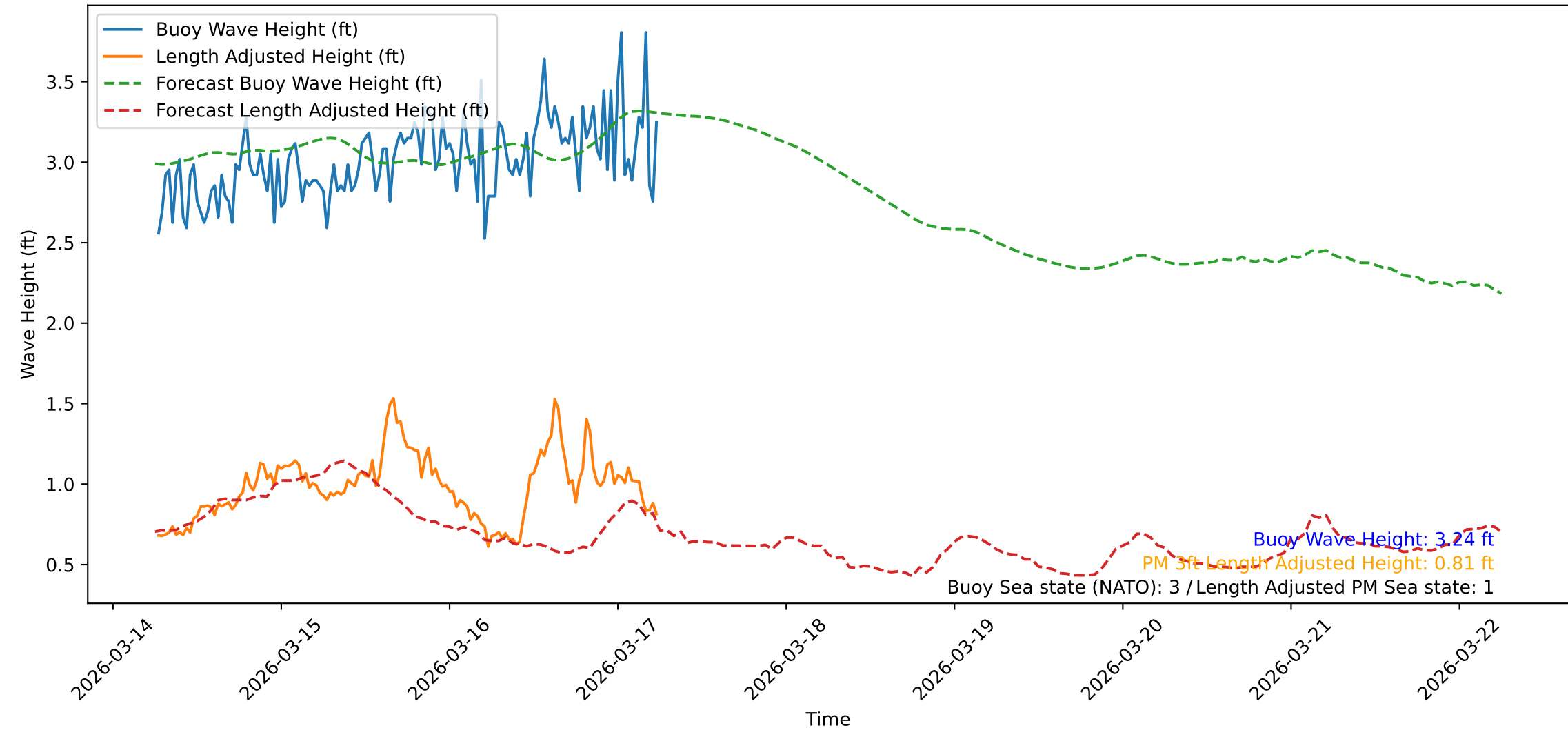
Wave Heights over Time for Red Beach at 2026-03-17 06:21:09
