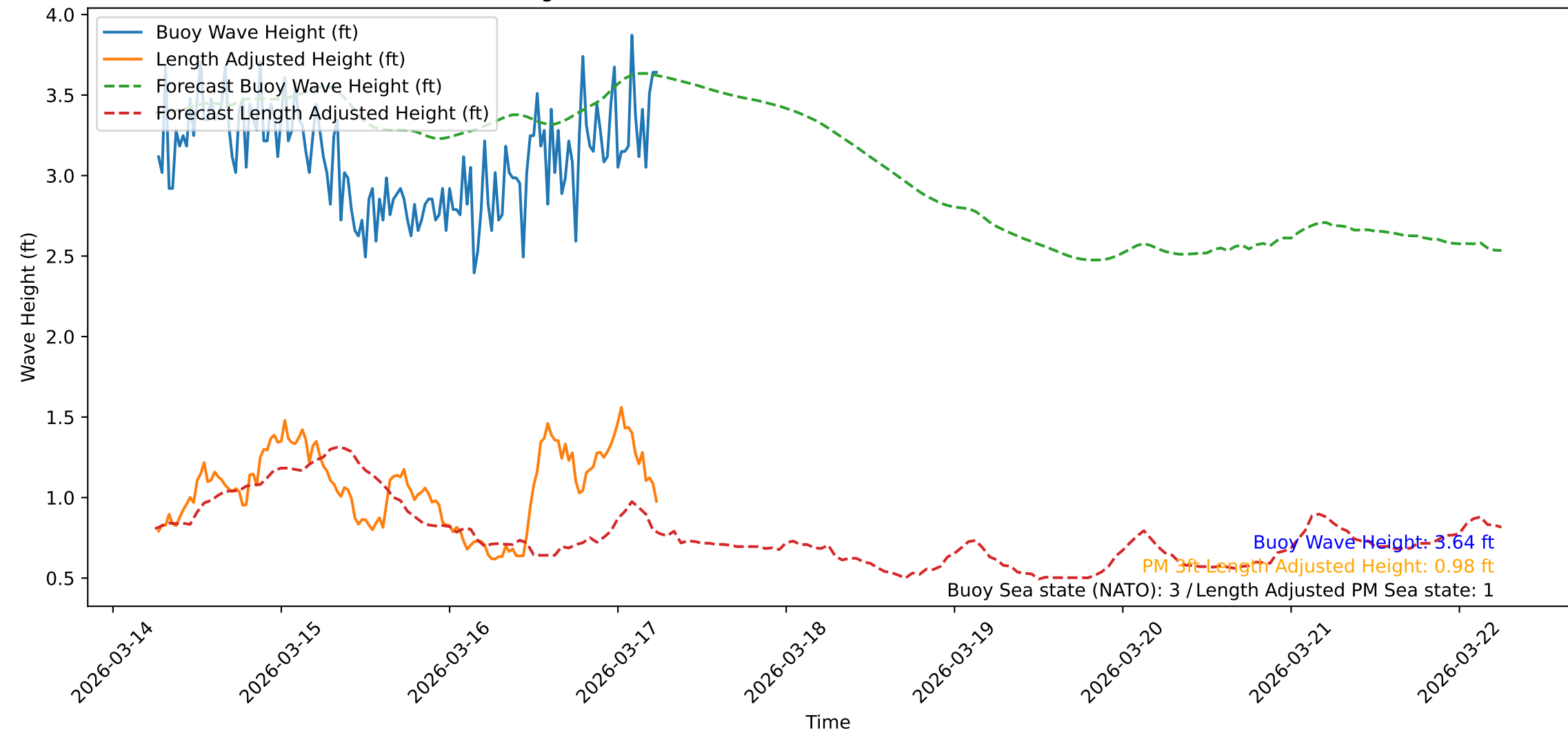
Wave Heights over Time for Oceanside Harbor at 2026-03-17 06:20:46
