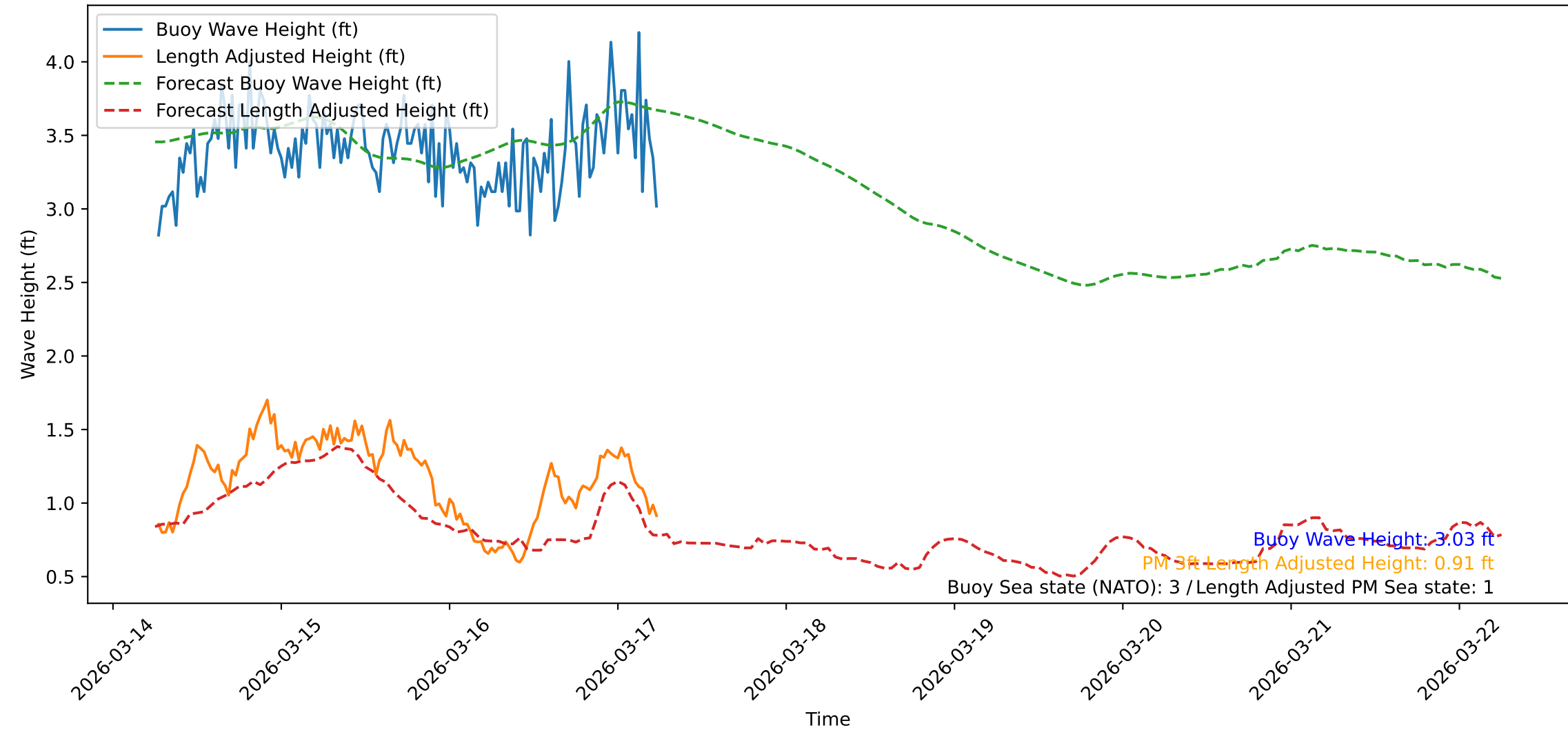
Wave Heights over Time for Green Beach at 2026-03-17 06:21:48
