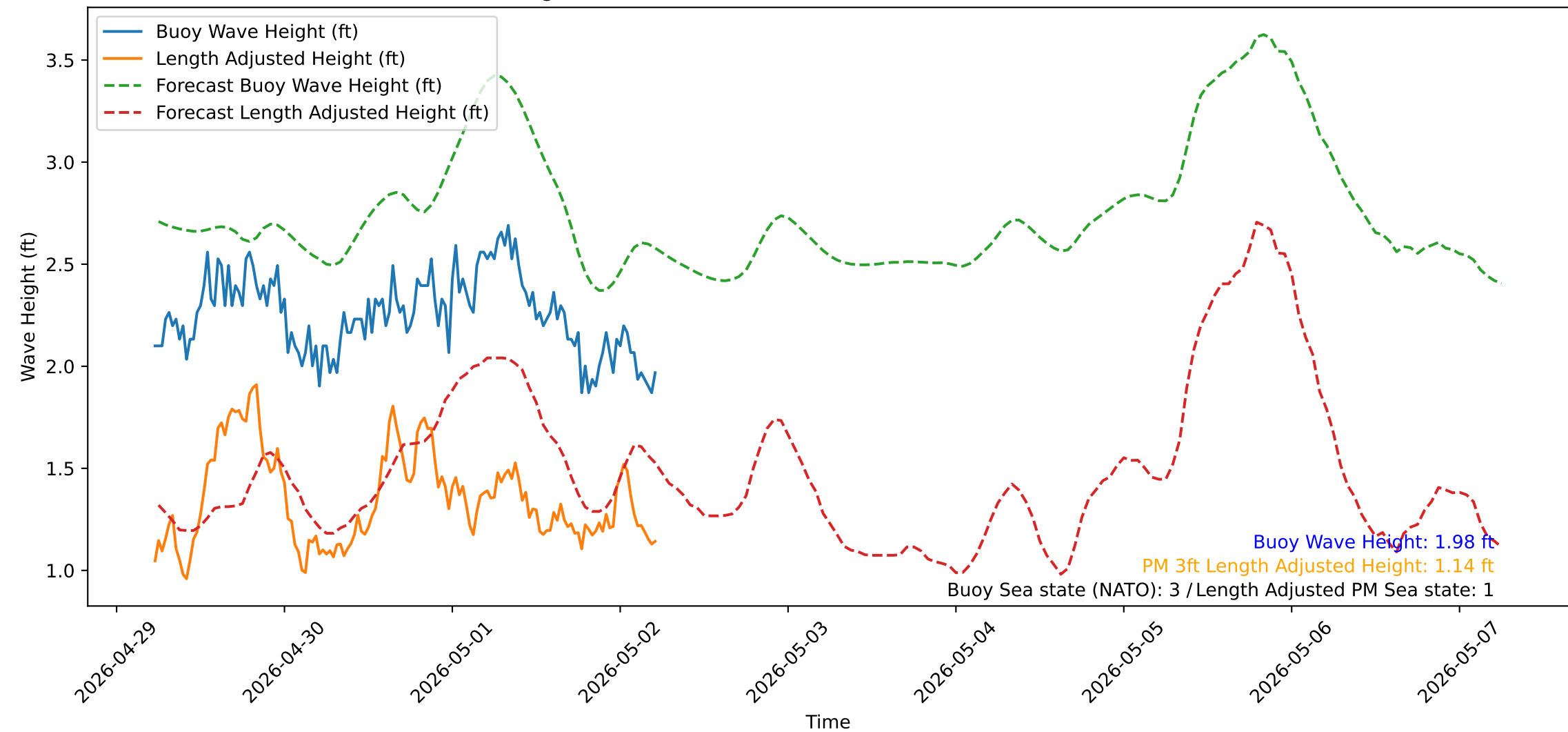
Wave Heights over Time for Oceanside Harbor at 2026-05-02 05:30:32
