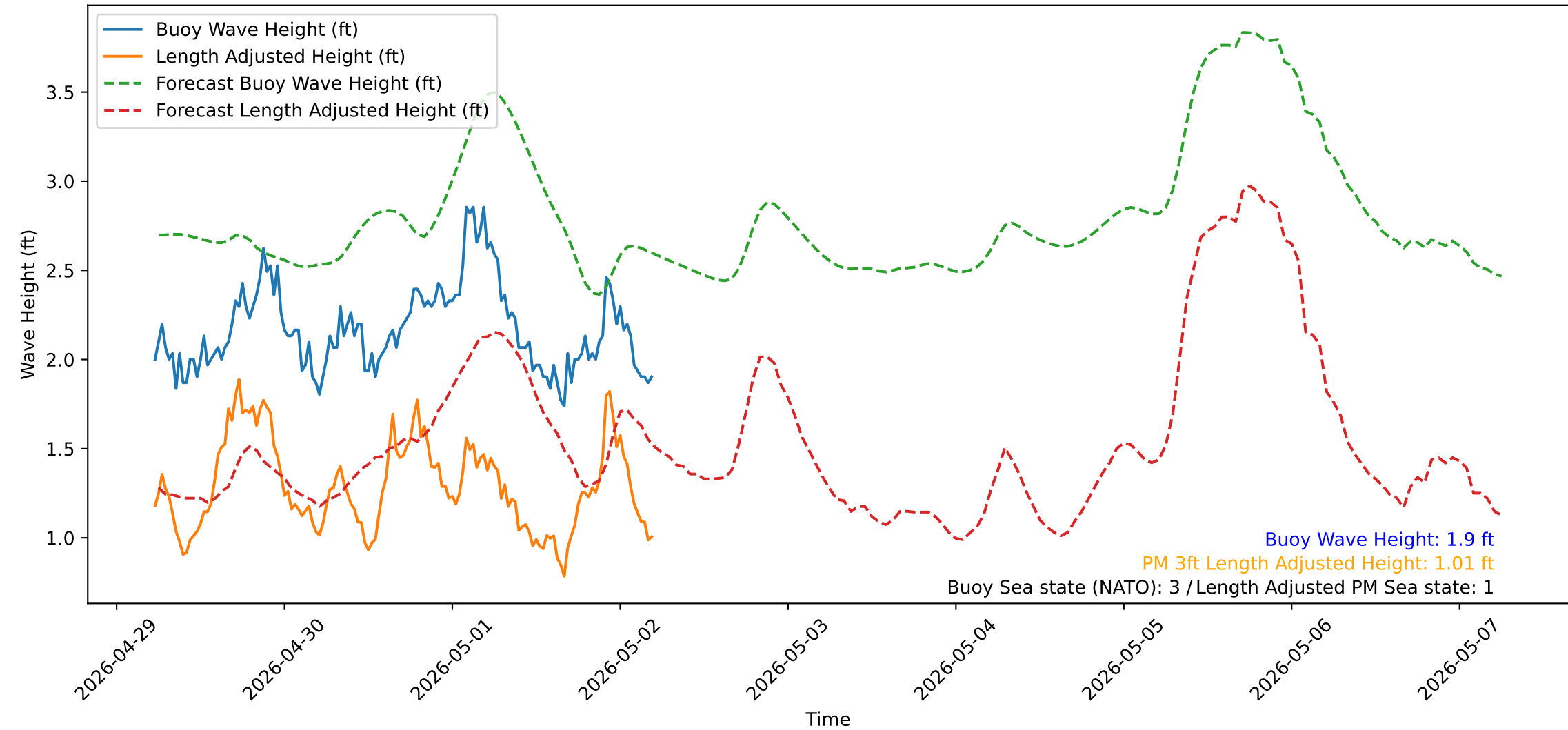
Wave Heights over Time for Green Beach at 2026-05-02 05:31:14
