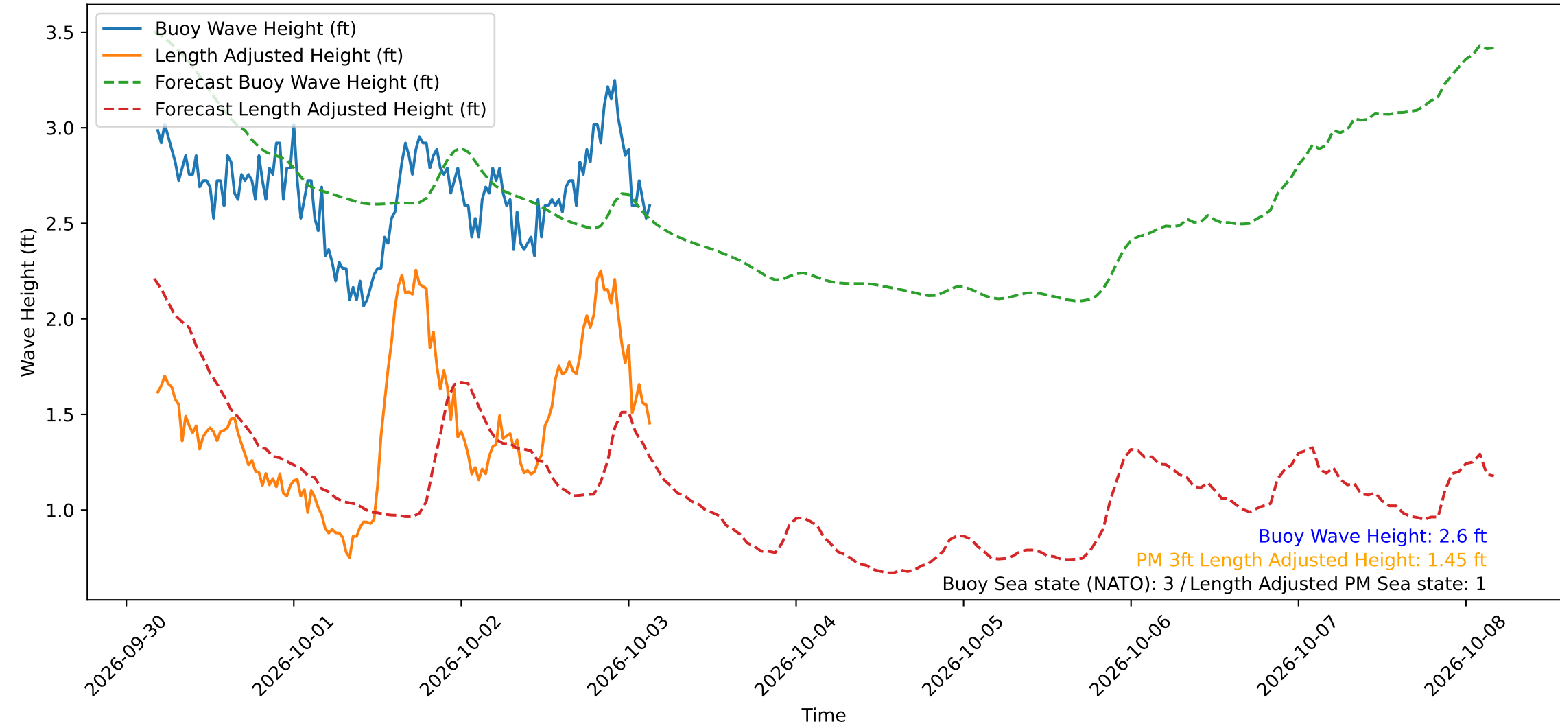
Wave Heights over Time for Red Beach at 2026-10-03 04:00:51
