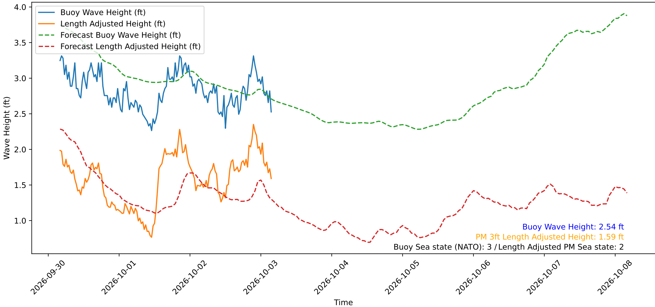
Wave Heights over Time for Oceanside Harbor at 2026-10-03 04:00:31
