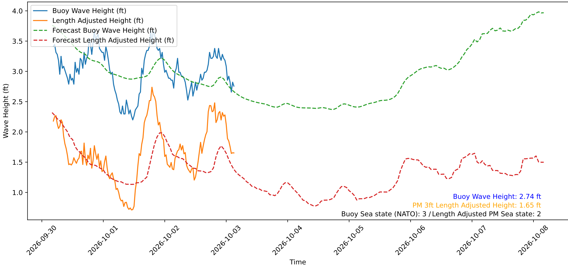
Wave Heights over Time for Green Beach at 2026-10-03 04:01:13
