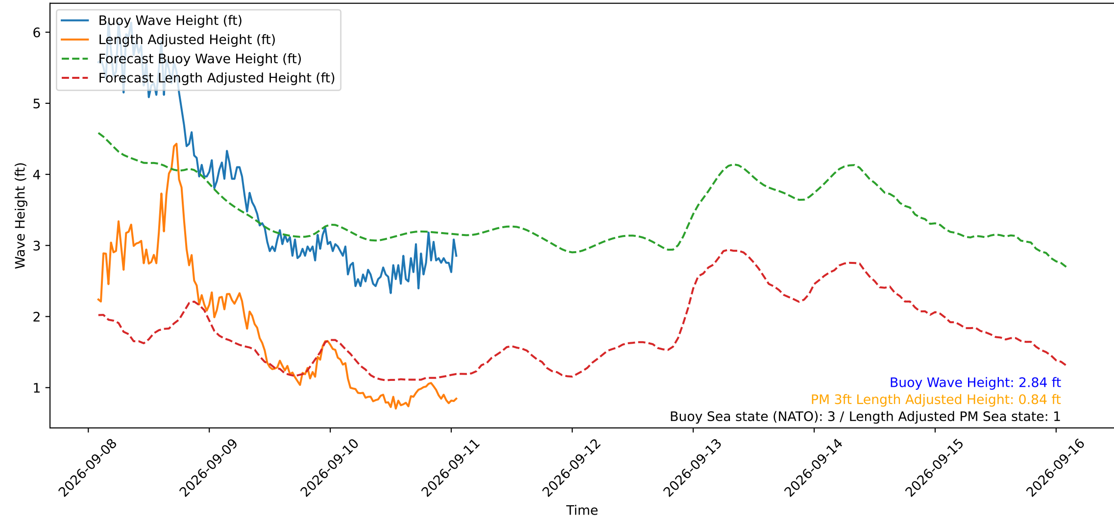
Wave Heights over Time for Red Beach at 2026-09-11 01:40:49
