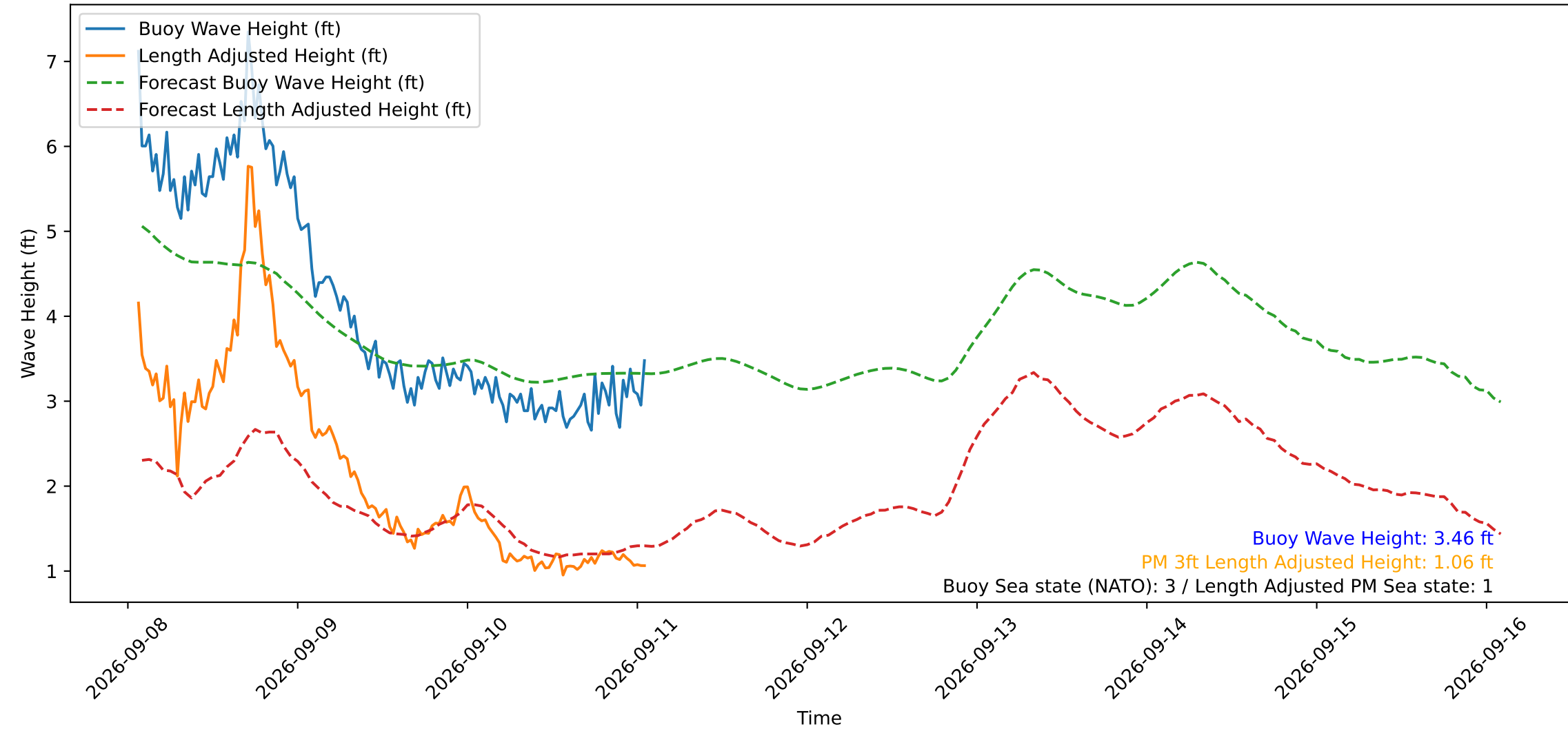
Wave Heights over Time for Oceanside Harbor at 2026-09-11 01:40:29
