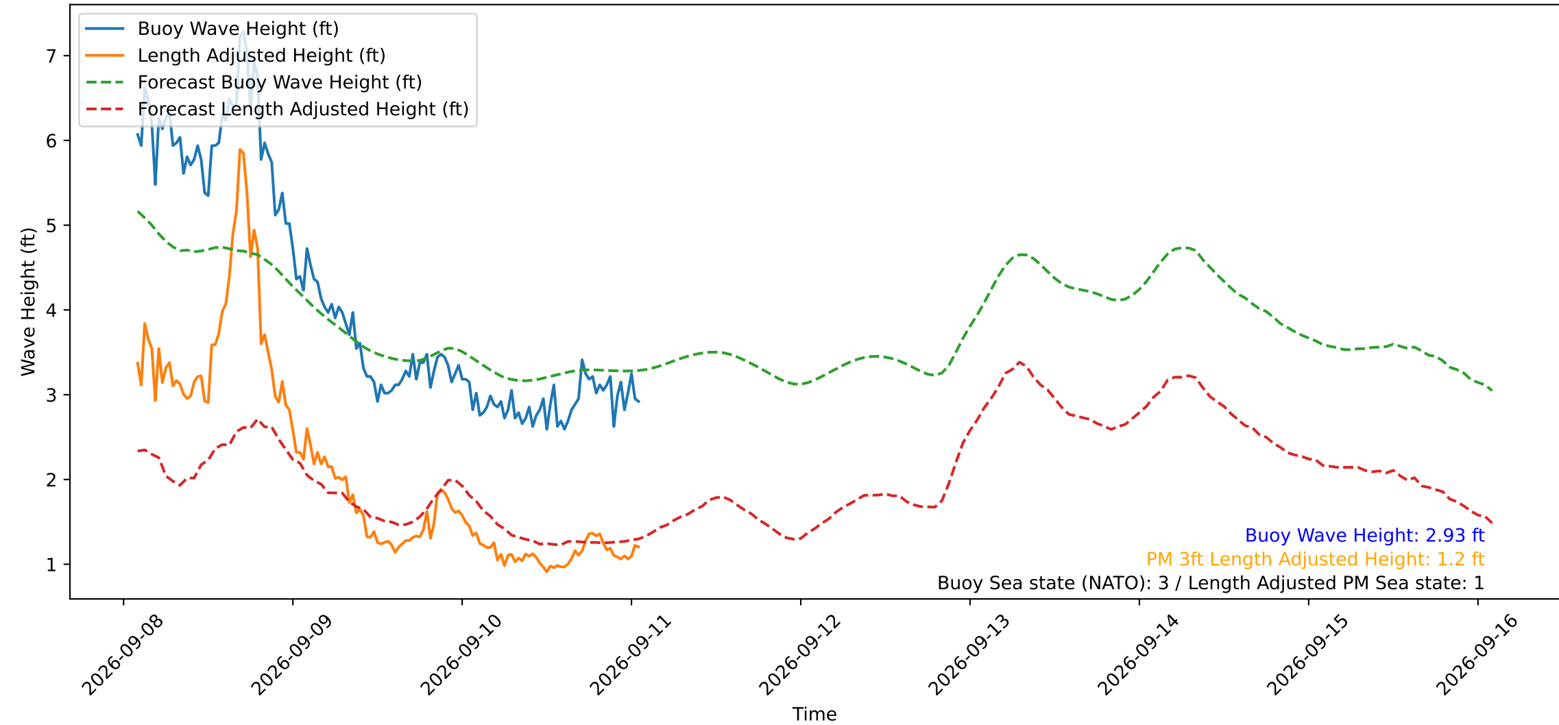
Wave Heights over Time for Green Beach at 2026-09-11 01:41:11
