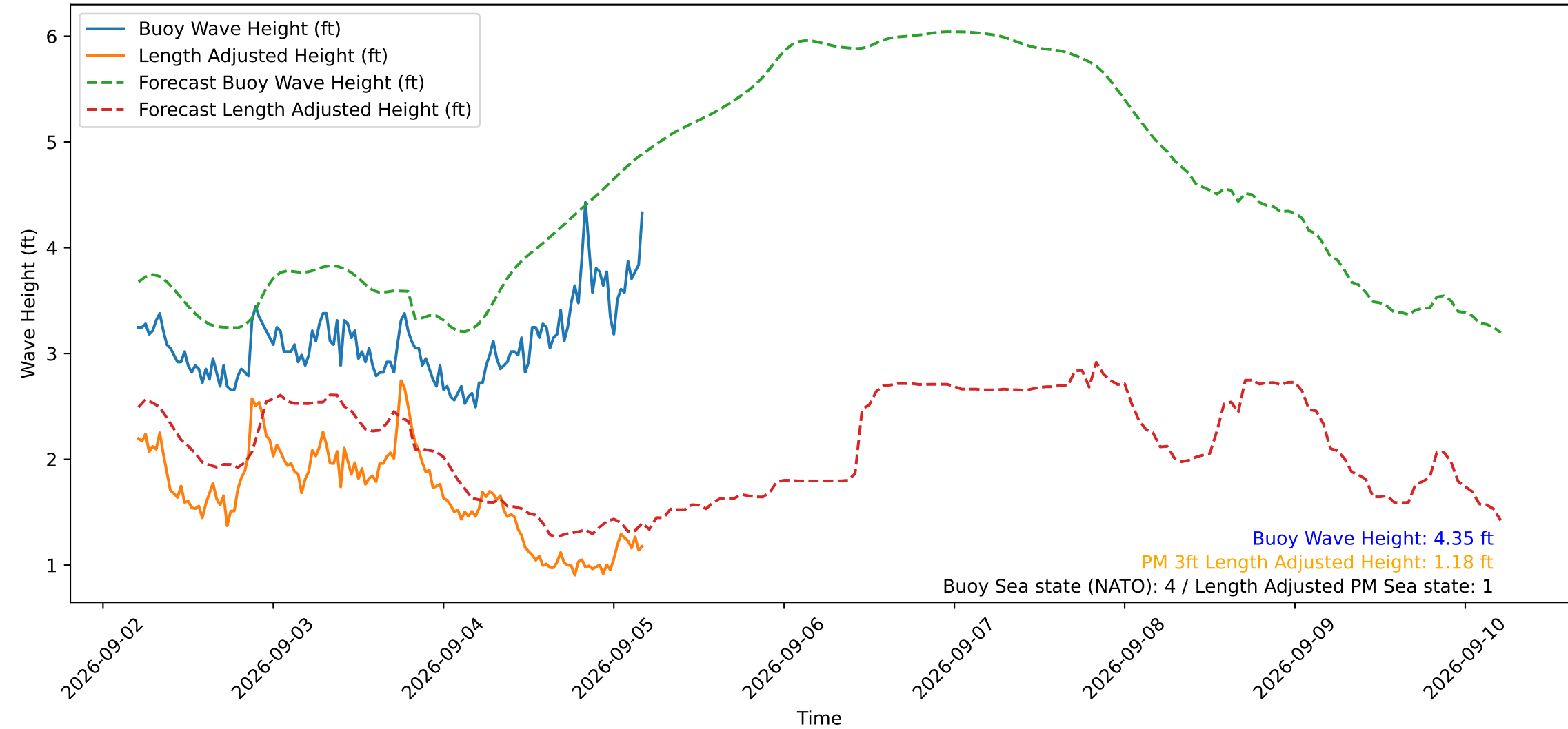
Wave Heights over Time for Green Beach at 2026-09-05 04:41:12
