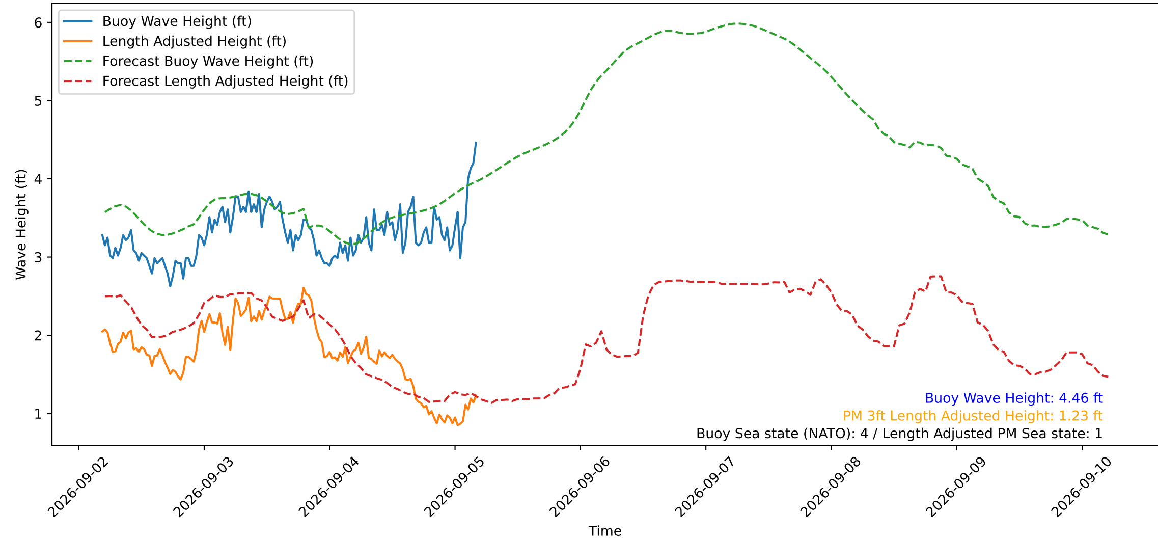
Wave Heights over Time for Oceanside Harbor at 2026-09-05 04:40:30
