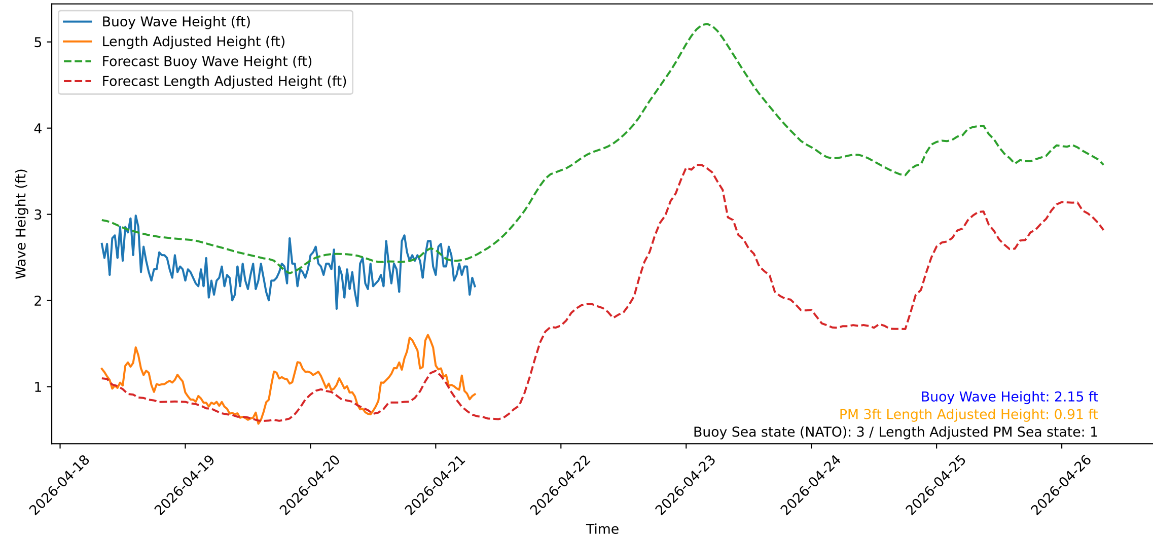
Wave Heights over Time for Oceanside Harbor at 2026-04-21 08:10:31
