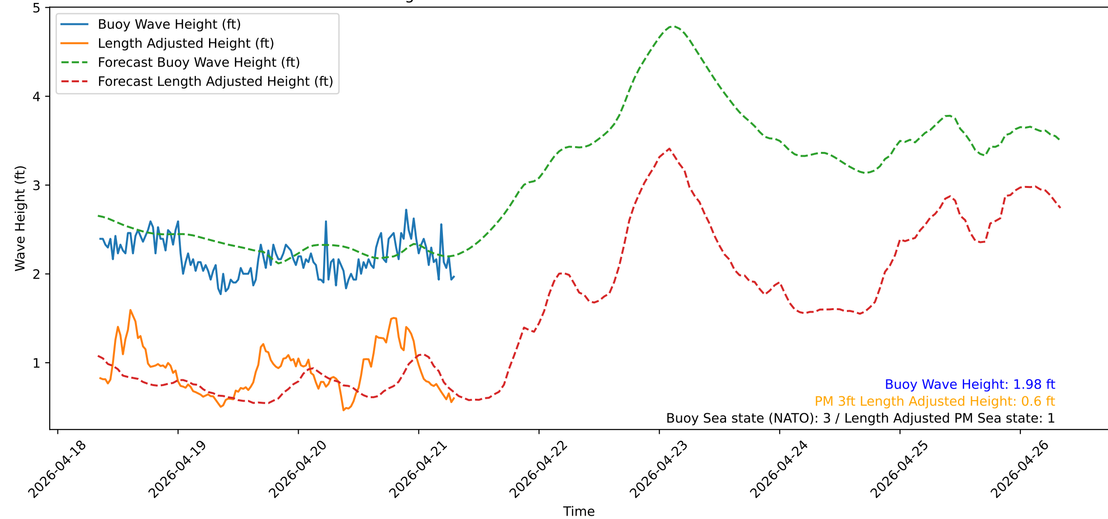
Wave Heights over Time for Red Beach at 2026-04-21 08:10:50
