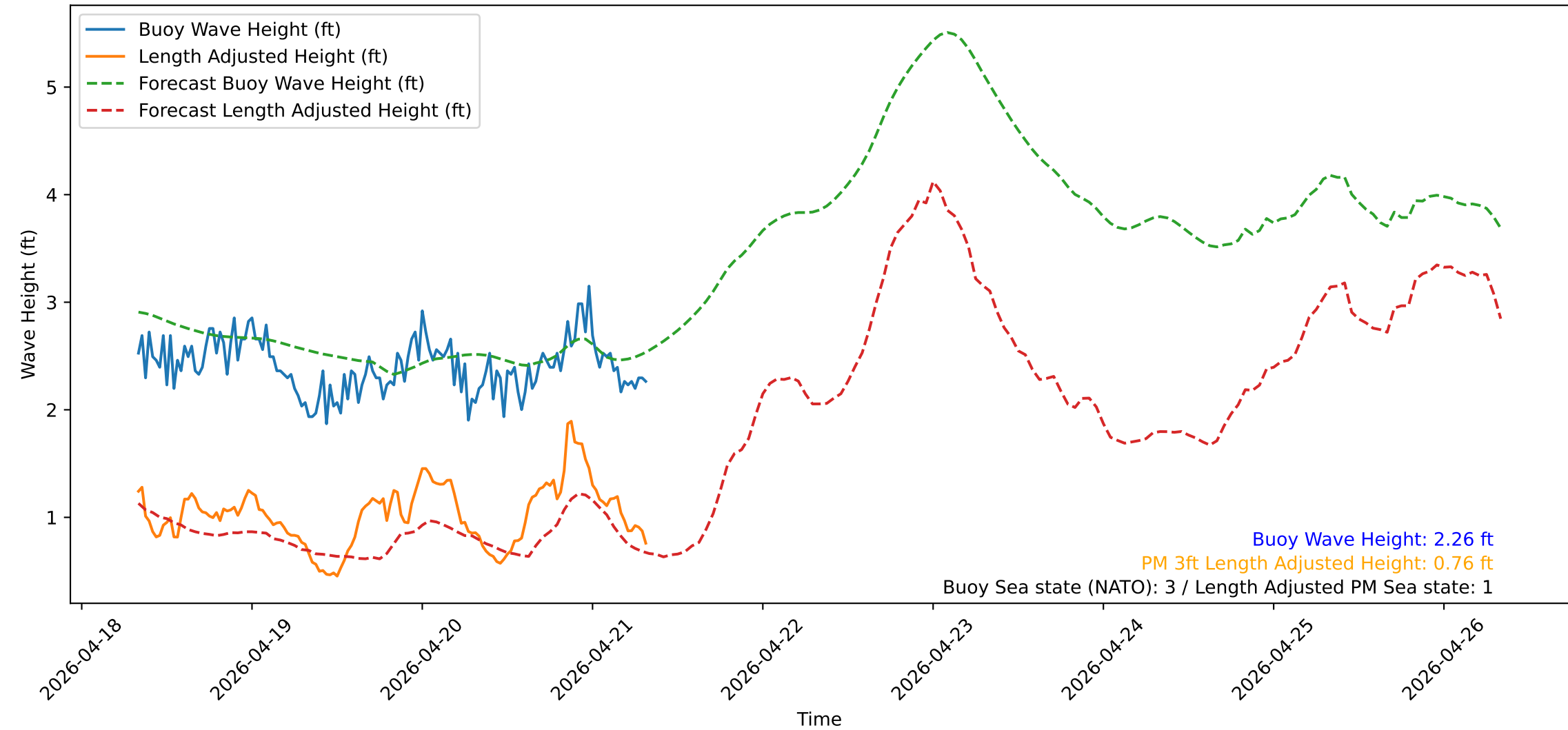
Wave Heights over Time for Green Beach at 2026-04-21 08:11:13
