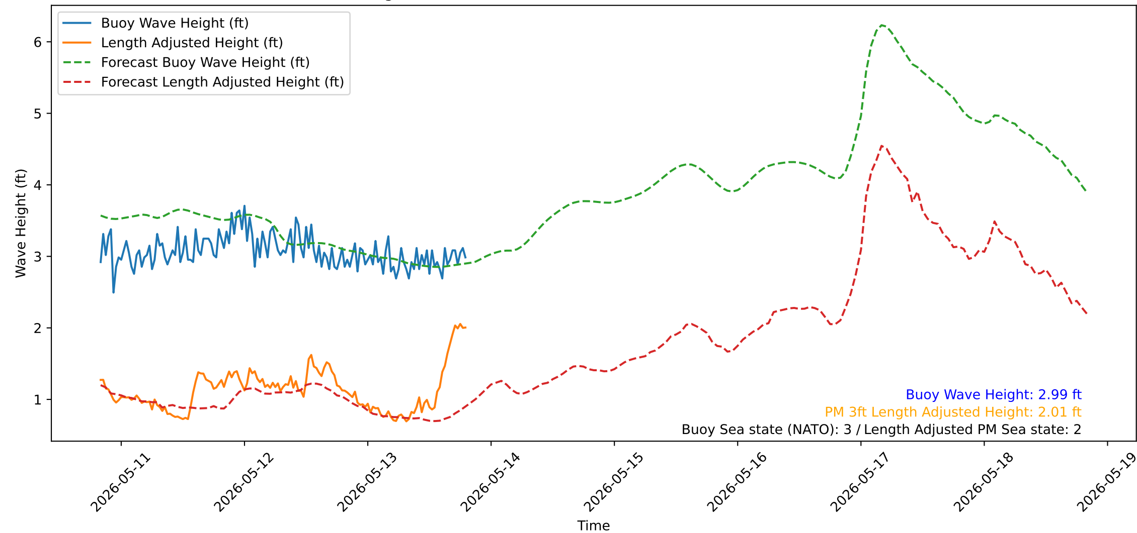
Wave Heights over Time for Oceanside Harbor at 2026-05-13 19:50:31
