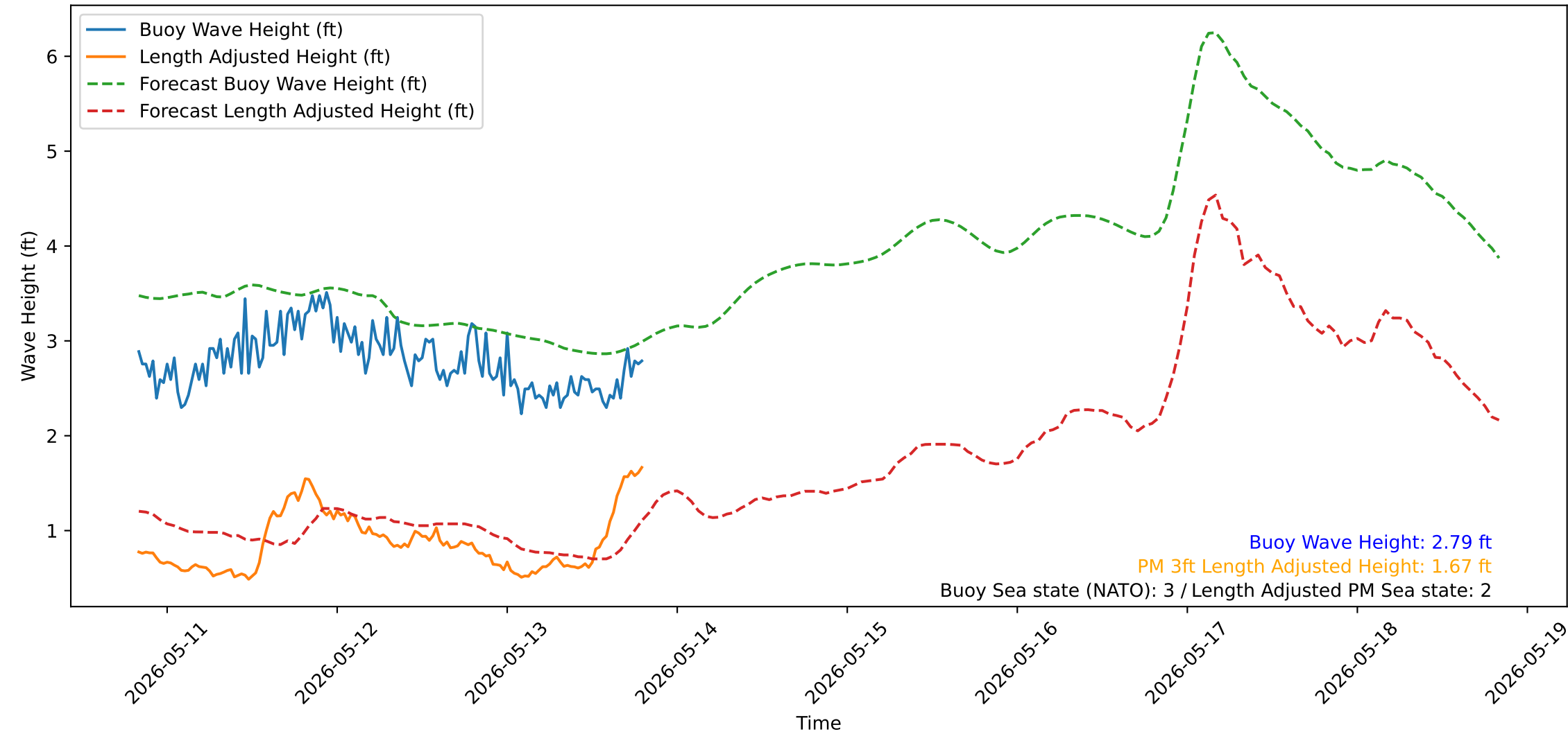
Wave Heights over Time for Green Beach at 2026-05-13 19:51:14
