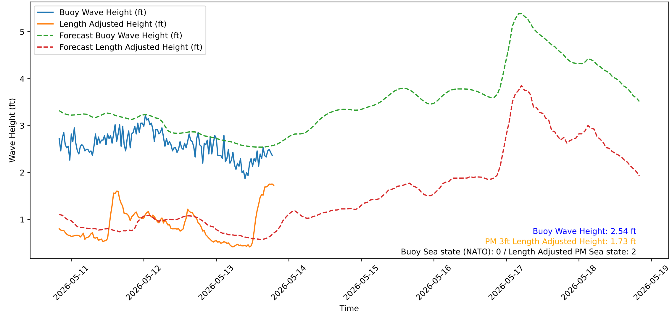
Wave Heights over Time for Red Beach at 2026-05-13 19:50:51
