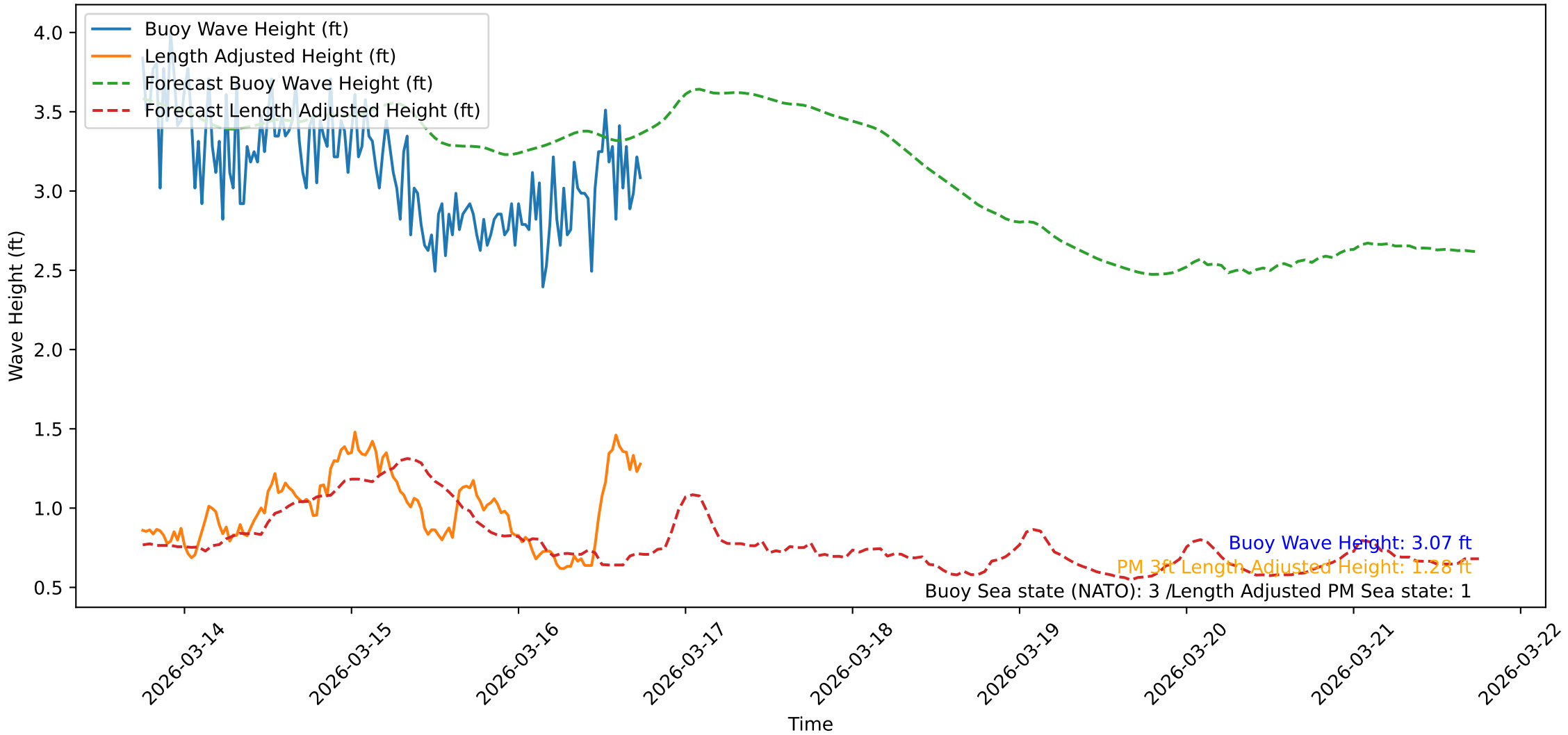
Wave Heights over Time for Oceanside Harbor at 2026-03-16 18:00:42
