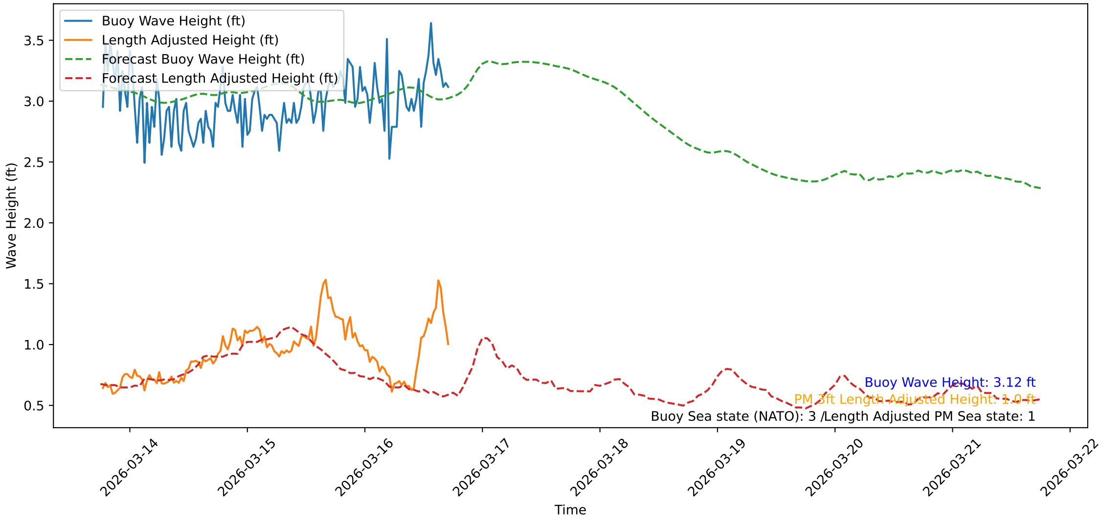
Wave Heights over Time for Red Beach at 2026-03-16 18:01:06
