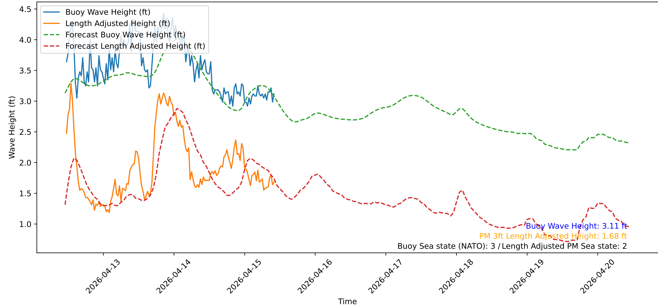
Wave Heights over Time for Red Beach at 2026-04-15 11:00:50
