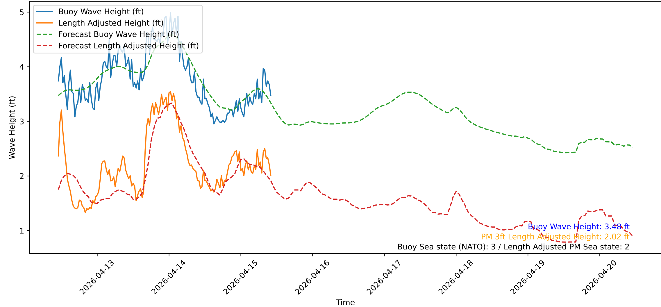
Wave Heights over Time for Green Beach at 2026-04-15 11:01:13
