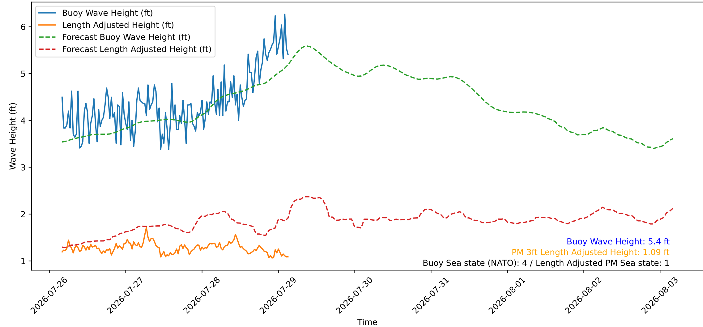
Wave Heights over Time for Green Beach at 2026-07-29 03:51:10
