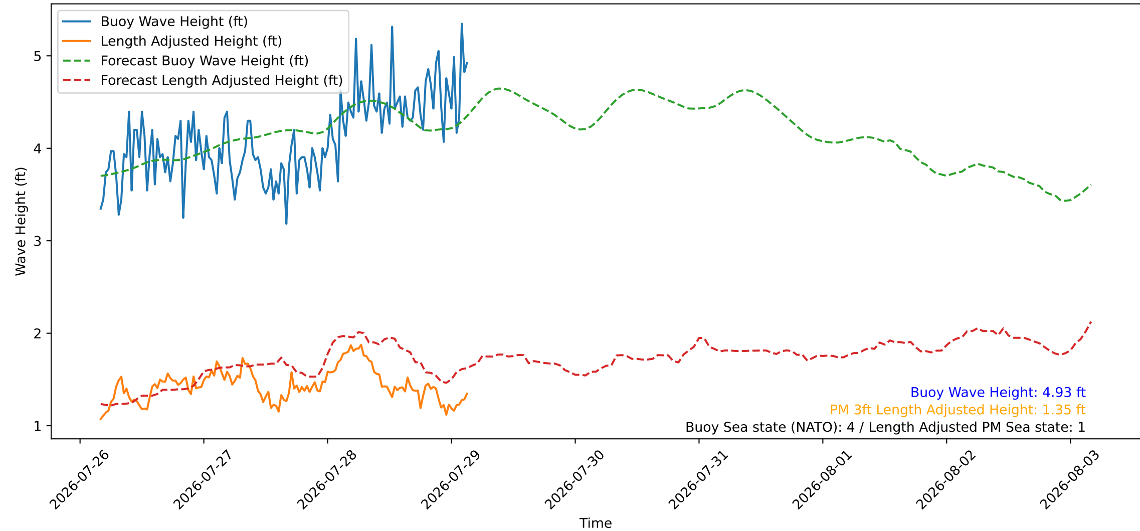
Wave Heights over Time for Oceanside Harbor at 2026-07-29 03:50:26
