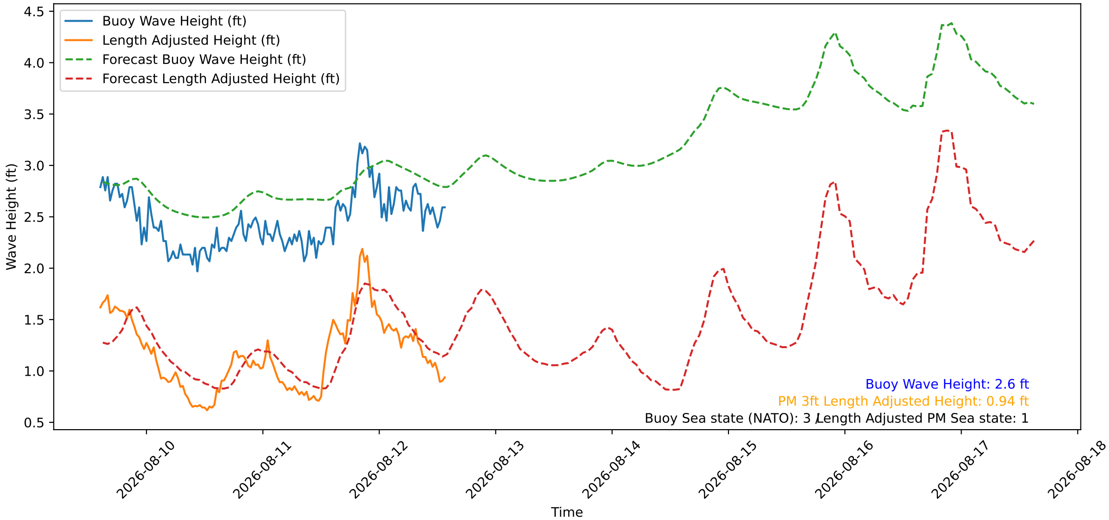
Wave Heights over Time for Green Beach at 2026-08-12 14:31:08
