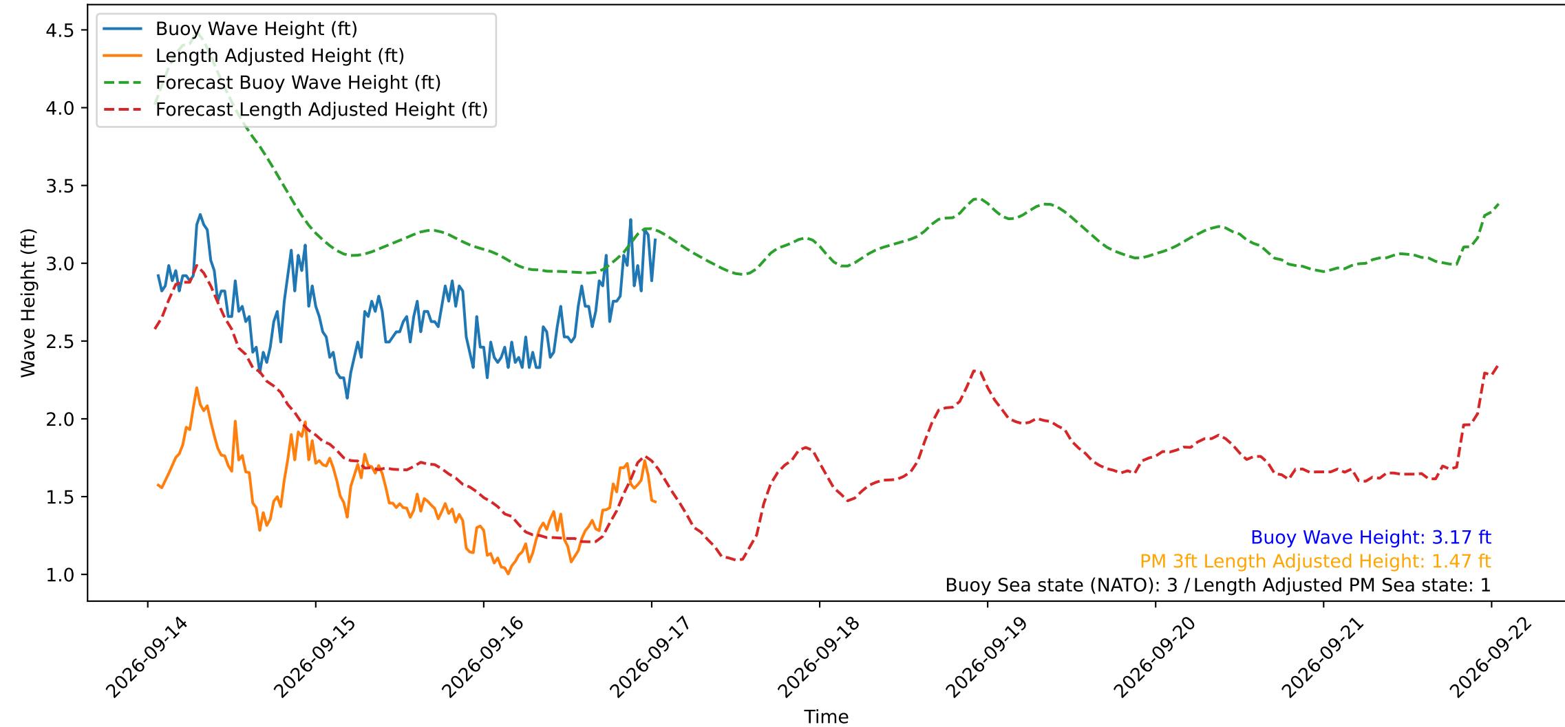
Wave Heights over Time for Green Beach at 2026-09-17 01:21:15
