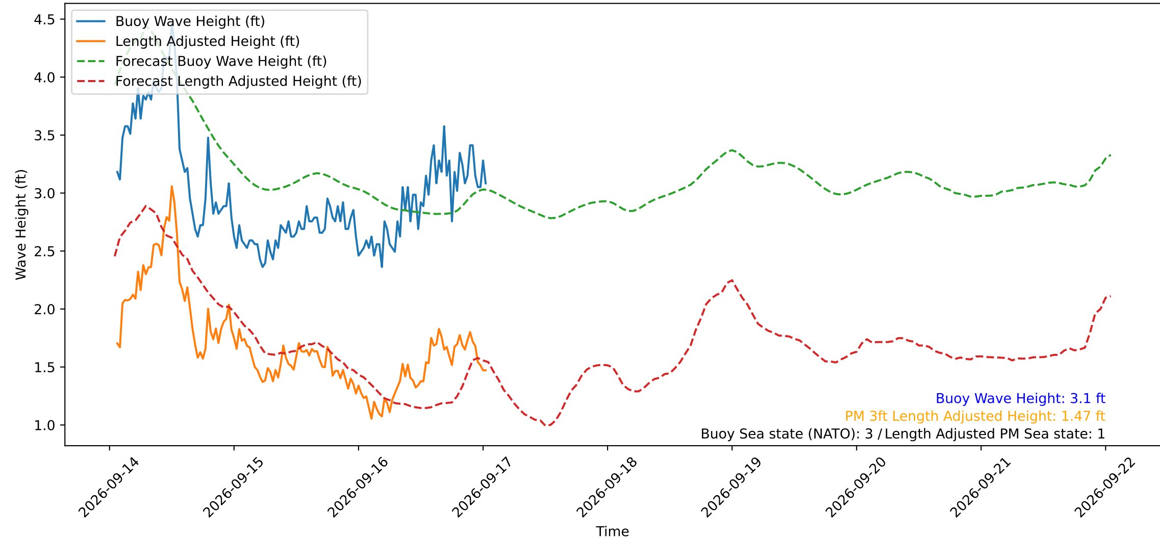
Wave Heights over Time for Oceanside Harbor at 2026-09-17 01:20:30
