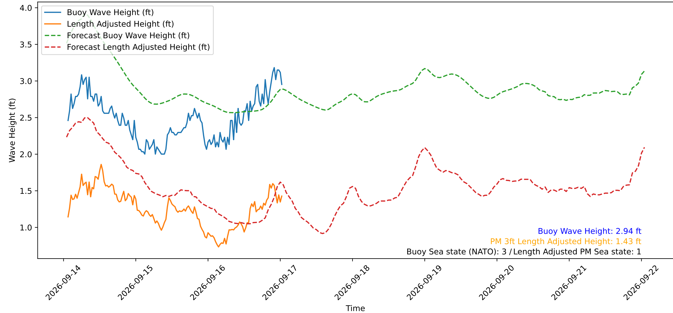
Wave Heights over Time for Red Beach at 2026-09-17 01:20:51
