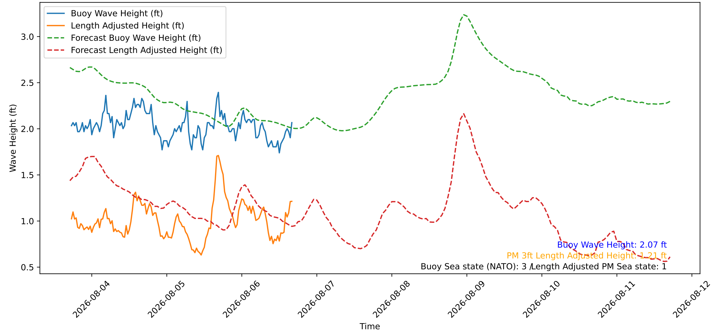
Wave Heights over Time for Red Beach at 2026-08-06 17:10:46
